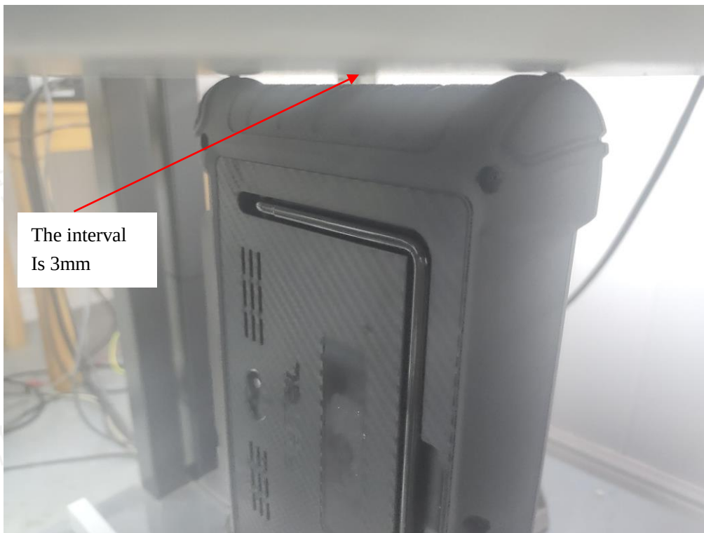
0mm body Vertical- Left Side Setup Photo
