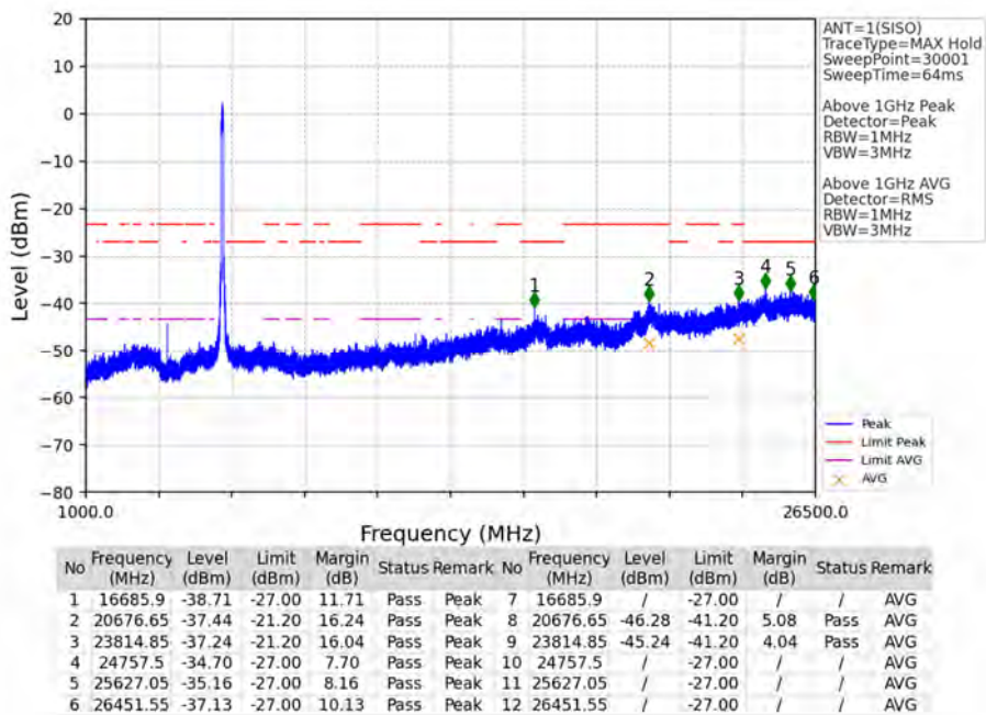
802.11ac(VHT80)_MCH_5775MHz_Ant1_NTNV
