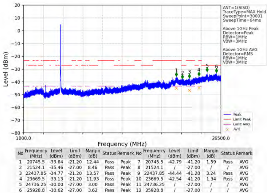
802.11ac(VHT40)_HCH_5795MHz_Ant1_NTNV
