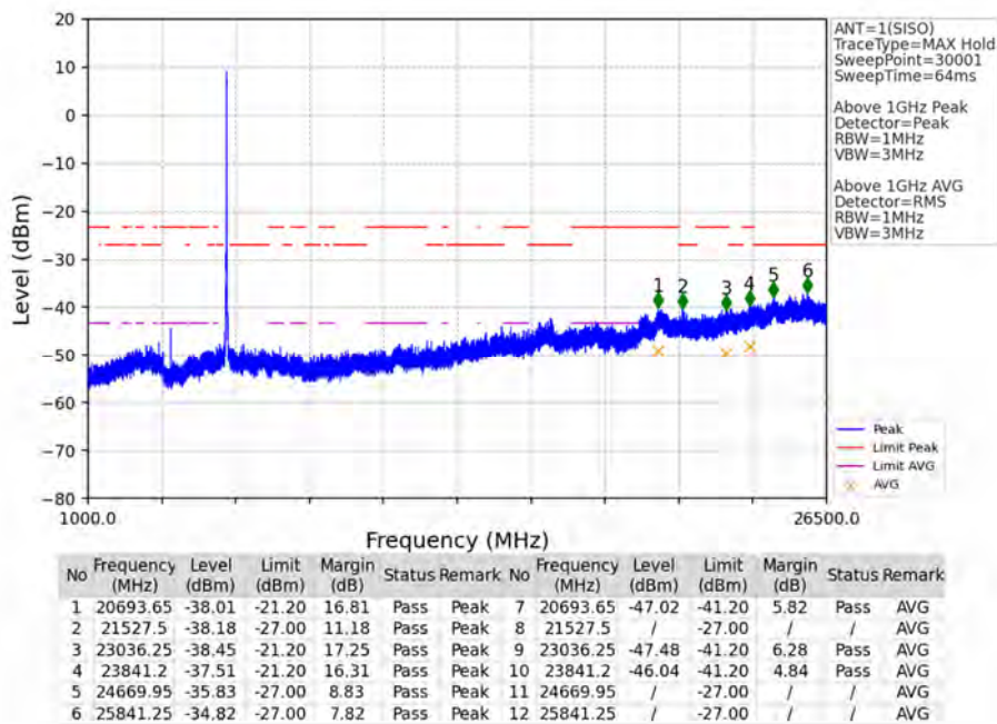
802.11ac(VHT20)_MCH_5785MHz_Ant1_NTNV
