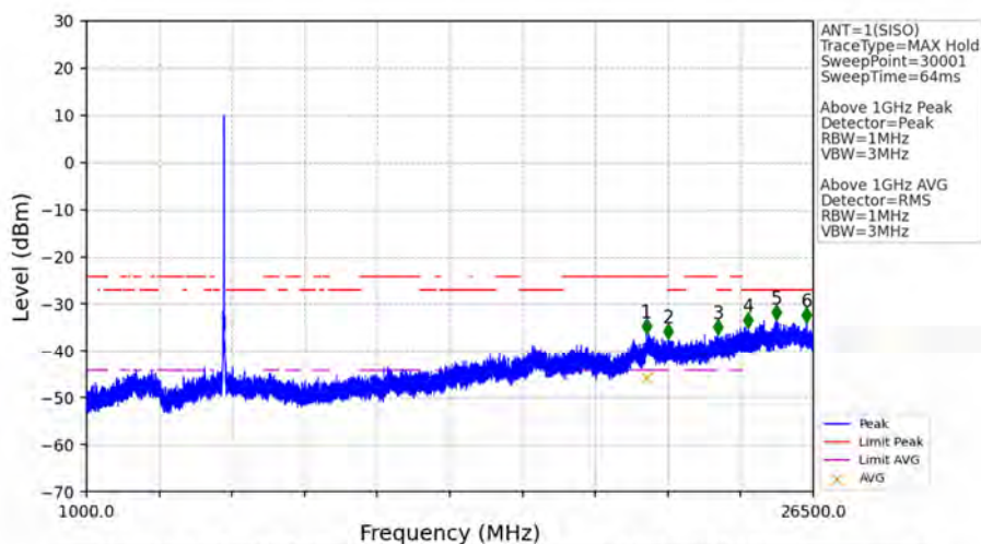
802.11a_HCH_5825MHz_Ant1_NTNV
