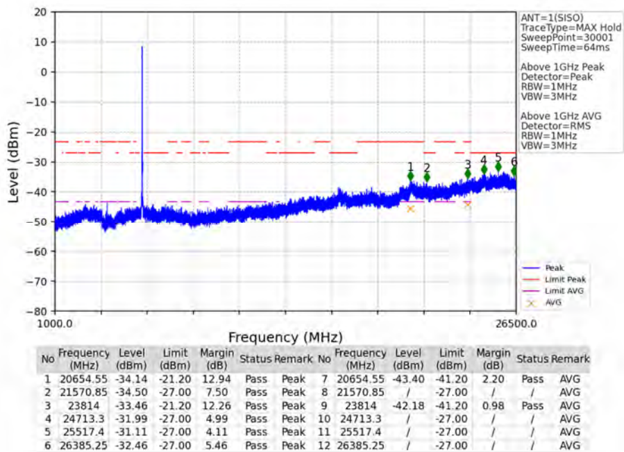
802.11ac(VHT20)_HCH_5825MHz_Ant1_NTNV
