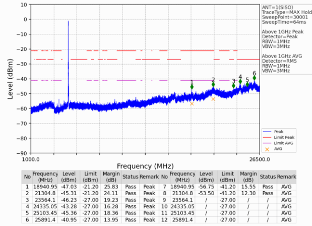
802.11a_LCH_5180MHz_Ant1_NTNV
