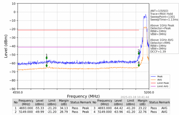
802.11a_LCH_5180MHz_Ant1_NTNV
