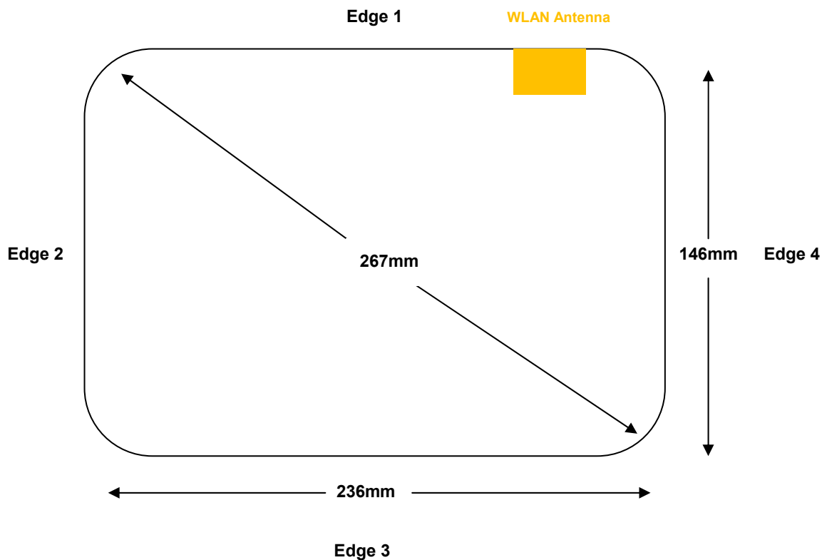
Front View
