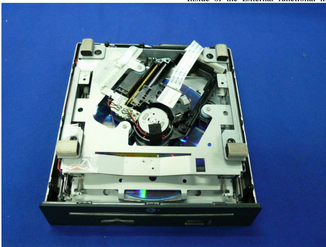
Figure 37 Inside of the External functional module
