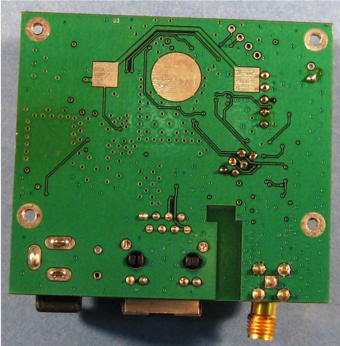
SHC-G – PCB Bottom
