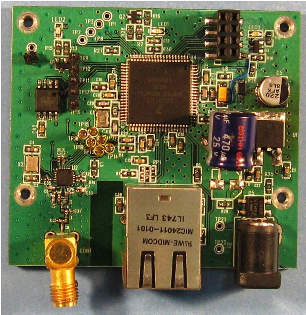
SHC-G – PCB Top
