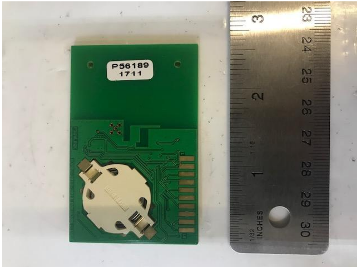
Figure 3. EUT (Back)
