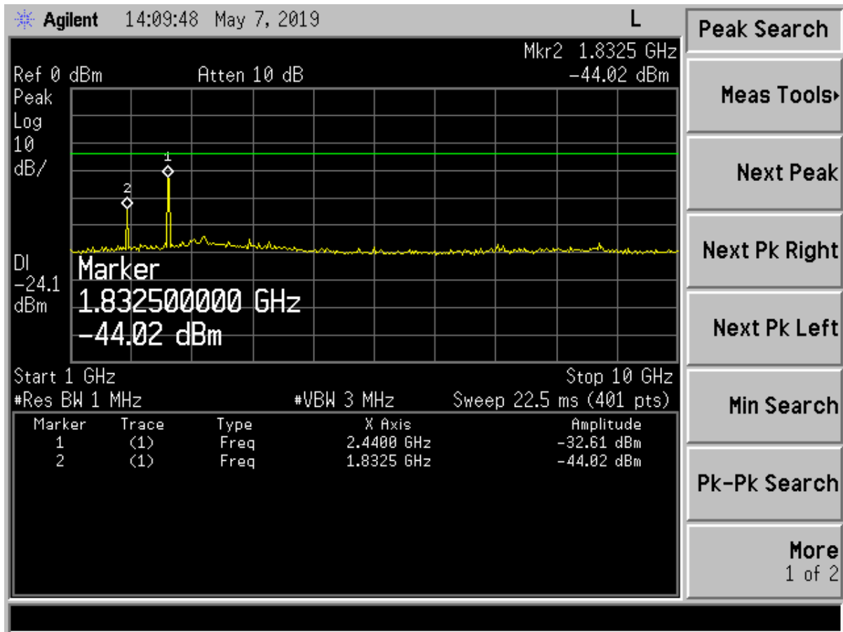
Figure 7. Conducted Spurious Emissions – Mid Channel, 1 GHz - 10 GHz
