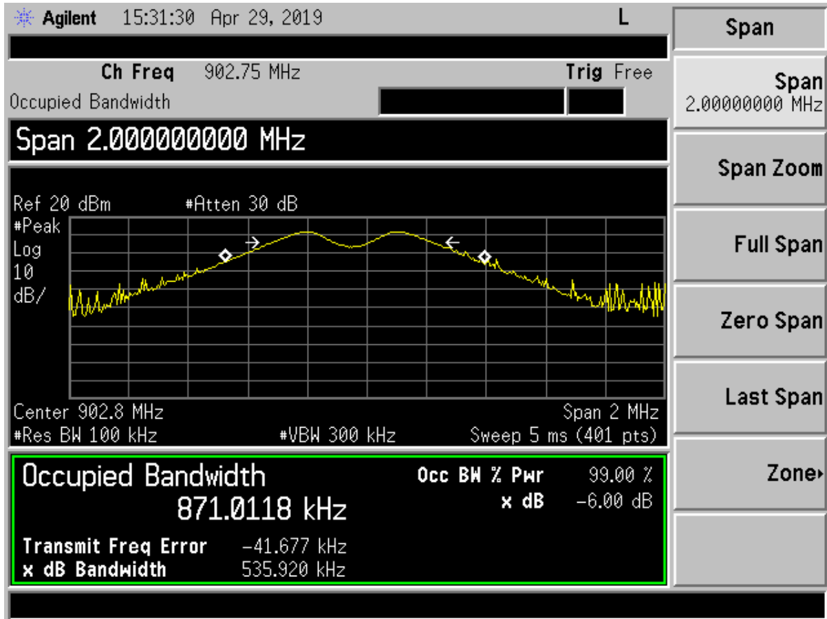
Figure 12. 6 dB Bandwidth Low Channel
