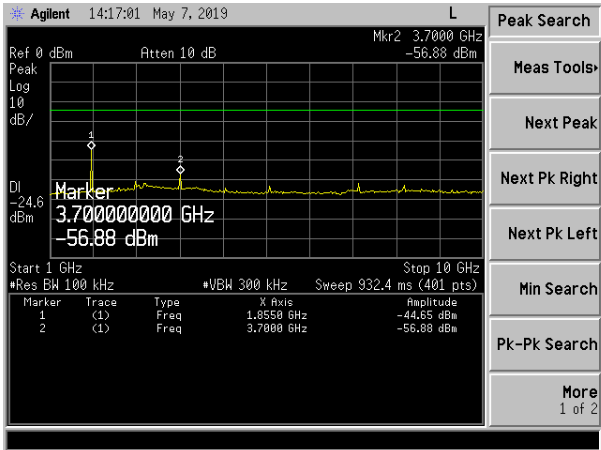
Figure 9. Conducted Spurious Emissions – High Channel, 1 GHz - 10 GHz
