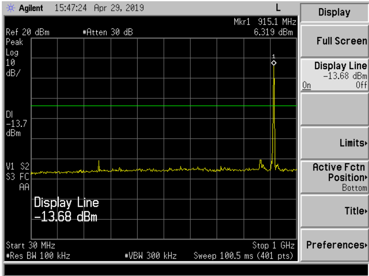
Figure 6. Conducted Spurious Emissions – Mid Channel, 30 MHz - 1 GHz
