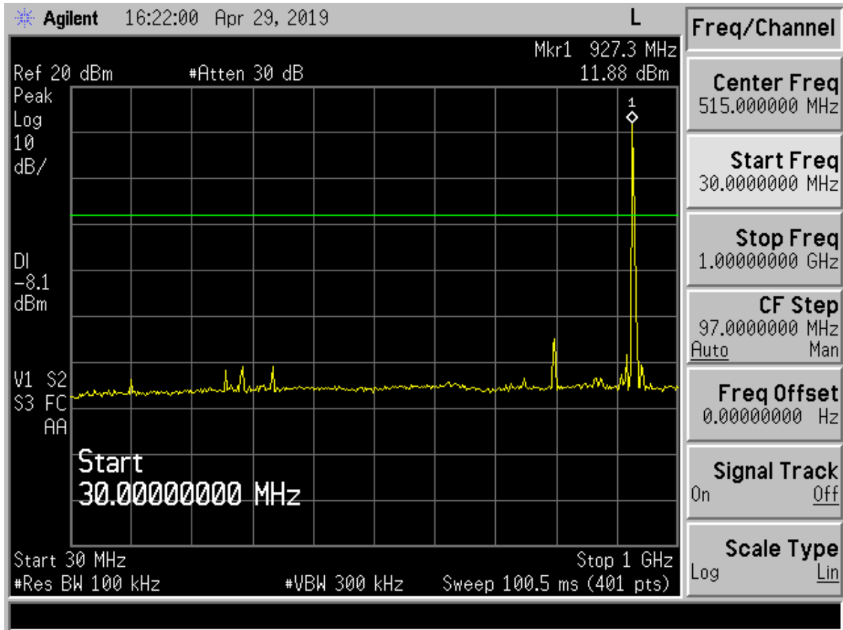
Figure 8. Conducted Spurious Emissions – High Channel, 30 MHz – 1 GHz
