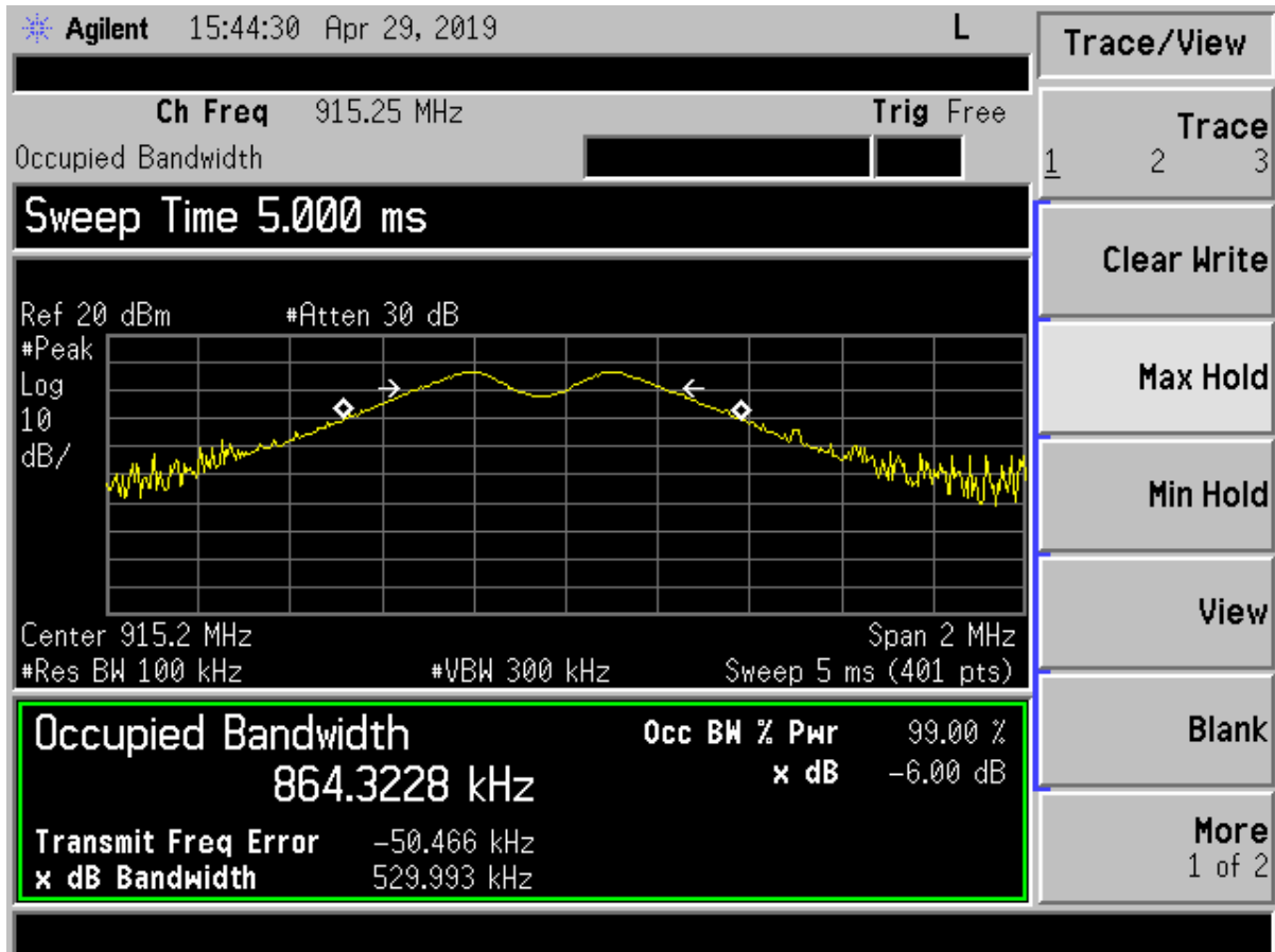
Figure 13. 6 dB Bandwidth Mid Channel
