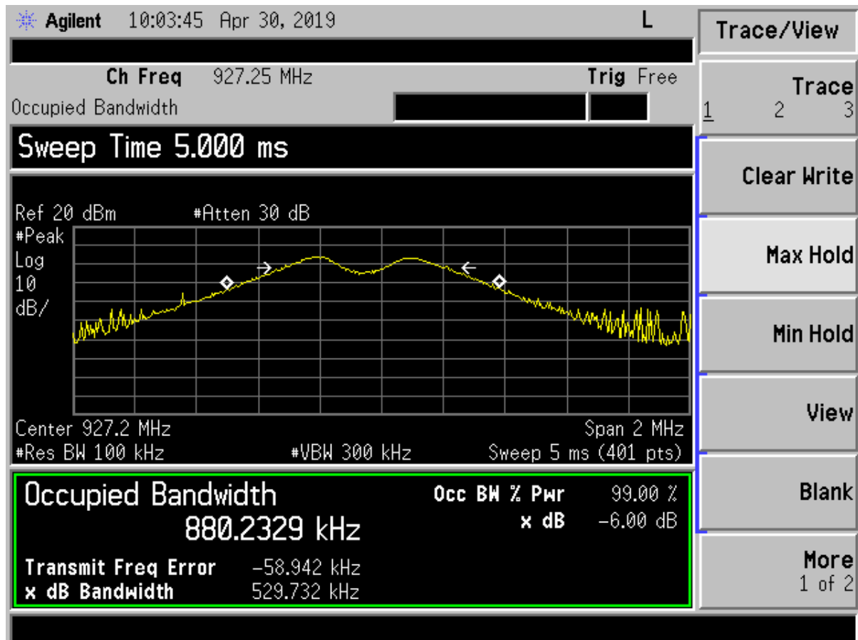
Figure 14. 6 dB Bandwidth High Channel
