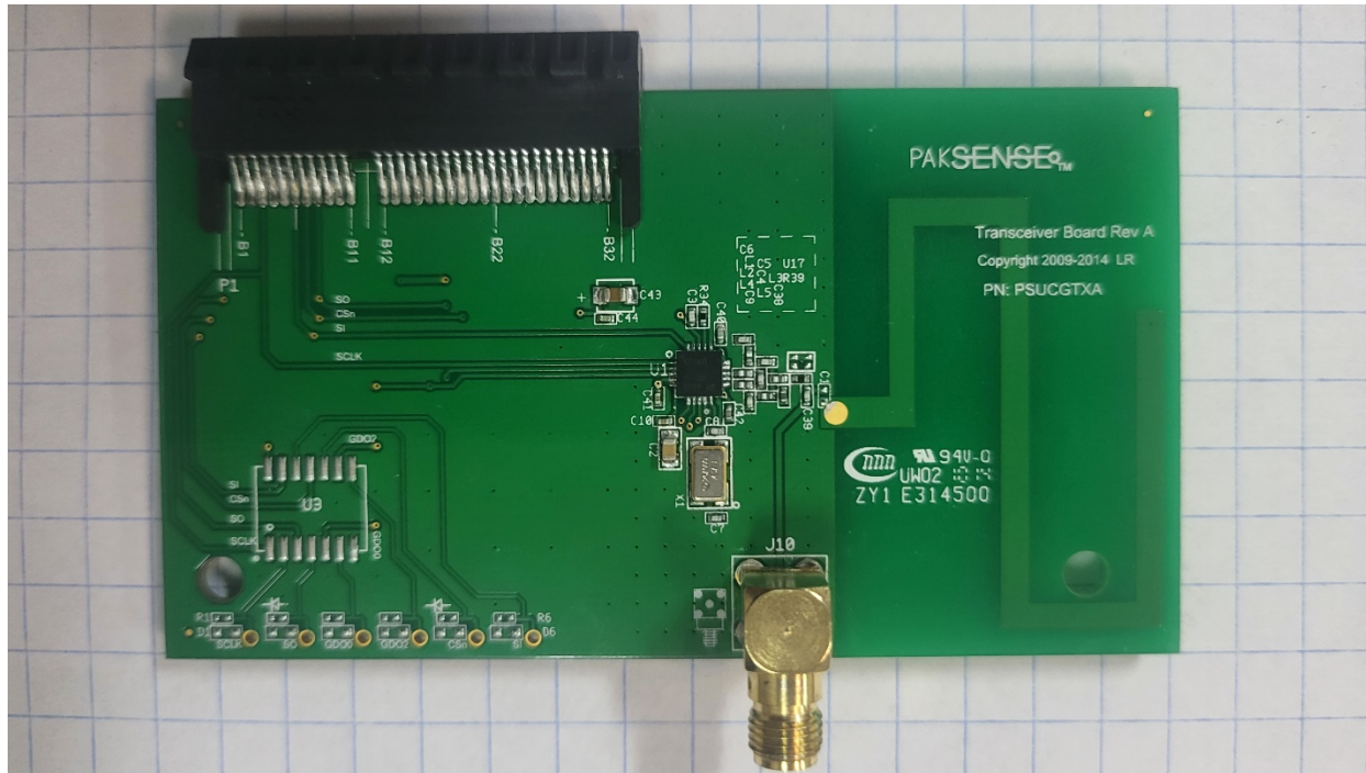
Figure 1. EUT, radio module Top View
