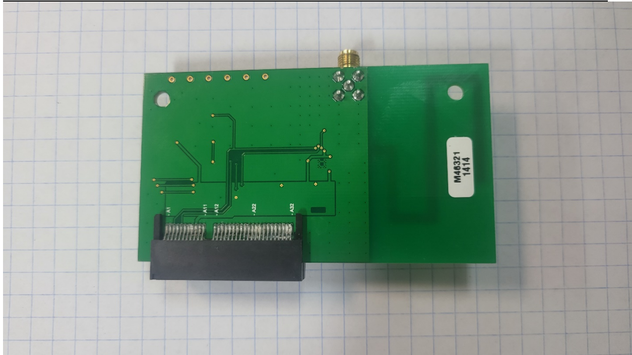
Figure 2. EUT, radio module Bottom View
