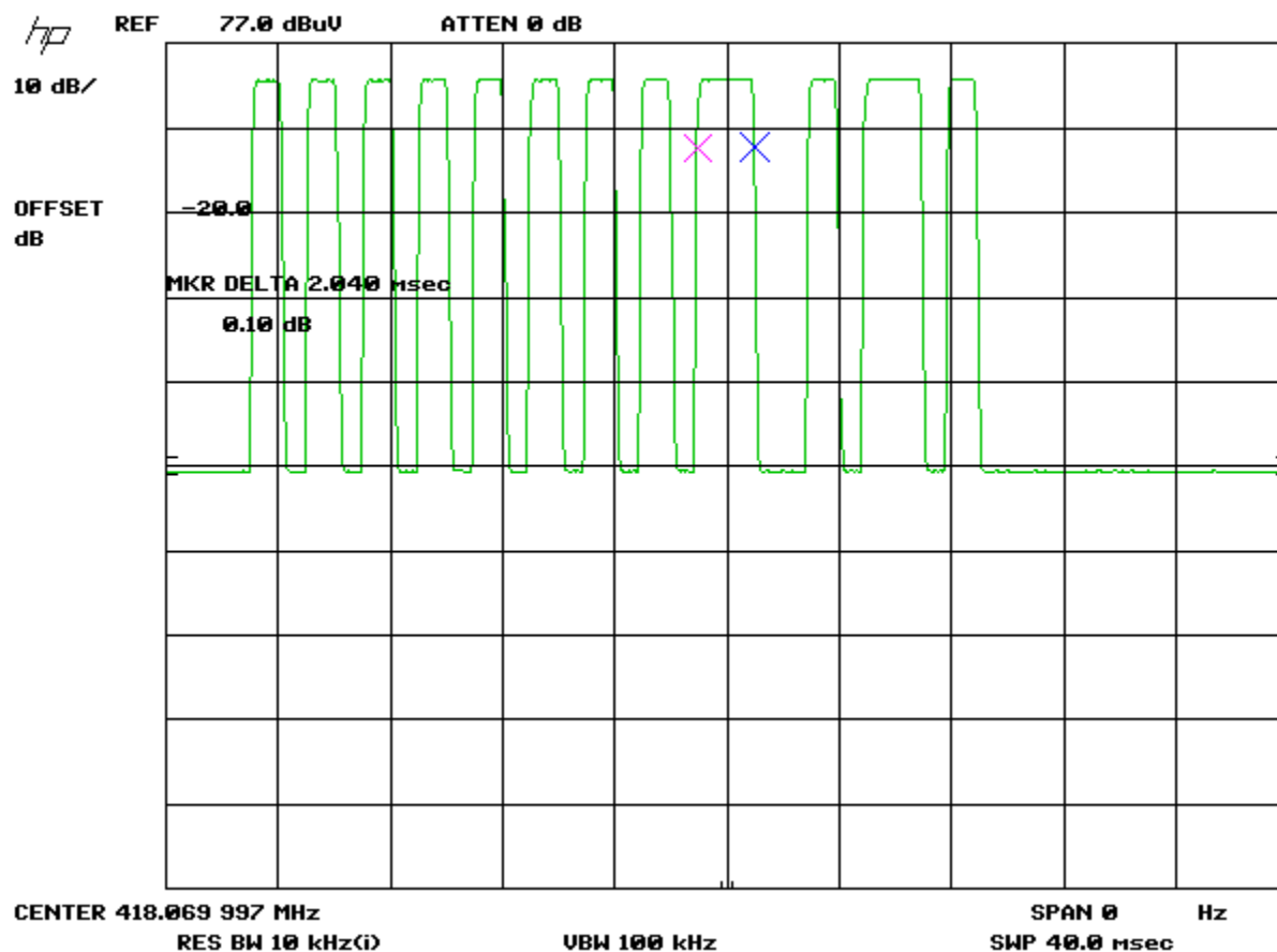
DUTY CYCLE PLOT – LONG PULSES
