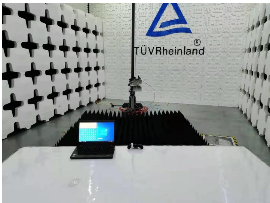
Photograph 4: Set-up photo for Radiated Emission, Above 1GHz
