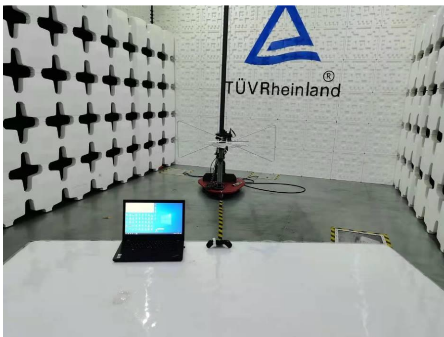
Photograph 3: Set-up photo for Radiated Emission, Below 1GHz
