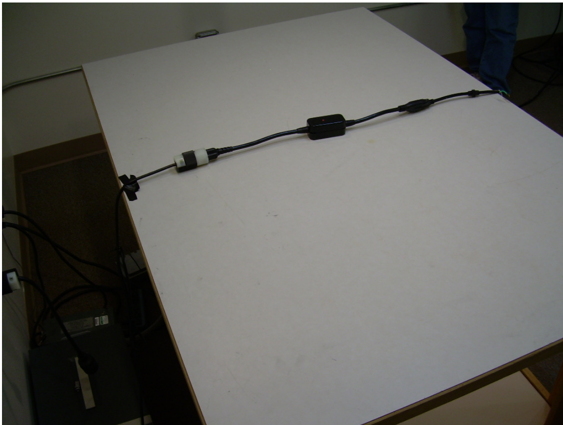
Back View of the Conducted Emission at the AC Mains Setup
