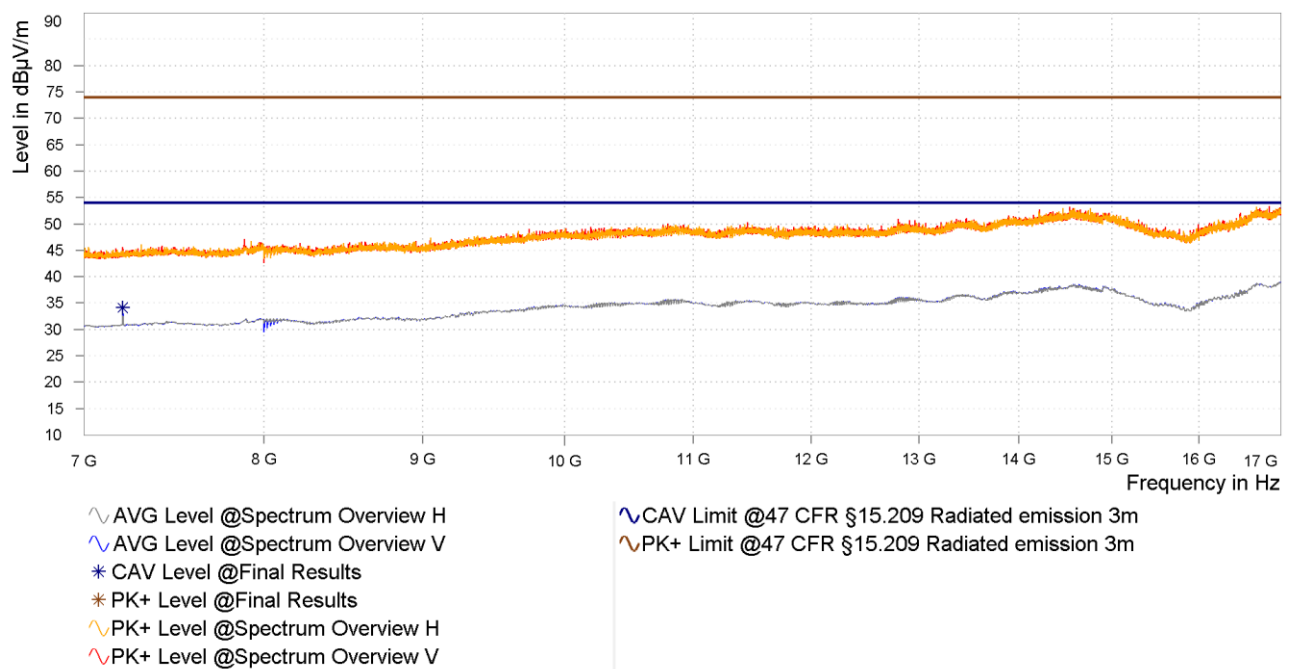
Figure 31: Chart of radiated emissions pre-measurement from 7 GHz to 17 GHz on lowest channel, EUT position Y, antenna polarization vertical and horizontal
