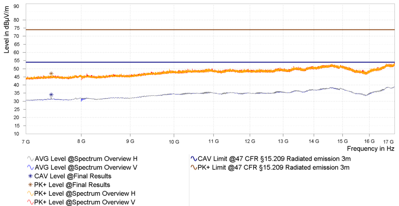
Figure 37: Chart of radiated emissions pre-measurement from 7 GHz to 17 GHz on highest channel, EUT position Y, antenna polarization vertical and horizontal
