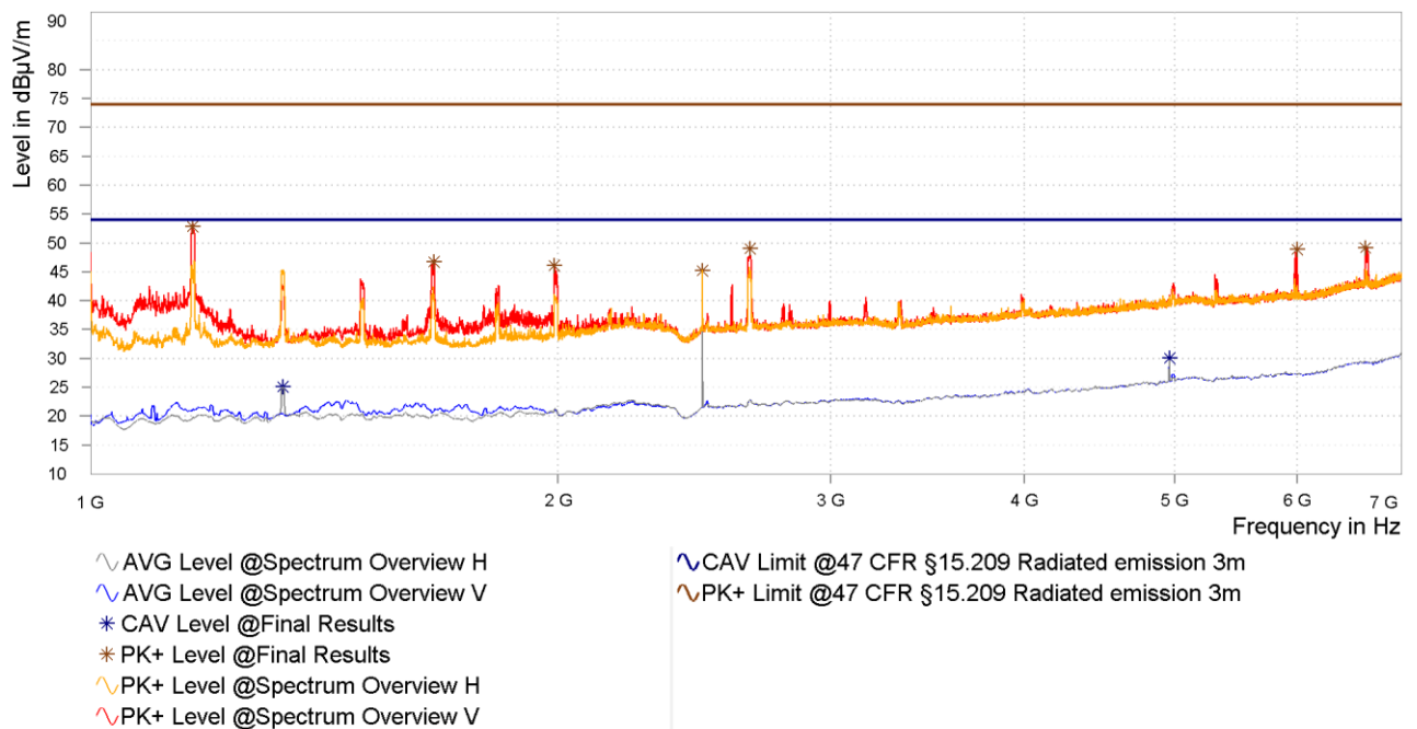
Figure 39: Chart of radiated emissions pre-measurement from 1 GHz to 7 GHz on highest channel, EUT position Y, antenna polarization vertical and horizontal
