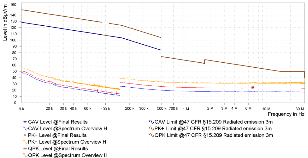
Figure 26: Chart of emissions test below 30 MHz on highest channel, EUT position Y, antenna parallel
