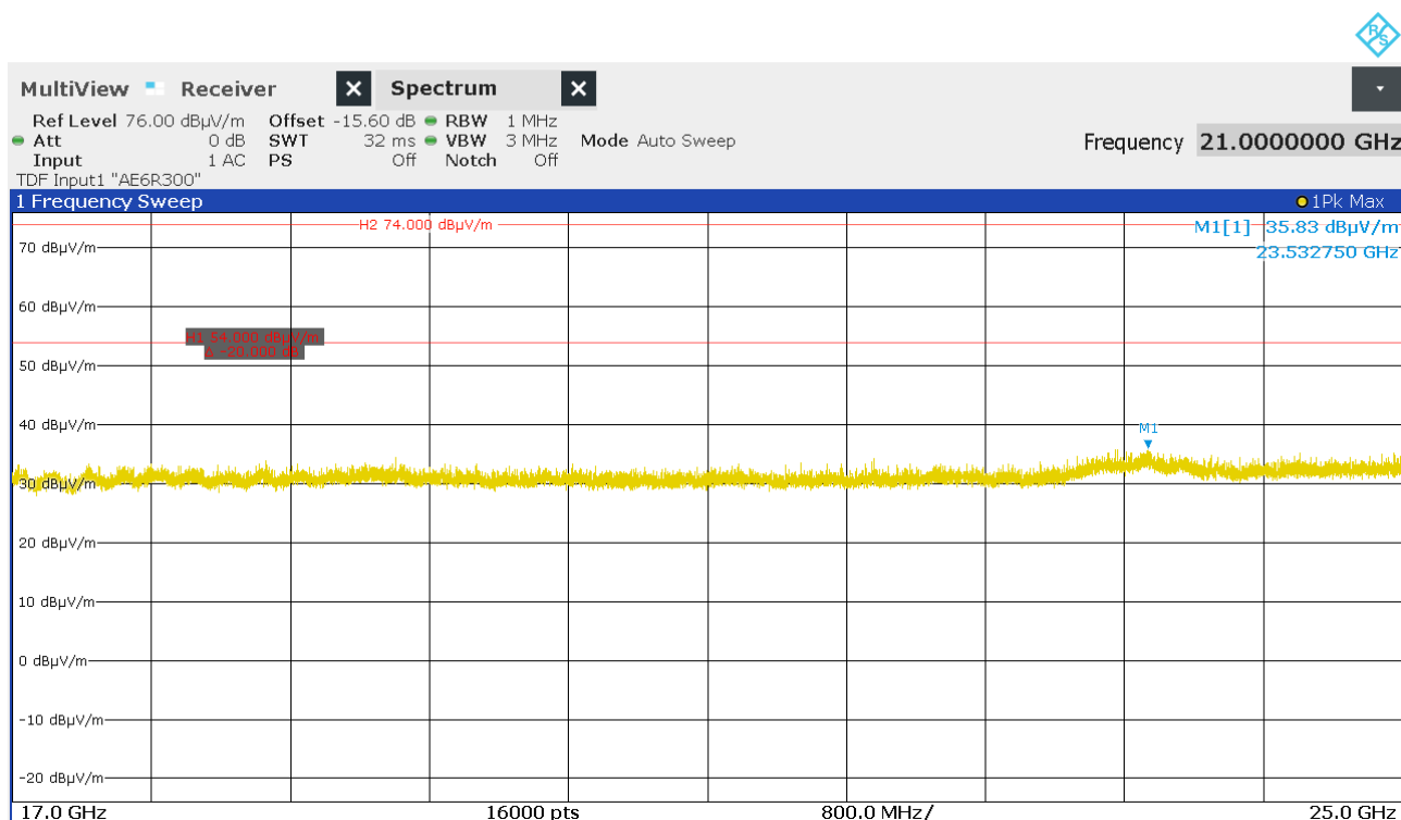
Figure 35: Chart of exploratory emissions measurement from 17 GHz to 25 GHz on middle channel, EUT position X, antenna polarization vertical and horizontal
