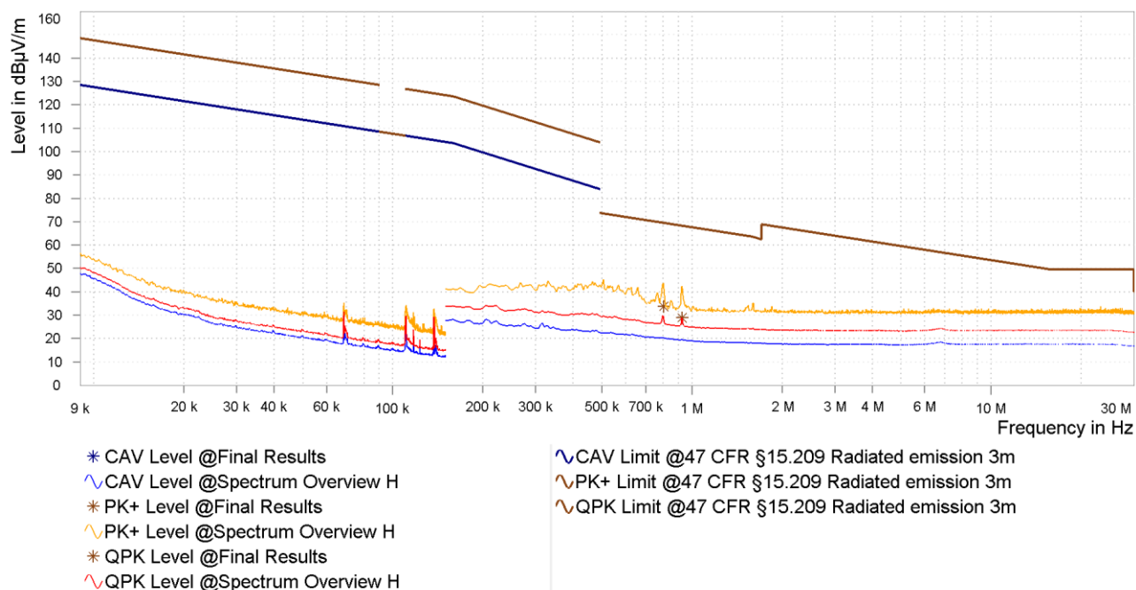
Figure 25: Chart of emissions test below 30 MHz on highest channel, EUT position Y, antenna in line
