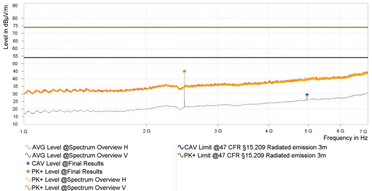
Figure 42: Chart of radiated emissions pre-measurement from 1 GHz to 7 GHz on highest channel, EUT position Y, antenna polarization vertical and horizontal
