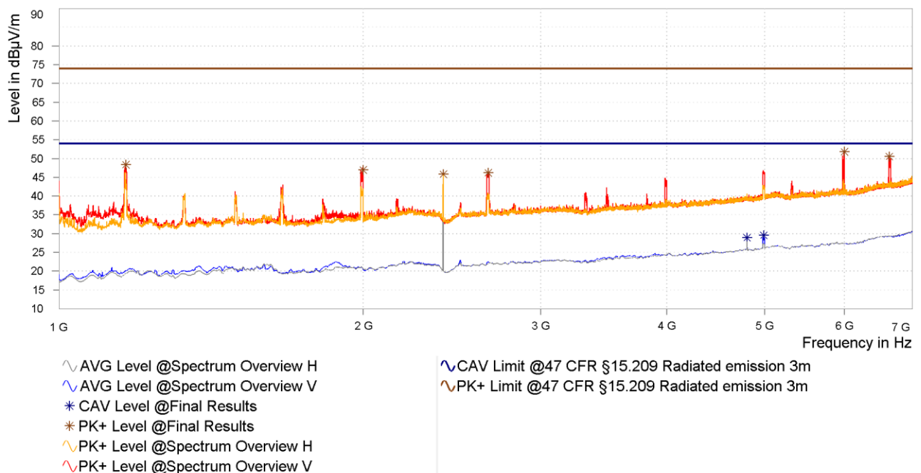
Figure 30: Chart of radiated emissions pre-measurement from 1 GHz to 7 GHz on lowest channel, EUT position Y, antenna polarization vertical and horizontal
