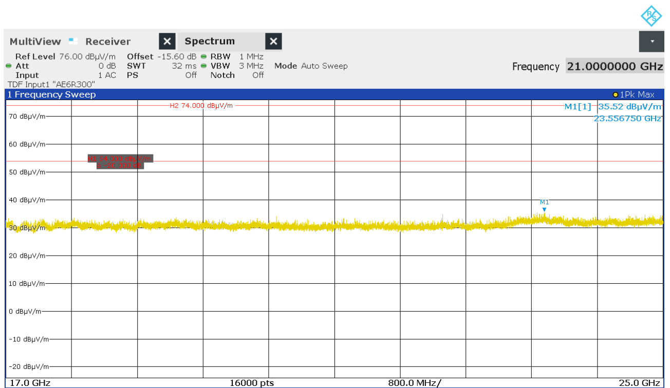
Figure 41: Chart of exploratory emissions measurement from 17 GHz to 25 GHz on highest channel, EUT position X, antenna polarization vertical and horizontal
