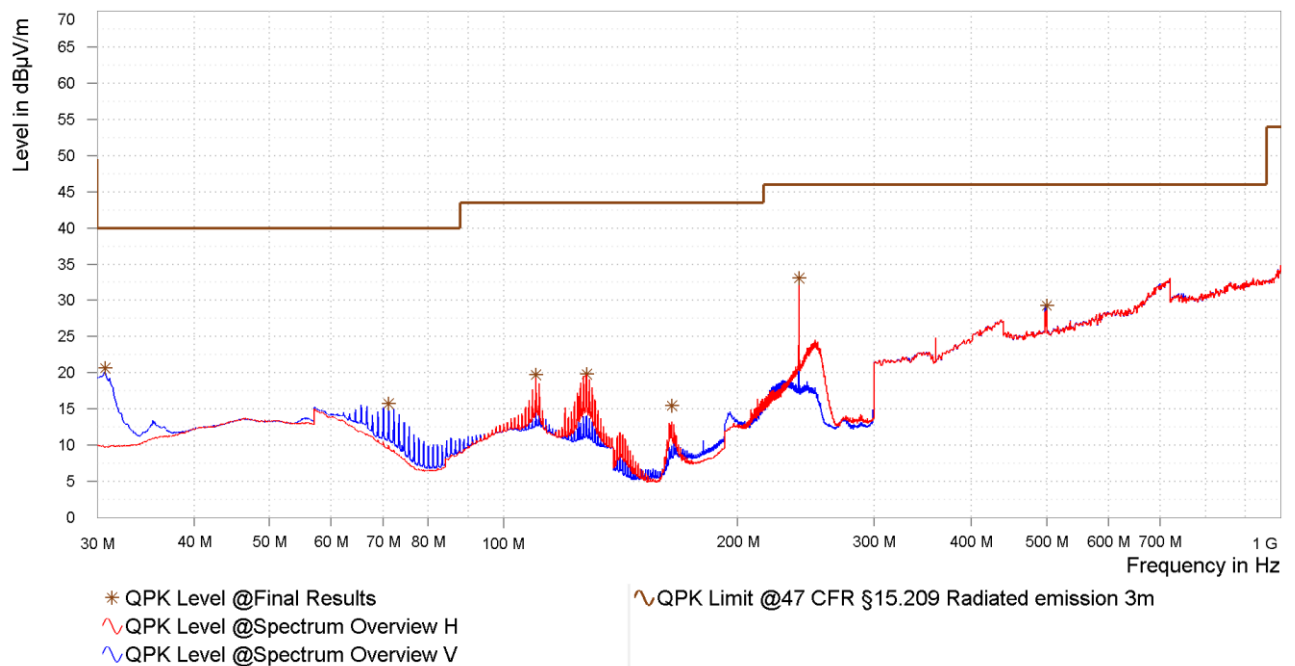
Figure 28: Chart of radiated emissions test from 30 MHz to 1 GHz on highest channel, EUT position Y, antenna polarization vertical and horizontal
