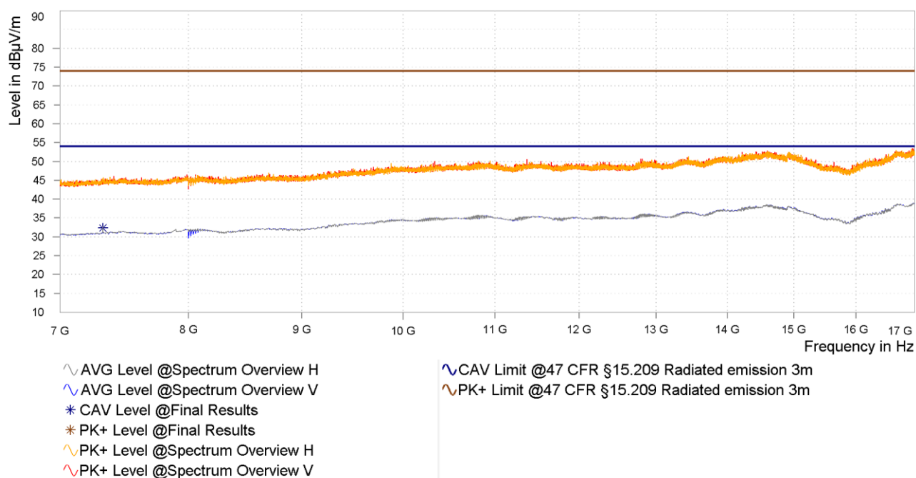
Figure 34: Chart of radiated emissions pre-measurement from 7 GHz to 17 GHz on middle channel, EUT position Y, antenna polarization vertical and horizontal
