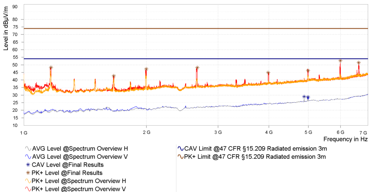
Figure 33: Chart of radiated emissions pre-measurement from 1 GHz to 7 GHz on middle channel, EUT position Y, antenna polarization vertical and horizontal
