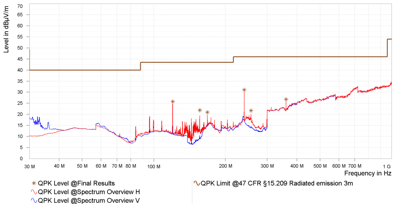
Figure 27: Chart of radiated emissions test from 30 MHz to 1 GHz on highest channel, EUT position Y, antenna polarization vertical and horizontal
