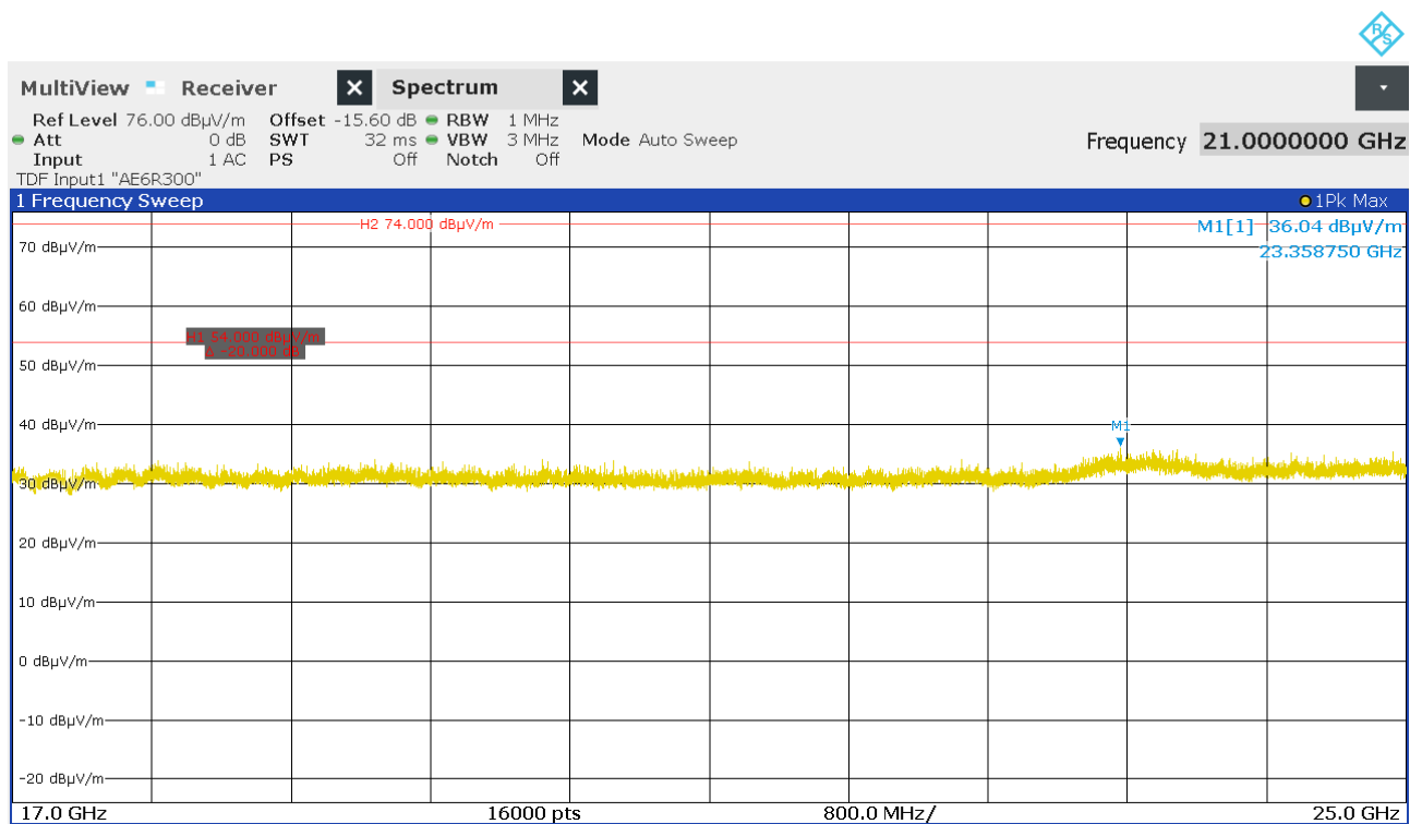
Figure 38: Chart of exploratory emissions measurement from 17 GHz to 25 GHz on highest channel, EUT position X, antenna polarization vertical and horizontal
