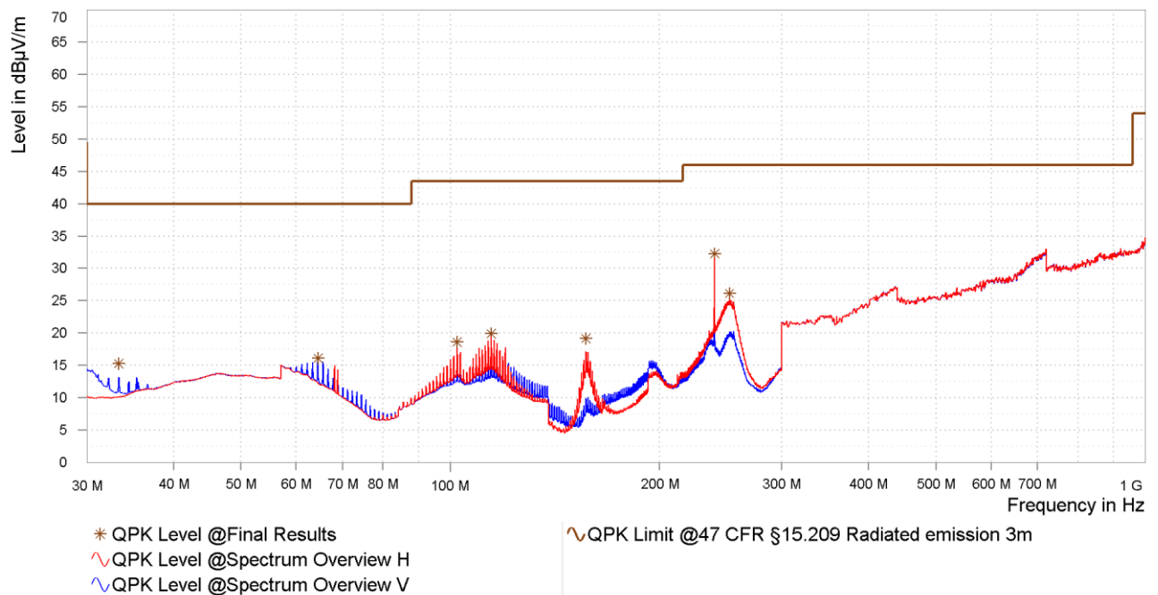
Figure 29: Chart of radiated emissions test from 30 MHz to 1 GHz on highest channel, EUT position Y, antenna polarization vertical and horizontal
