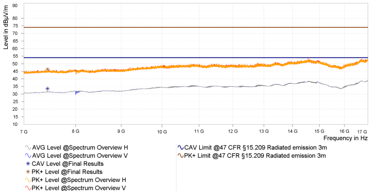
Figure 40: Chart of radiated emissions pre-measurement from 7 GHz to 17 GHz on highest channel, EUT position Y, antenna polarization vertical and horizontal
