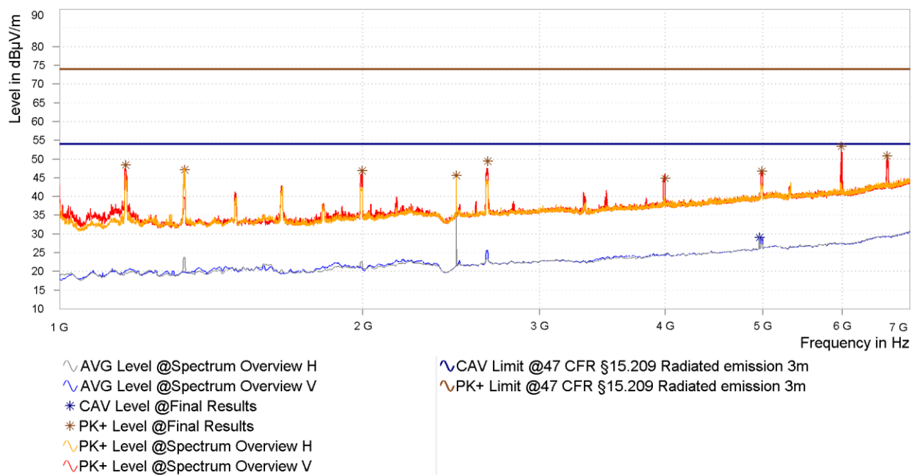
Figure 36: Chart of radiated emissions pre-measurement from 1 GHz to 7 GHz on highest channel, EUT position Y, antenna polarization vertical and horizontal
