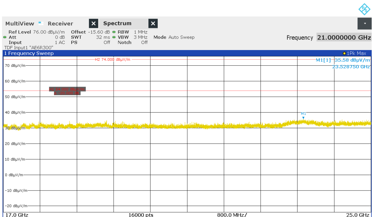
Figure 32: Chart of exploratory radiated emissions measurement from 17 GHz to 25 GHz on lowest channel, EUT position X, antenna polarization vertical and horizontal
