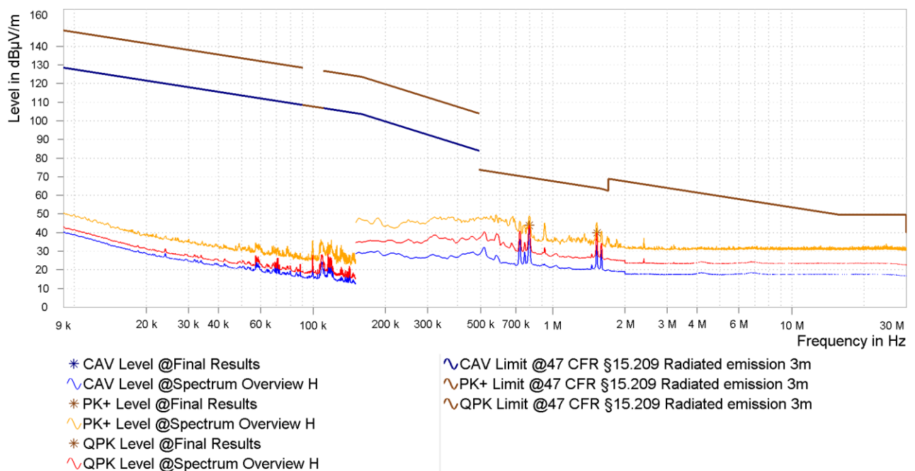
Figure 24: Chart of emissions test below 30 MHz on highest channel, EUT position Y, antenna parallel
