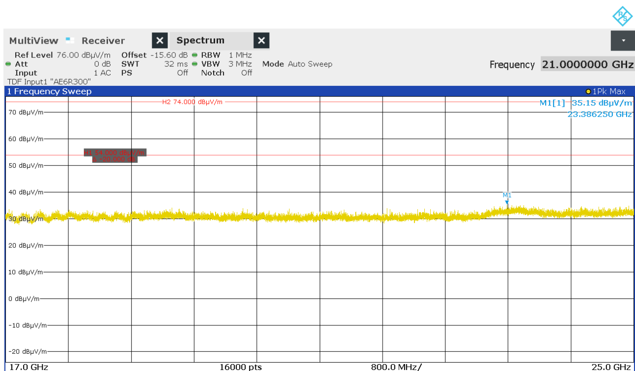
Figure 44: Chart of exploratory emissions measurement from 17 GHz to 25 GHz on highest channel, EUT position X, antenna polarization vertical and horizontal
