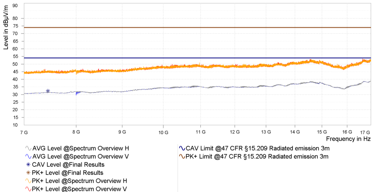
Figure 43: Chart of radiated emissions pre-measurement from 7 GHz to 17 GHz on highest channel, EUT position Y, antenna polarization vertical and horizontal
