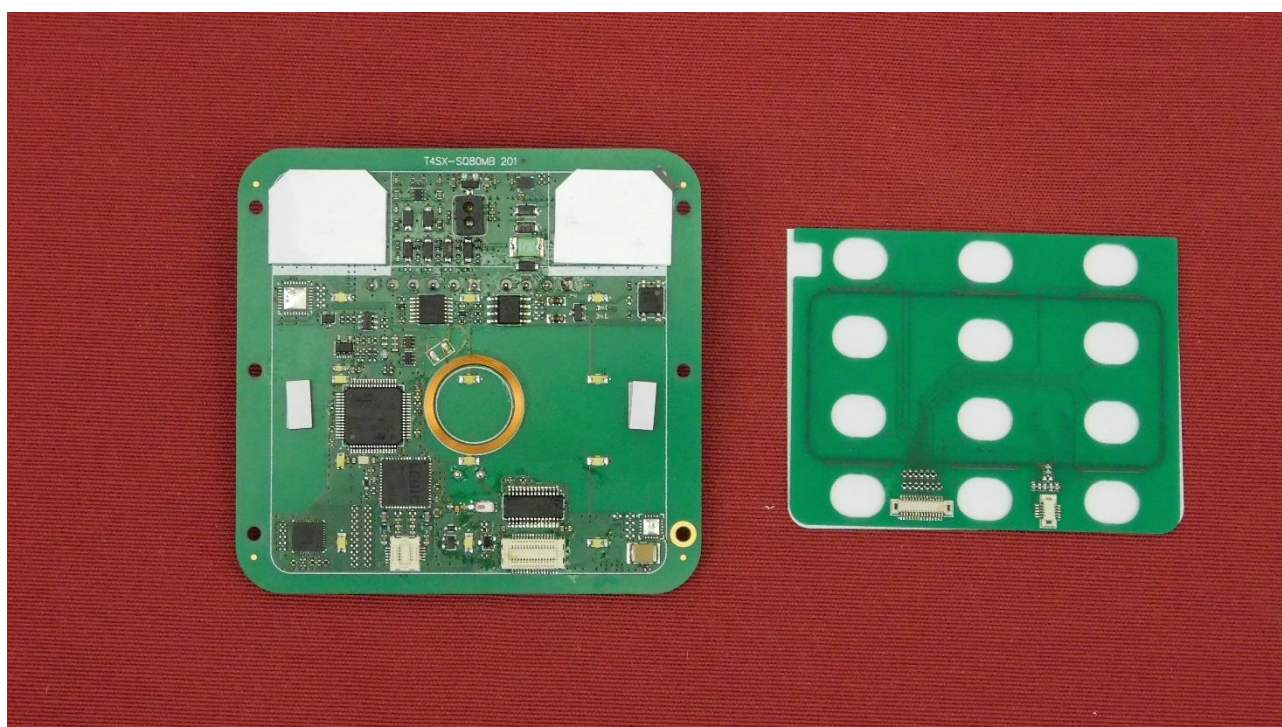
Picture 6: Main PCB and touch PCB decoupled
