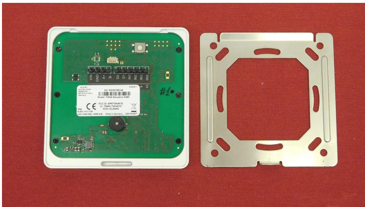
Picture 3 EUT – rear view with demounted metallic support
