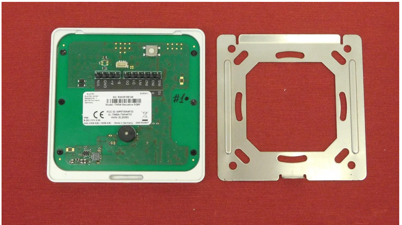
Picture 3 EUT – rear view with demounted metallic support
