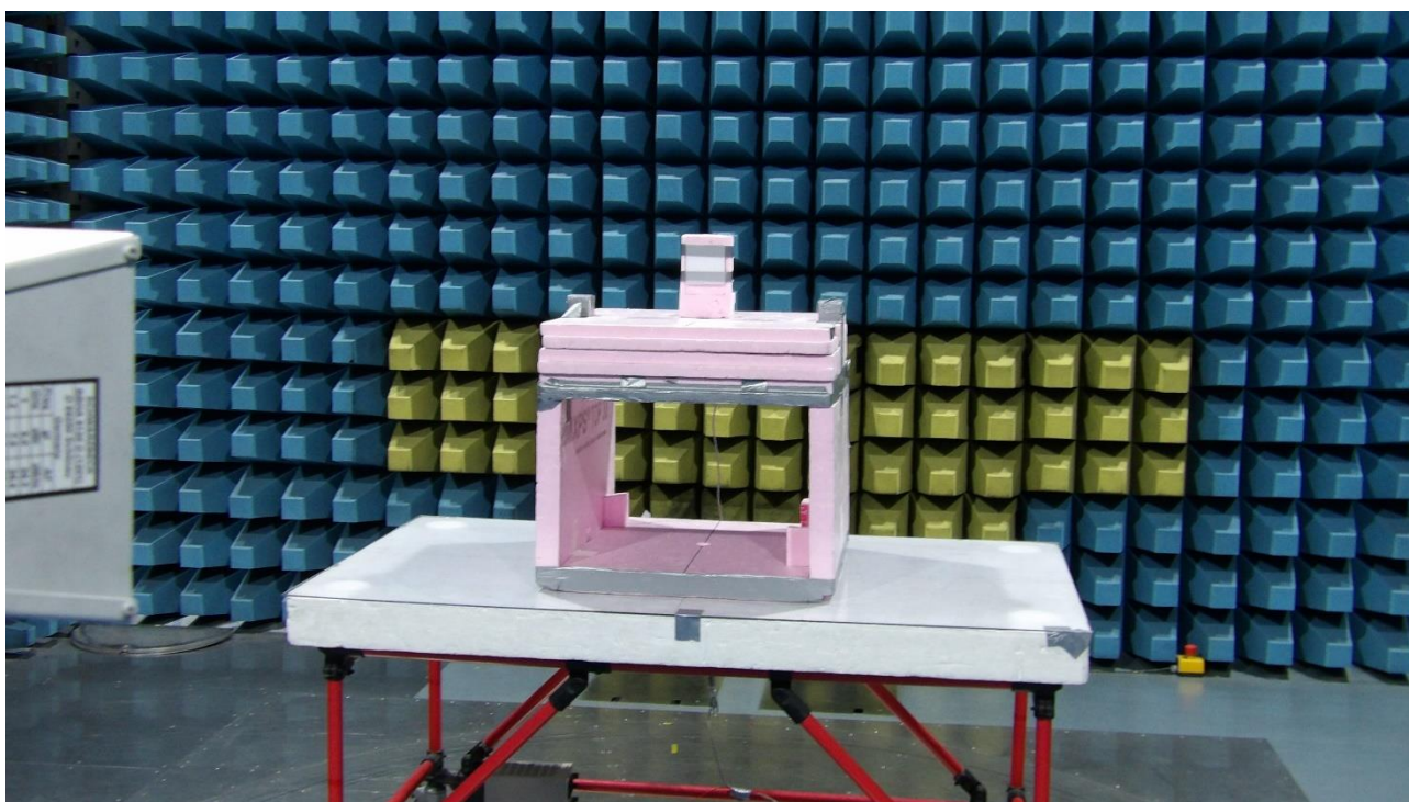
Picture 15: SAC, radiated emission test 1 GHz – 13 GHz (rear view)
