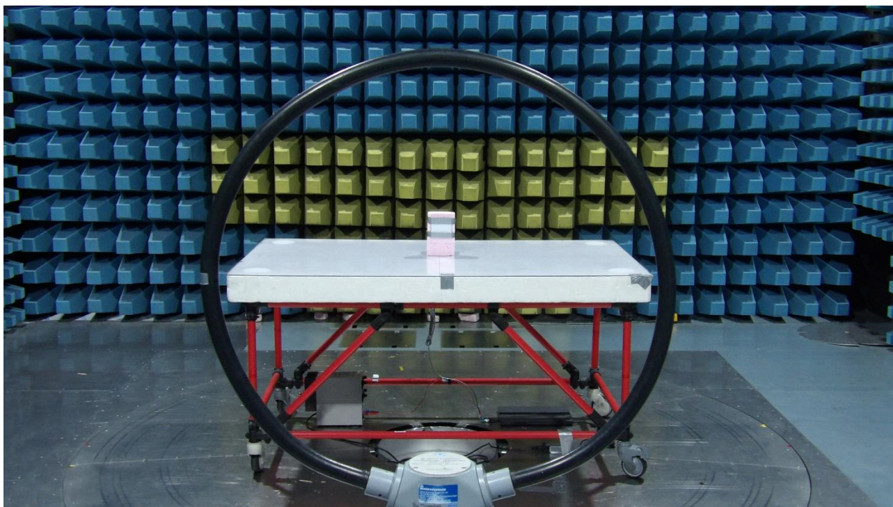
Picture 11: SAC, test setup radiated emission test 9 kHz - 30 MHz (rear view)
