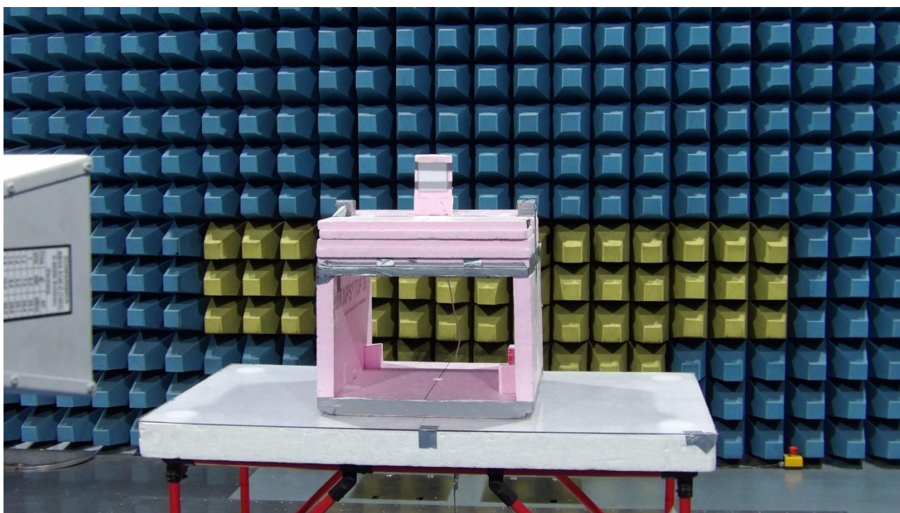
Picture 21: SAC, radiated emission test 1 GHz – 13 GHz (rear view)
