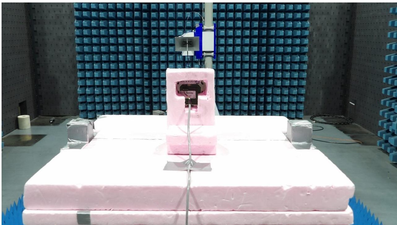
Picture 14: SAC, radiated emission test 1 GHz – 13 GHz (front view)
