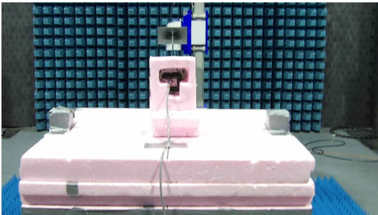
Picture 20: SAC, radiated emission test 1 GHz – 13 GHz (front view)
