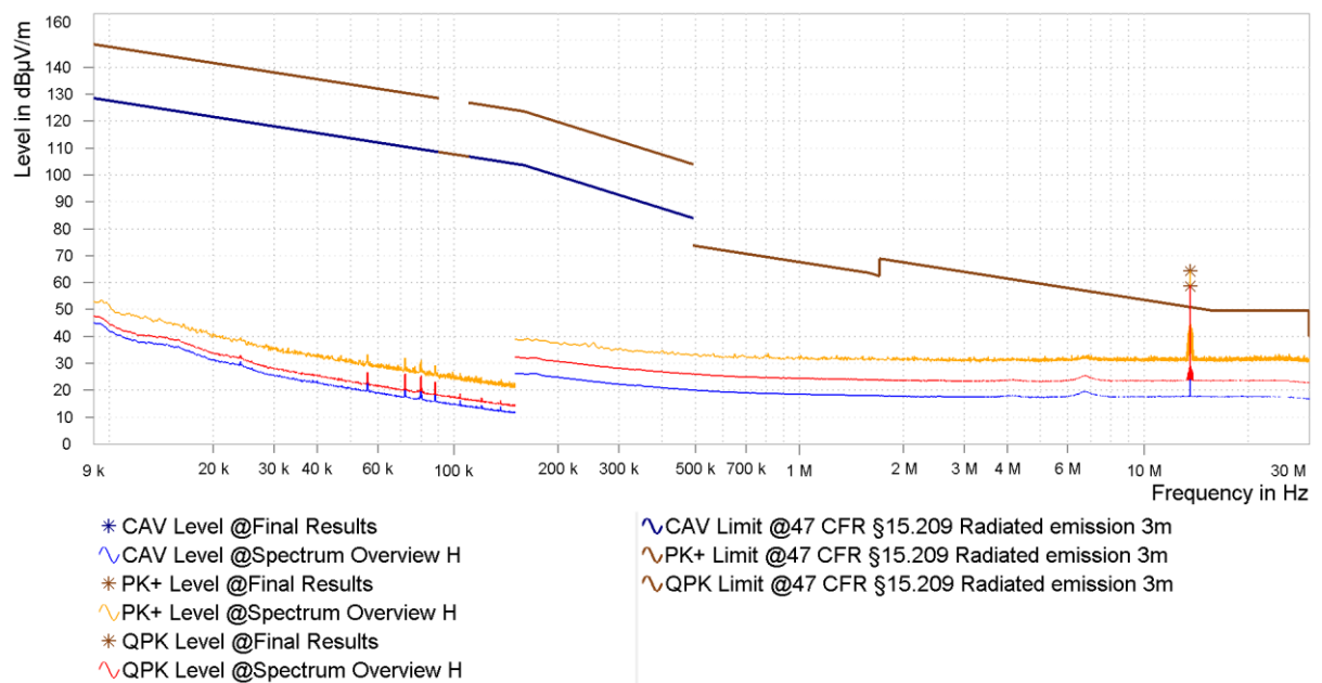
Figure 13: Chart of radiated emissions test below 30 MHz, EUT position Y, antenna polarization in line, without tag
