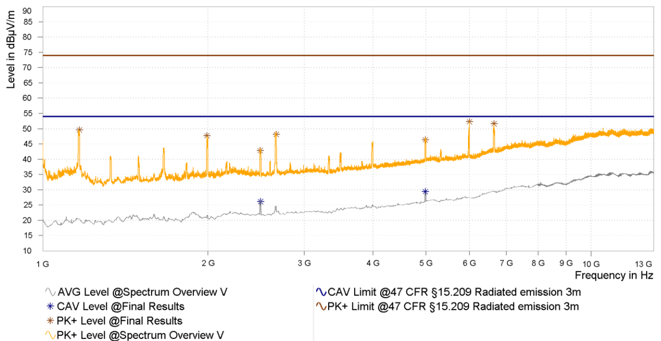
Figure 17: Chart of emissions test from 1 GHz to 13 GHz, EUT position Y, antenna polarization vertical, without tag
