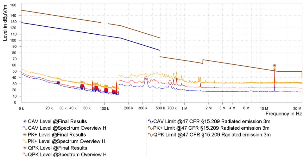
Figure 12: Chart of radiated emissions test below 30 MHz, EUT position Y, antenna polarization parallel, without tag
