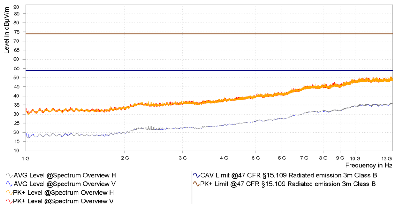
Figure 19: Chart of emissions test from 1 GHz to 13 GHz, EUT position Y, antenna polarization vertical and horizontal, with tag
