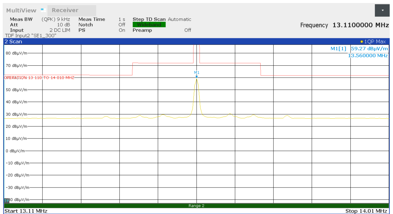
Figure 10: Chart of emission within the band 13.110 MHz to 14.010 MHz, EUT in position Y, with tag, antenna in line at 3 m distance
