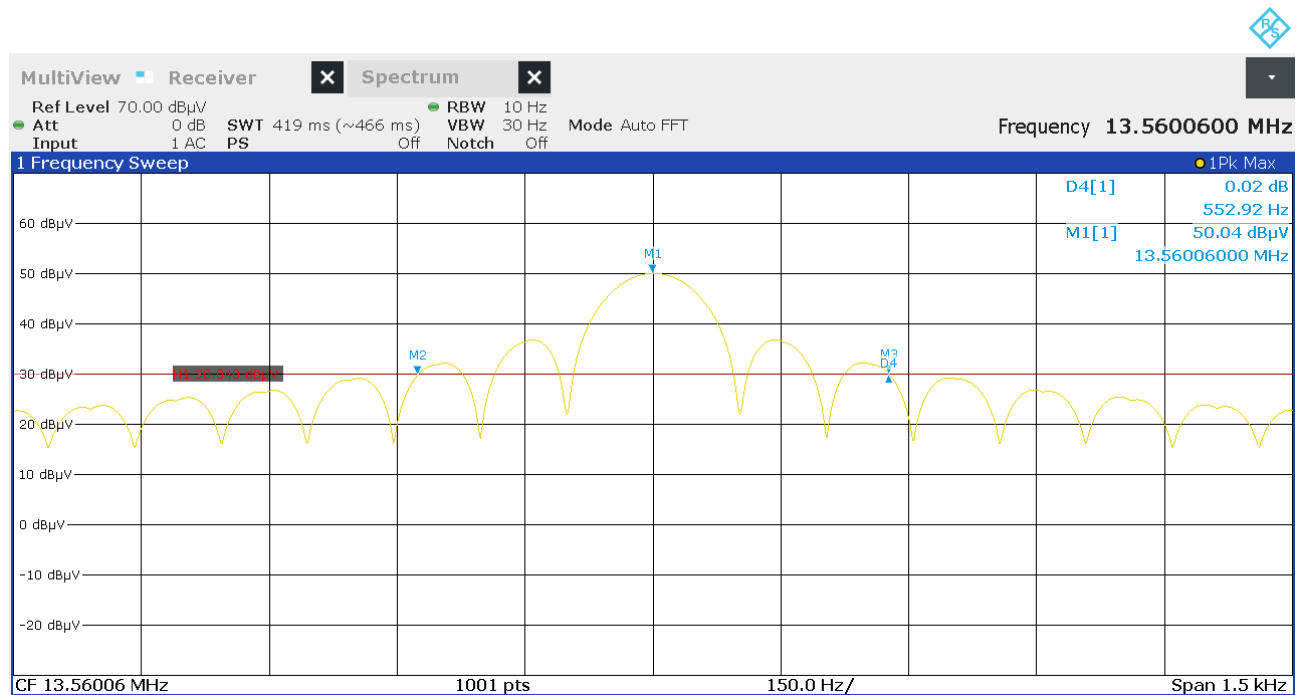
Figure 8: Chart of 20 dB bandwidth tests at normal conditions, without tag
