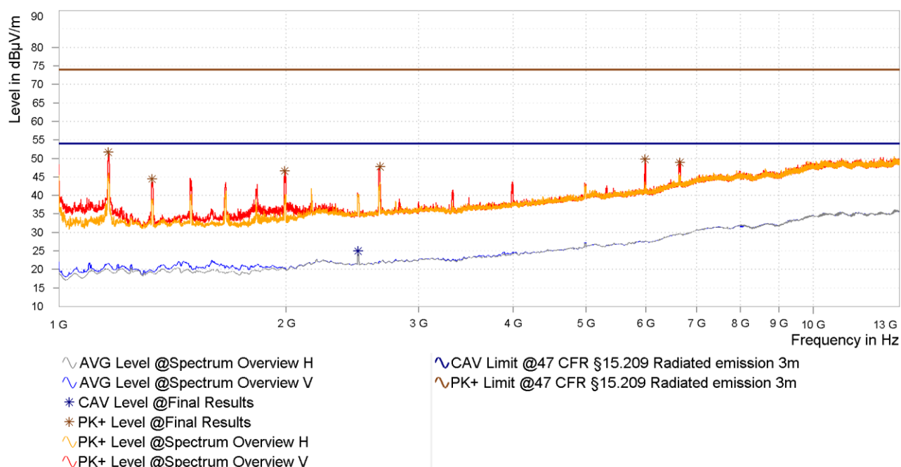
Figure 18: Chart of emissions test from 1 GHz to 13 GHz, EUT position Y, antenna polarization vertical and horizontal, without tag
