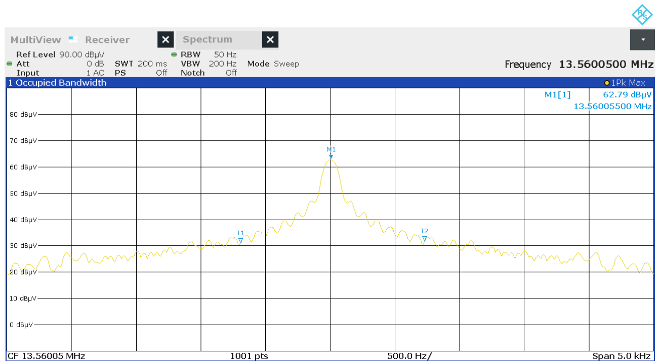
Figure 9: Chart of occupied bandwidth test, without tag
