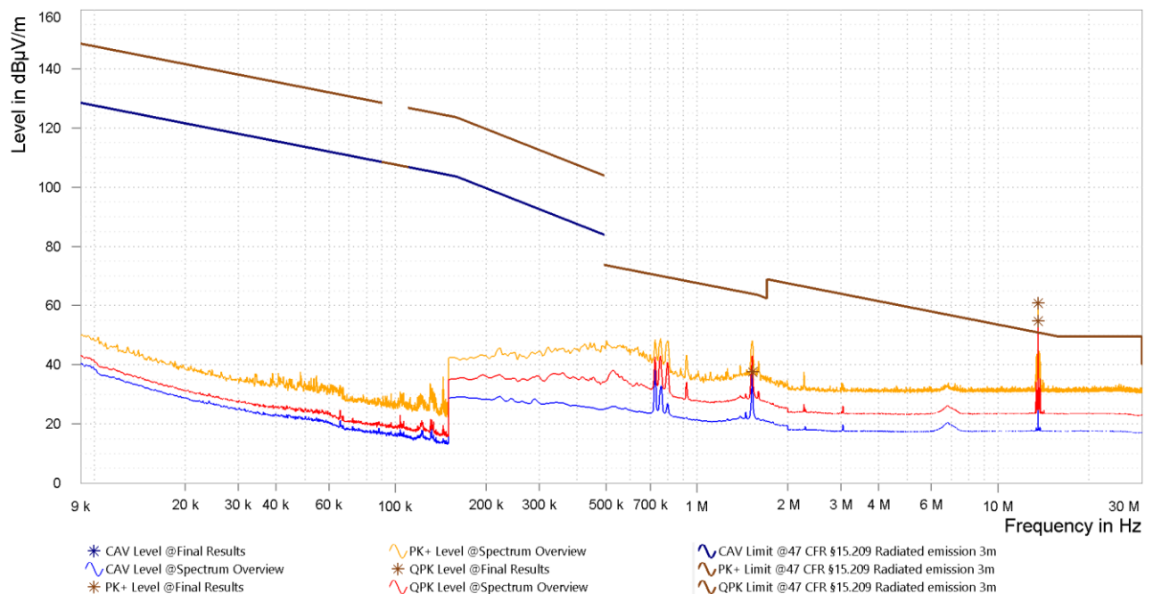
Figure 11: Chart of radiated emissions test below 30 MHz, EUT position Y, antenna polarization in line, with tag
