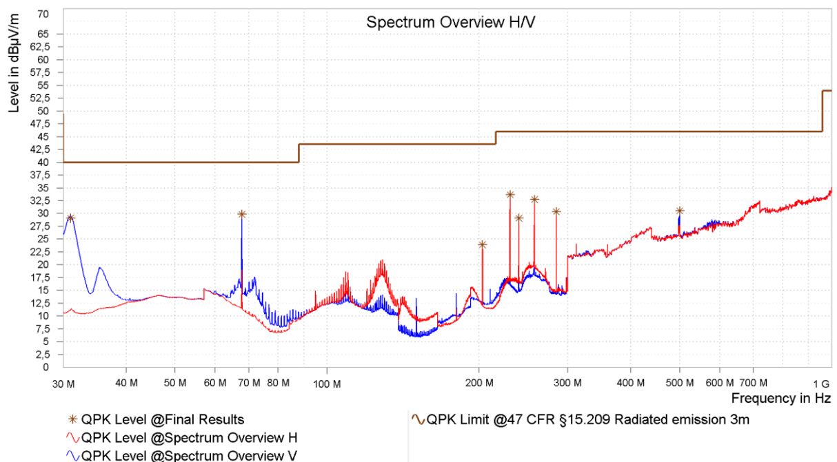
Figure 15: Chart of radiated emissions test from 30 MHz to 1 GHz, EUT position Y, antenna polarization horizontal and vertical, with tag
