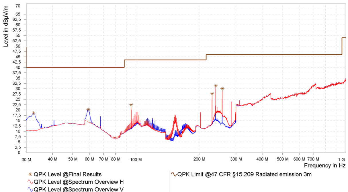
Figure 16: Chart of radiated emissions test from 30 MHz to 1 GHz, EUT position Y, antenna polarization horizontal and vertical, with tag
