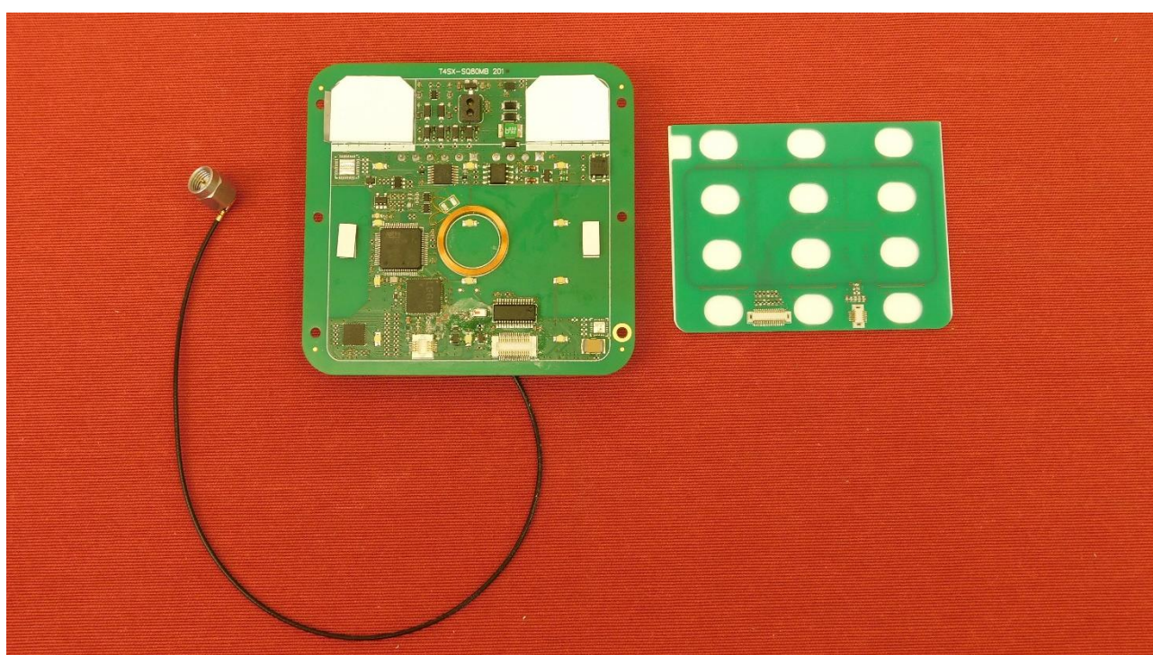
Picture 12: Main PCB and touch PCB decoupled
