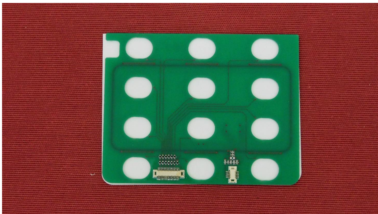
Picture 11: Touch PCB – bottom side
