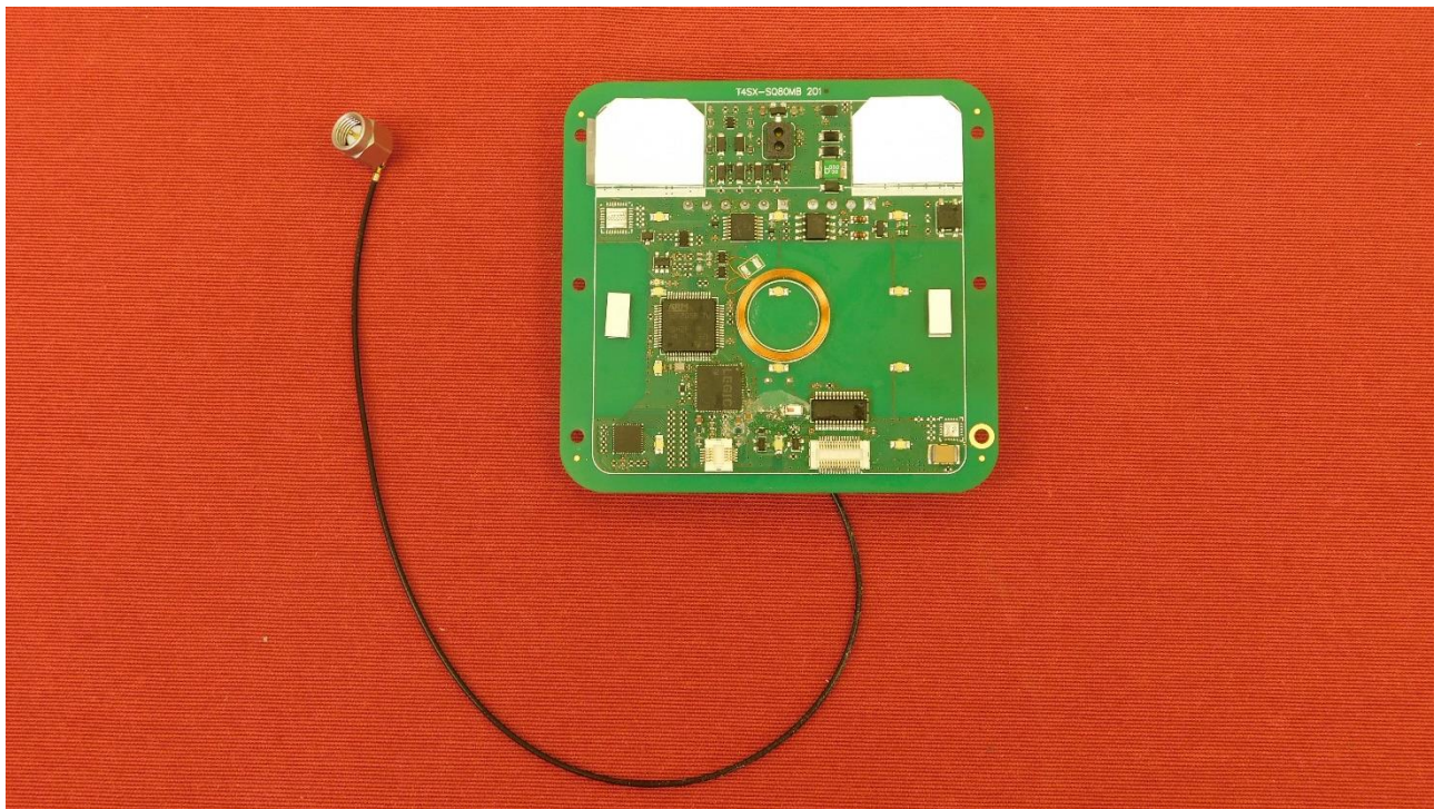
Picture 9: Main PCB – top view
