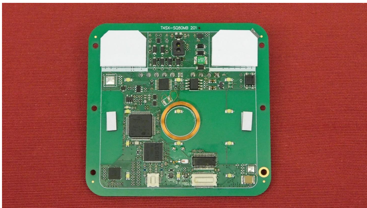
Picture 3: Main PCB – top view
