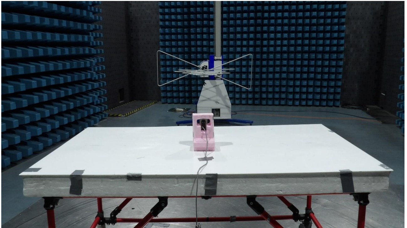
Picture 18: SAC, radiated emission test 30 MHz - 1 GHz (front view)
