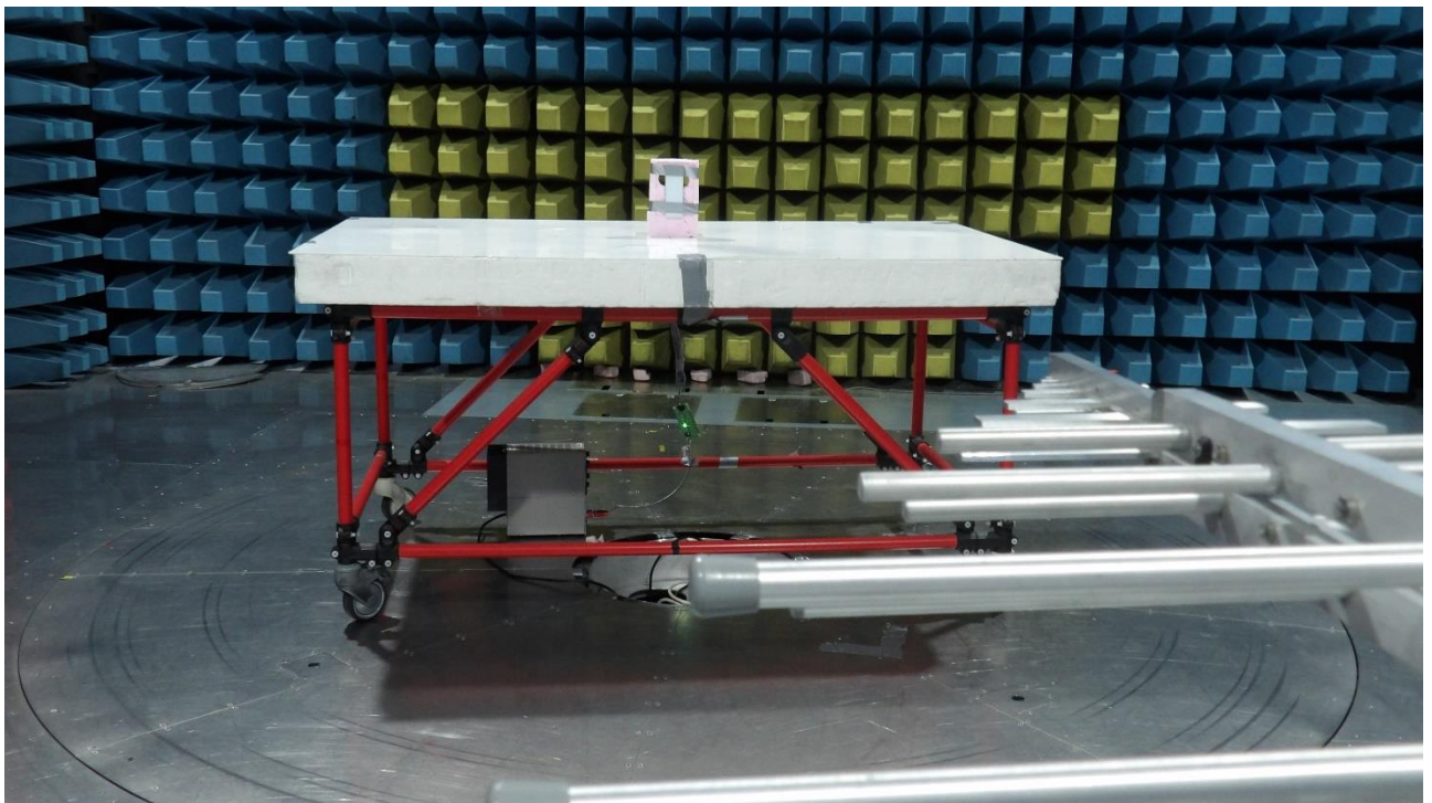
Picture 19: SAC, radiated emission test 30 MHz - 1 GHz (rear view)
