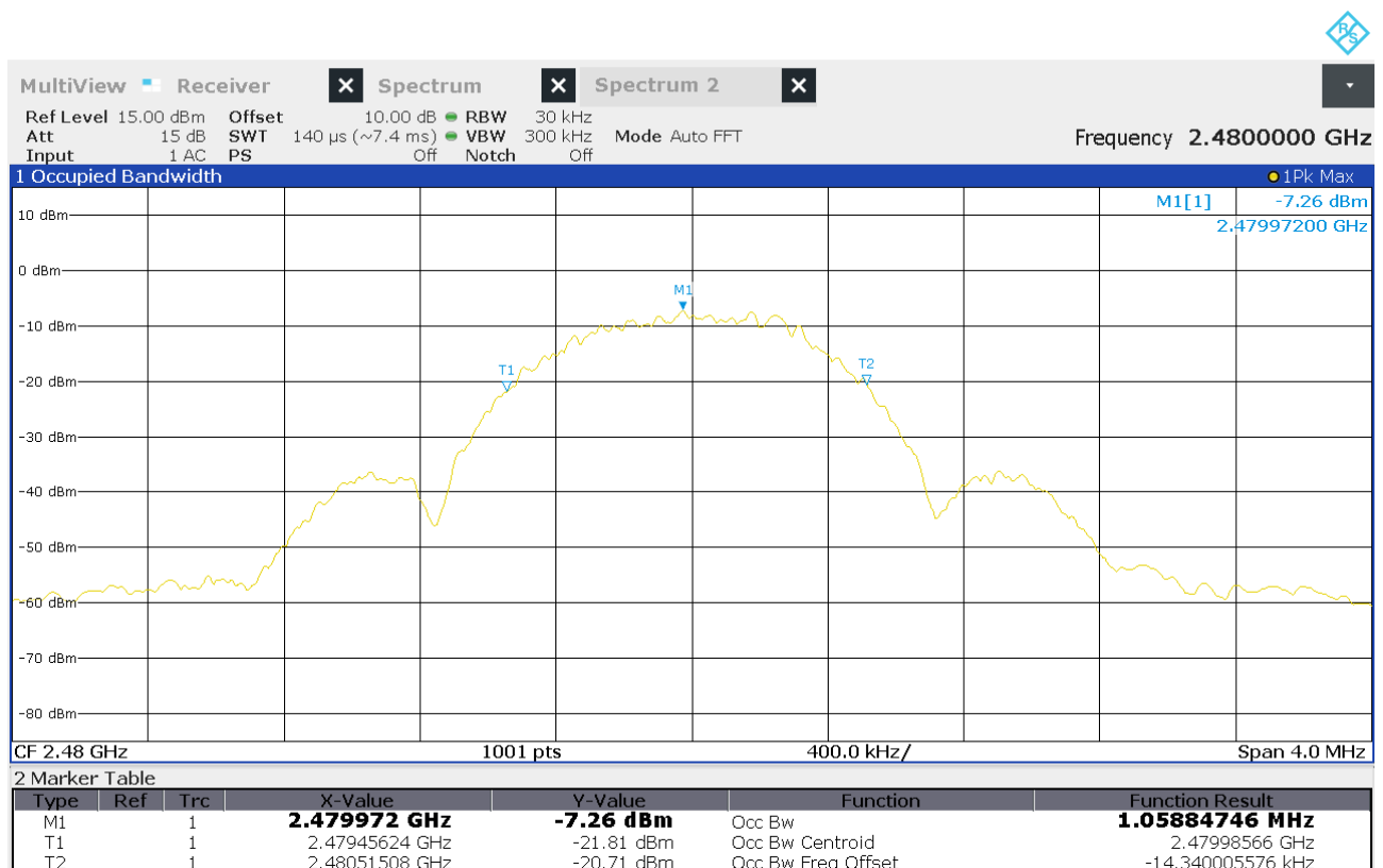
Figure 14: Chart of occupied bandwidth test on highest channel
