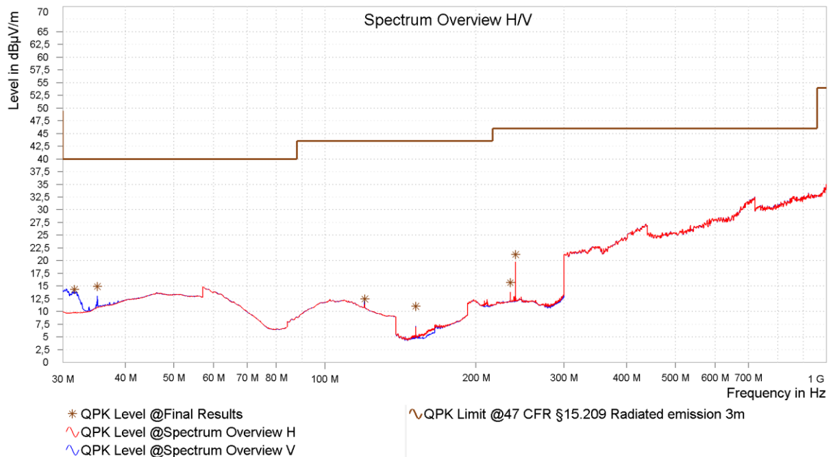
Figure 29: Chart of radiated emissions test from 30 MHz to 1 GHz on lowest channel, EUT position Y, antenna polarization vertical and horizontal
