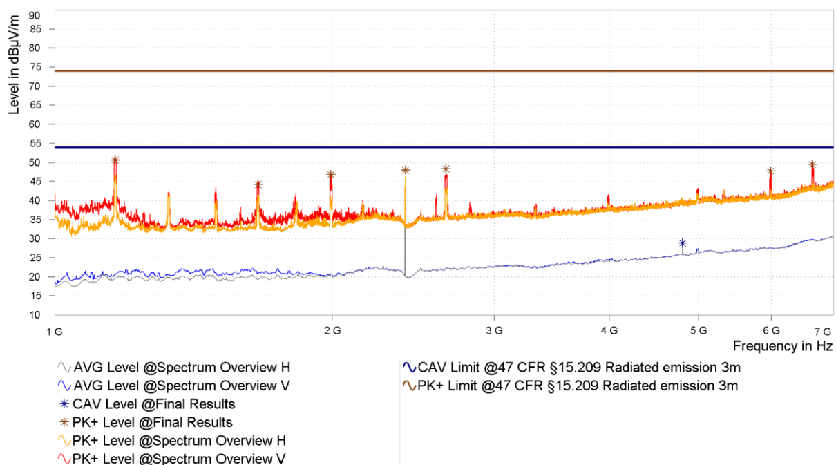
Figure 39: Chart of radiated emissions pre-measurement from 1 GHz to 7 GHz on lowest channel, EUT position Y, antenna polarization vertical and horizontal
