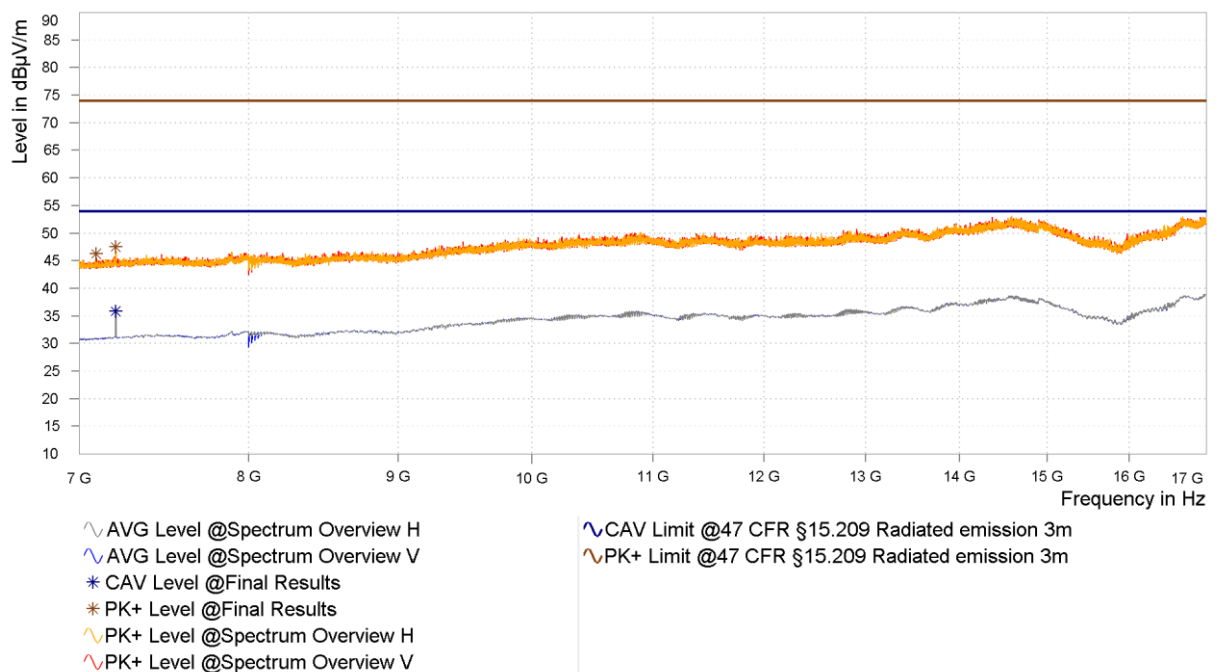
Figure 43: Chart of radiated emissions pre-measurement from 7 GHz to 17 GHz on lowest channel, EUT position Y, antenna polarization vertical and horizontal
