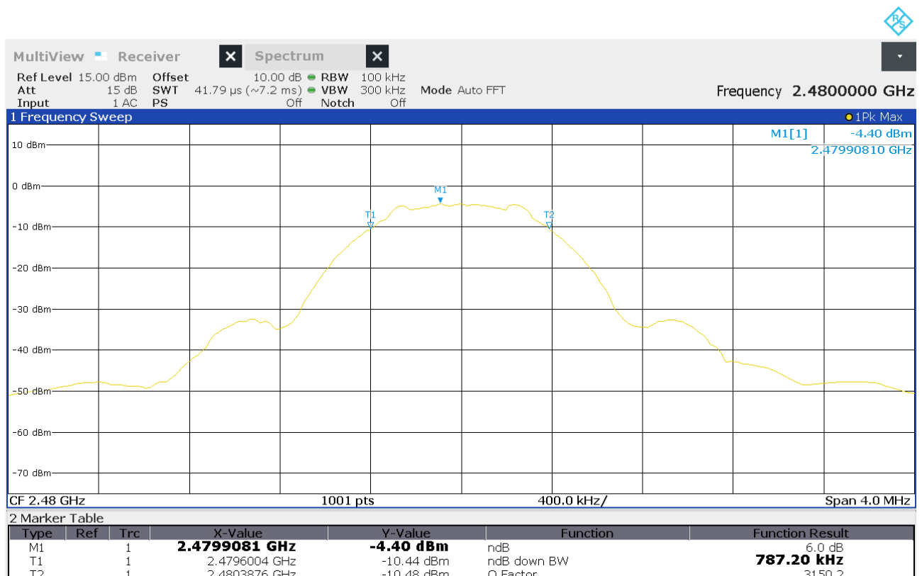
Figure 11: Chart of 6 dB bandwidth test on highest channel
