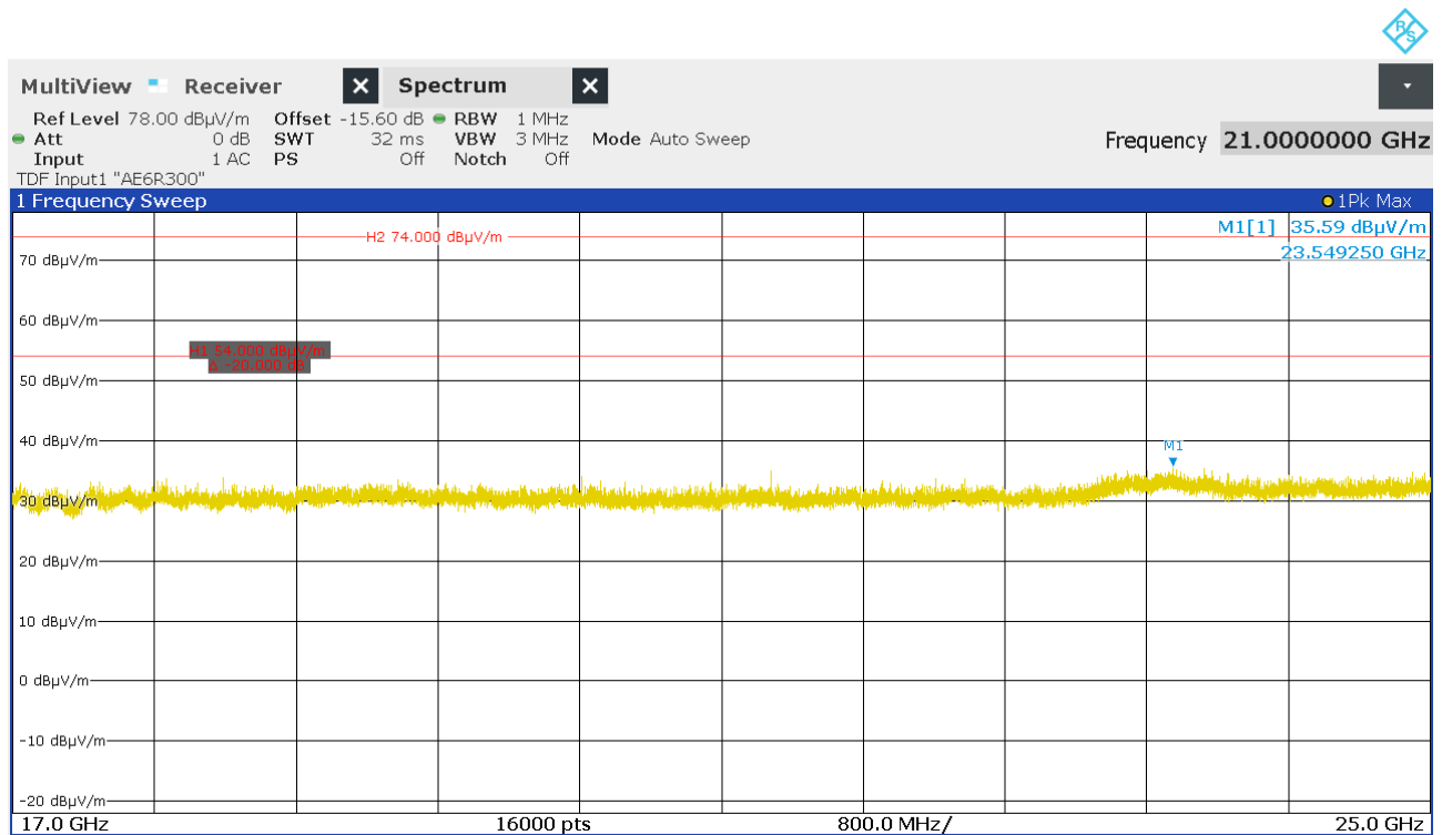
Figure 32: Chart of exploratory radiated emissions measurement from 17 GHz to 25 GHz on lowest channel, EUT position X, antenna polarization horizontal and vertical
