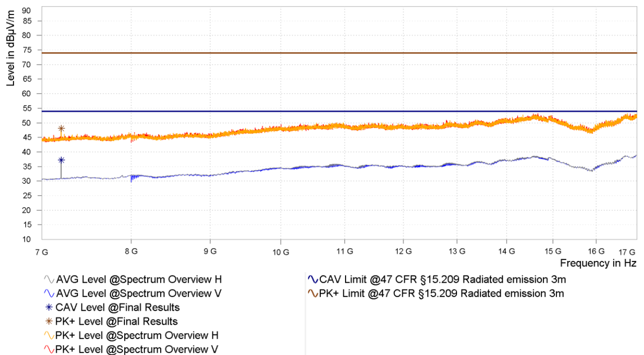
Figure 31: Chart of radiated emissions pre-measurement from 7 GHz to 17 GHz on lowest channel, EUT position Y, antenna polarization horizontal and vertical
