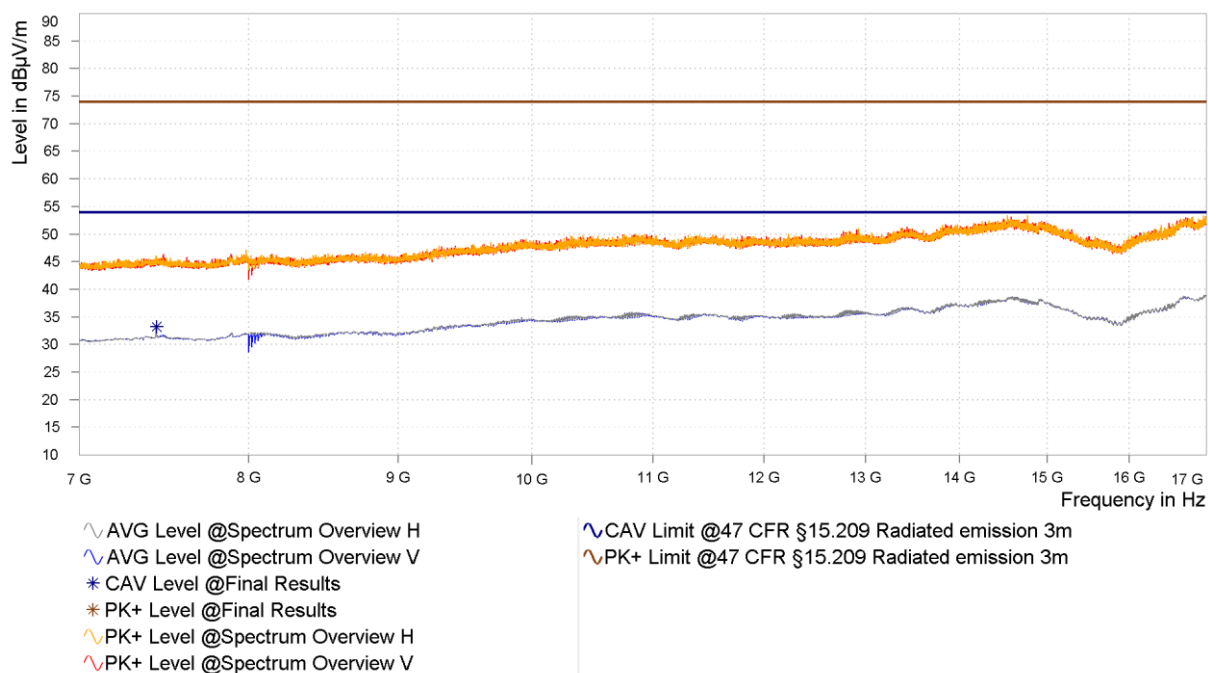
Figure 37: Chart of radiated emissions pre-measurement from 7 GHz to 17 GHz on highest channel, EUT position Y, antenna polarization horizontal and vertical
