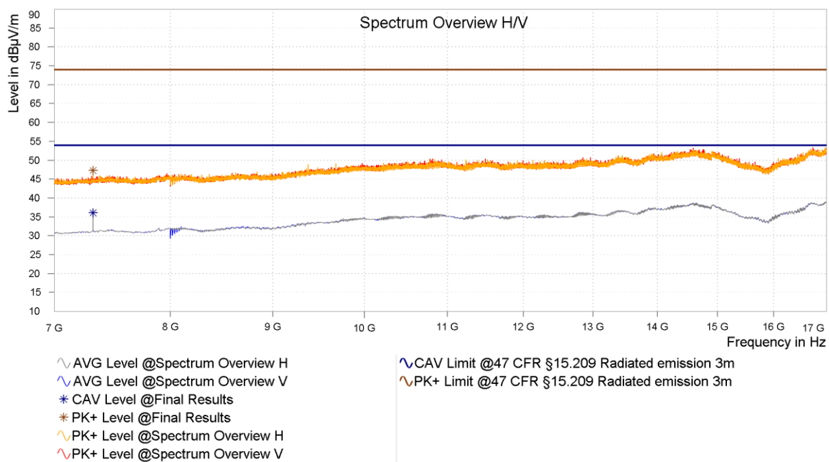
Figure 34: Chart of radiated emissions pre-measurement from 7 GHz to 17 GHz on middle channel, EUT position Y, antenna polarization horizontal and vertical
