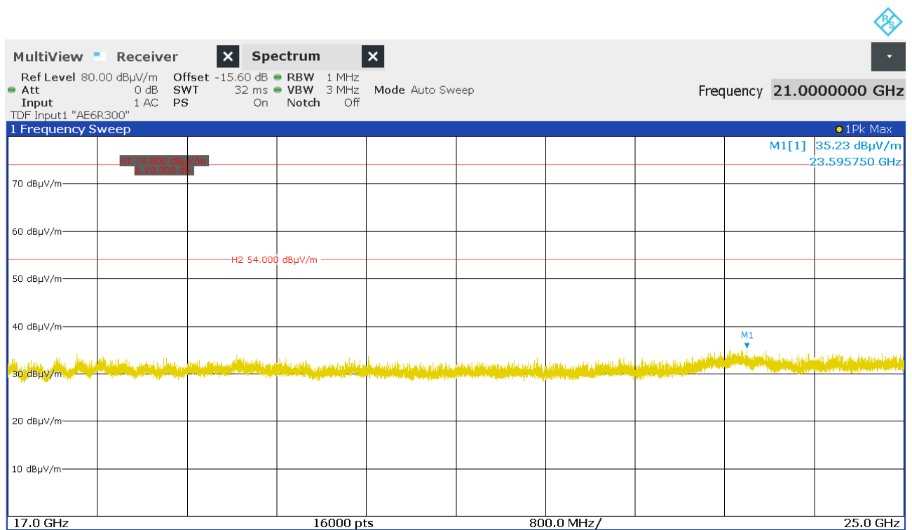
Figure 41: Chart of exploratory radiated emissions measurement from 17 GHz to 25 GHz on lowest channel, EUT position X, antenna polarization vertical and horizontal
