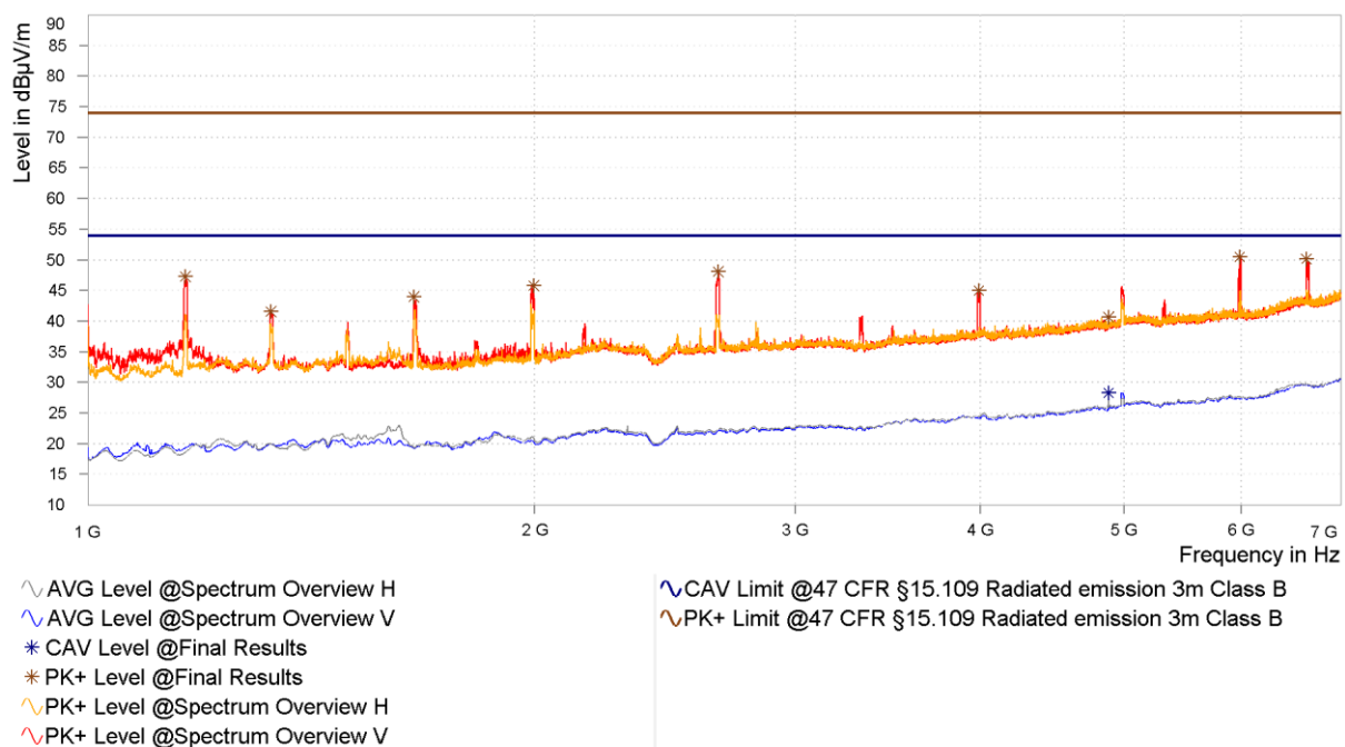
Figure 33: Chart of radiated emissions pre-measurement from 1 GHz to 7 GHz on middle channel, EUT position Y, antenna polarization horizontal and vertical
