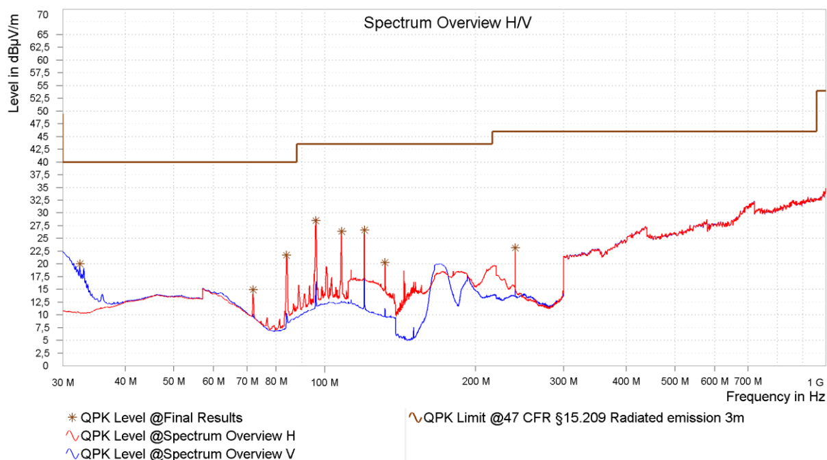
Figure 27: Chart of radiated emissions test from 30 MHz to 1 GHz on lowest channel, EUT position Y, antenna polarization vertical and horizontal
