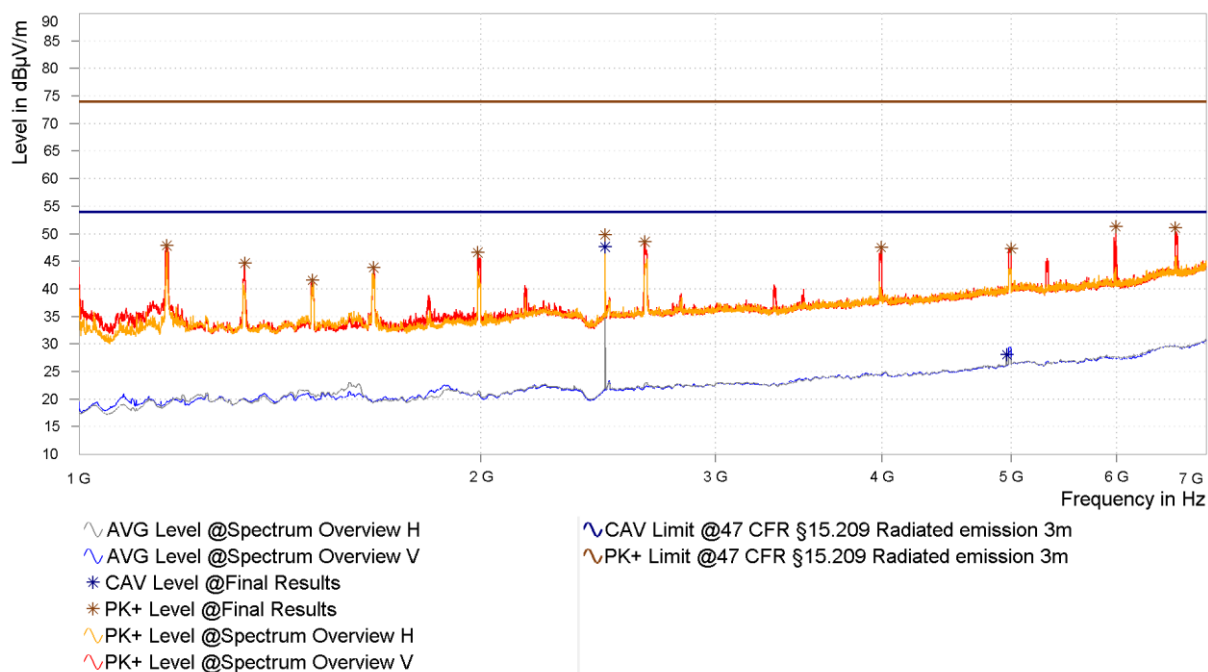
Figure 36: Chart of radiated emissions pre-measurement from 1 GHz to 7 GHz on highest channel, EUT position Y, antenna polarization horizontal and vertical
