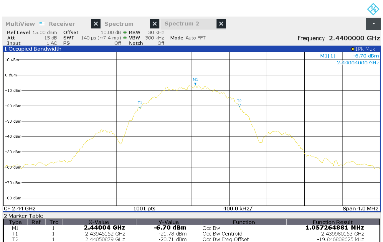
Figure 13: Chart of occupied bandwidth test on middle channel
