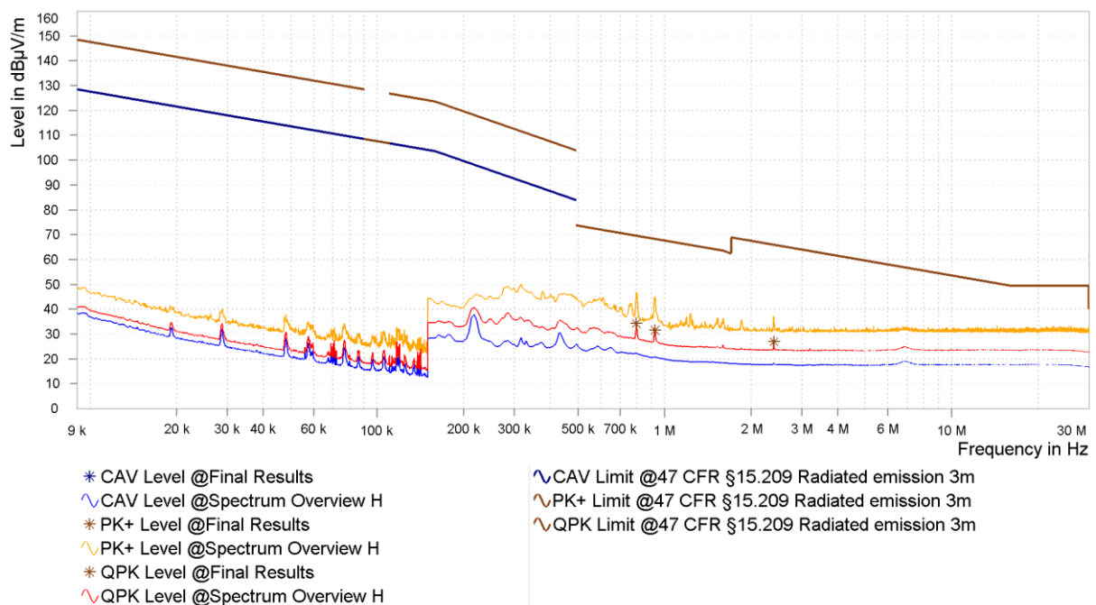
Figure 24: Chart of emissions test below 30 MHz on lowest channel, EUT position Y, antenna parallel
