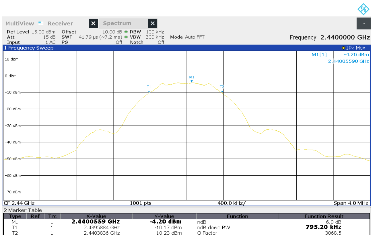
Figure 10: Chart of 6 dB bandwidth test on middle channel
