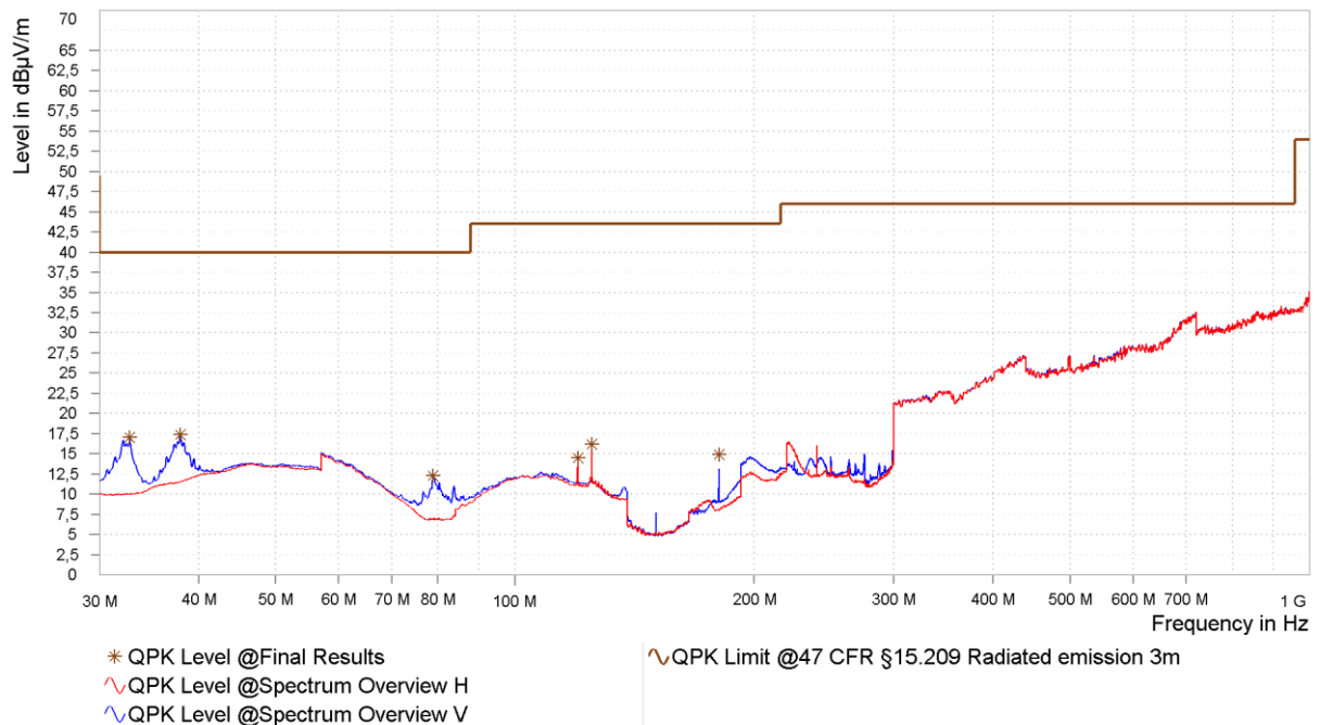
Figure 28: Chart of radiated emissions test from 30 MHz to 1 GHz on lowest channel, EUT position Y, antenna polarization vertical and horizontal
