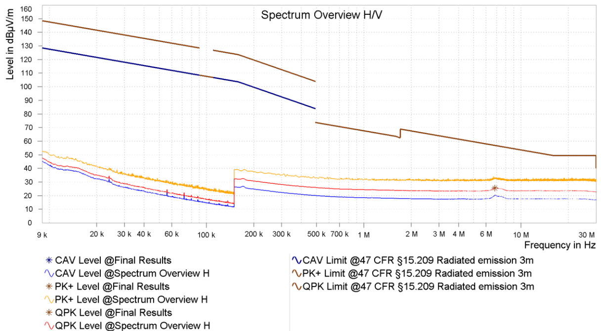
Figure 26: Chart of emissions test below 30 MHz on lowest channel, EUT position Y, antenna parallel
