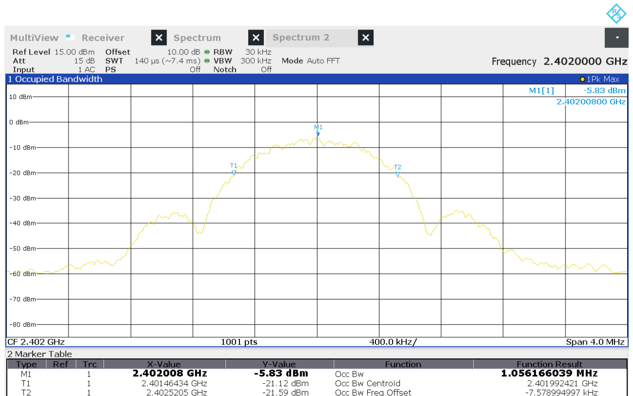
Figure 12: Chart of occupied bandwidth test on lowest channel
