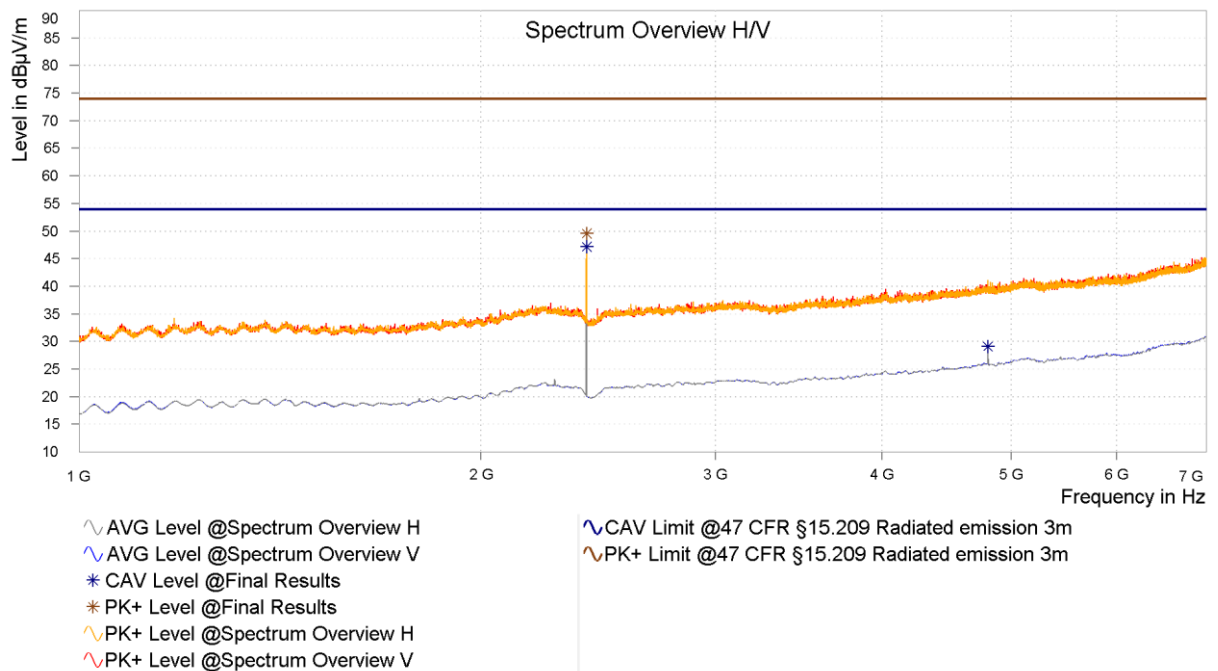
Figure 42: Chart of radiated emissions pre-measurement from 1 GHz to 7 GHz on lowest channel, EUT position Y, antenna polarization vertical and horizontal
