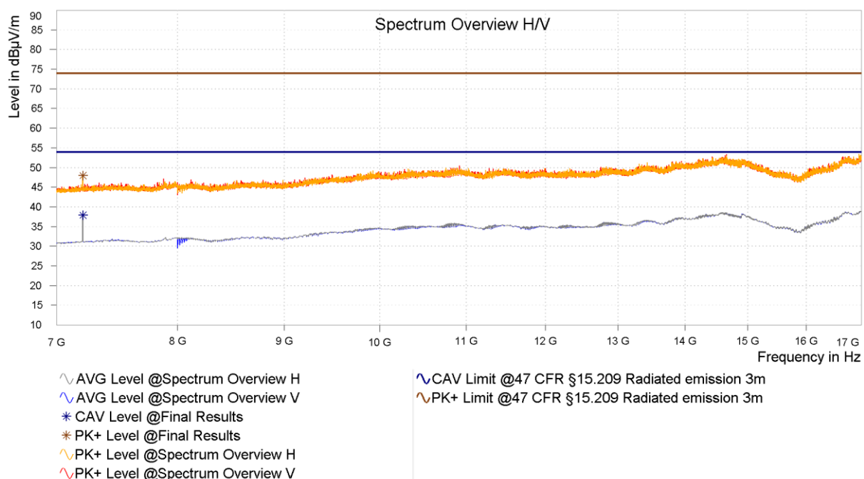
Figure 40: Chart of radiated emissions pre-measurement from 7 GHz to 17 GHz on lowest channel, EUT position Y, antenna polarization vertical and horizontal
