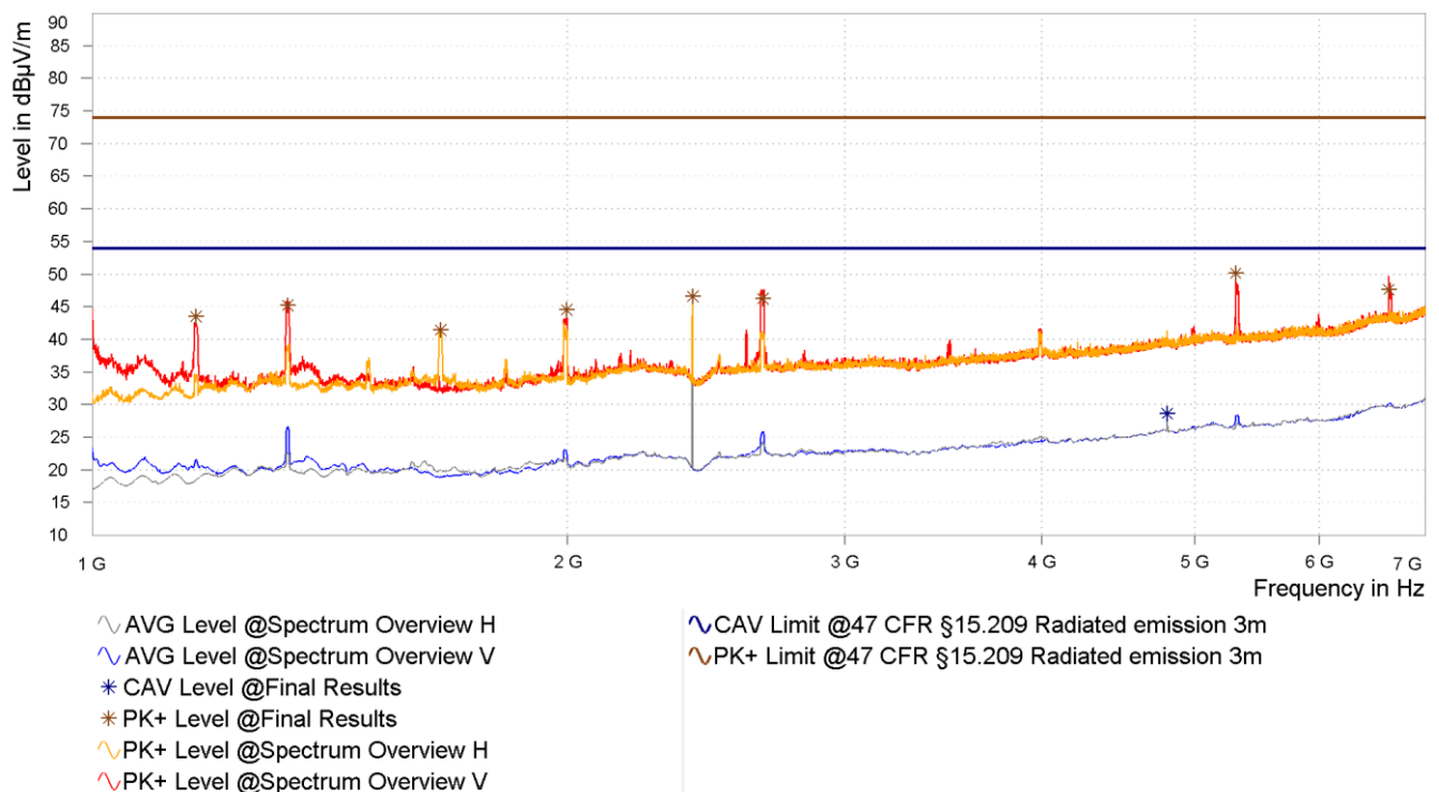
Figure 30: Chart of radiated emissions pre-measurement from 1 GHz to 7 GHz on lowest channel, EUT position Y, antenna polarization horizontal and vertical
