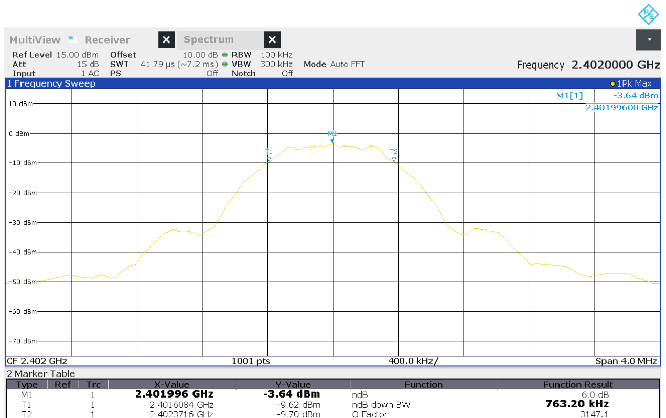
Figure 9: Chart of 6 dB bandwidth test on lowest channel
