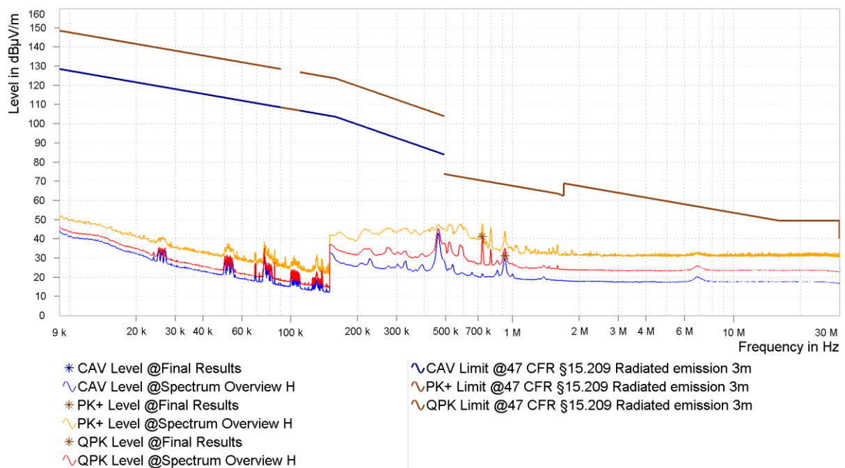
Figure 25: Chart of emissions test below 30 MHz on lowest channel, EUT position Y, antenna parallel
