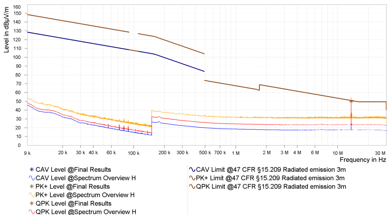
Figure 13: Chart of radiated emissions test below 30 MHz, EUT position Y, antenna polarization in line, without tag
