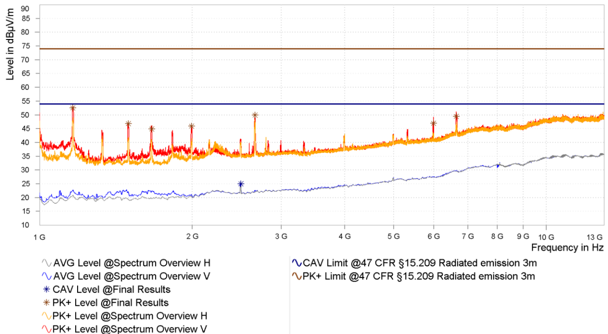
Figure 18: Chart of emissions test from 1 GHz to 13 GHz, EUT position Y, antenna polarization vertical and horizontal, with tag
