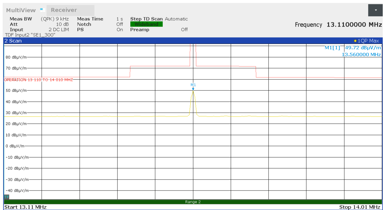
Figure 10: Chart of emission within the band 13.110 MHz to 14.010 MHz, EUT in position Y, without tag, antenna in line at 3 m distance
