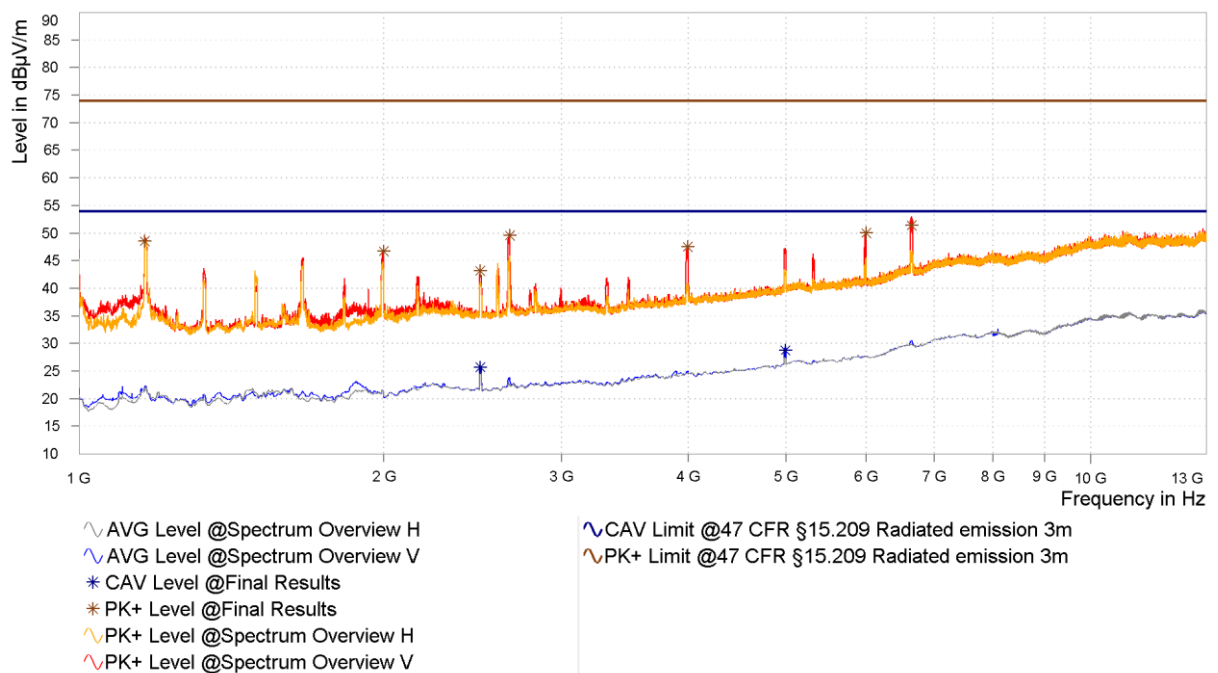
Figure 17: Chart of emissions test from 1 GHz to 13 GHz, EUT position Y, antenna polarization vertical and horizontal, with tag
