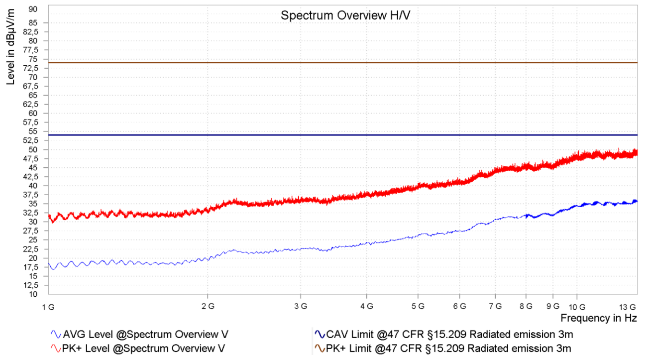
Figure 19: Chart of emissions test from 1 GHz to 13 GHz, EUT position Y, antenna polarization vertical, without tag
