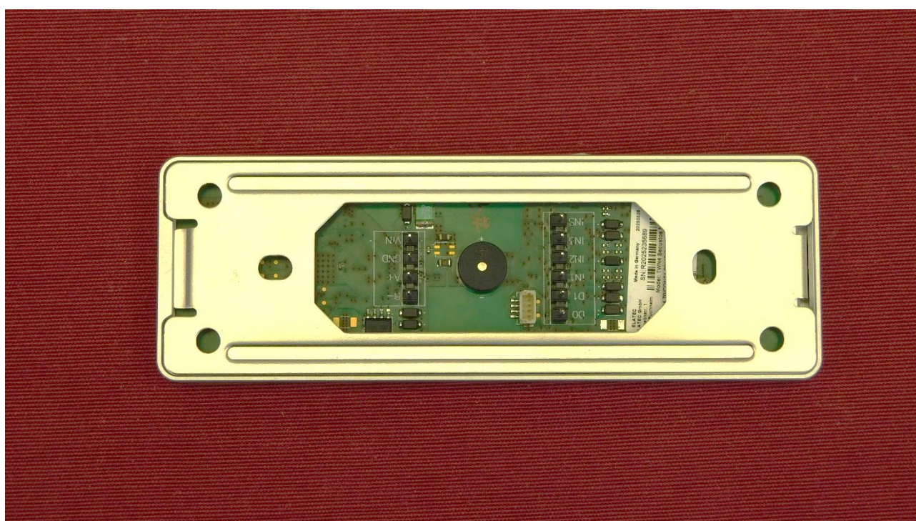
Picture 2: EUT – rear view with metallic support
