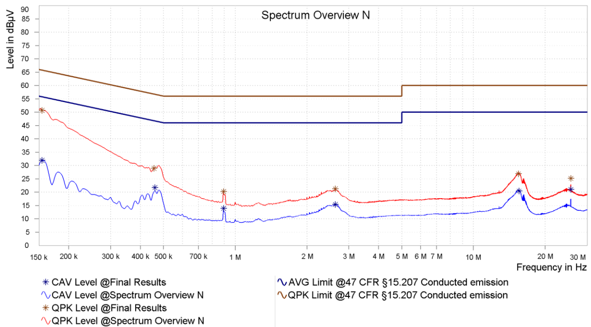
Figure 6: Chart of AC powerline conducted emissions on N
