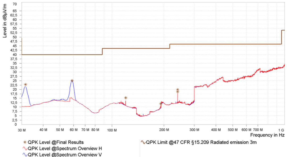
Figure 13: Chart of radiated emissions test from 30 MHz to 1 GHz, EUT position Y, with tag, antenna horizontal and vertical
