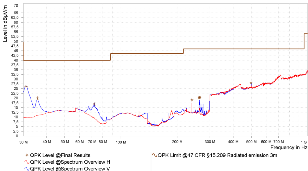
Figure 12: Chart of radiated emissions test from 30 MHz to 1 GHz, EUT position Y, with tag, antenna horizontal and vertical
