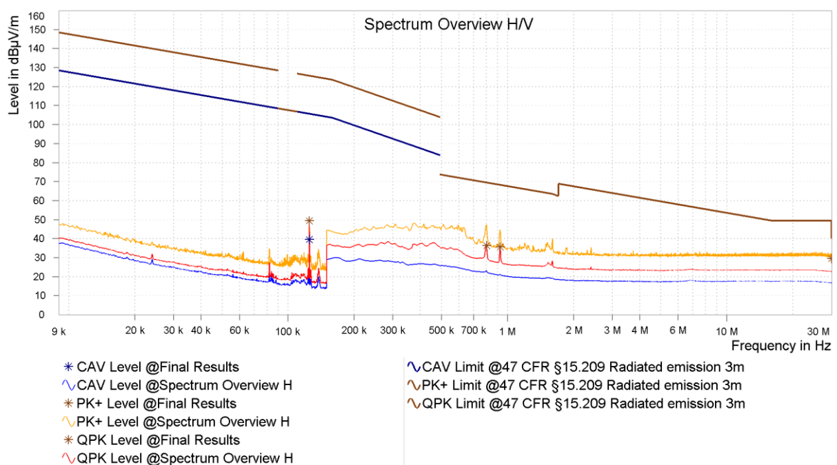
Figure 8: Chart of radiated emissions test below 30 MHz, EUT position Y, antenna polarization parallel, with tag
