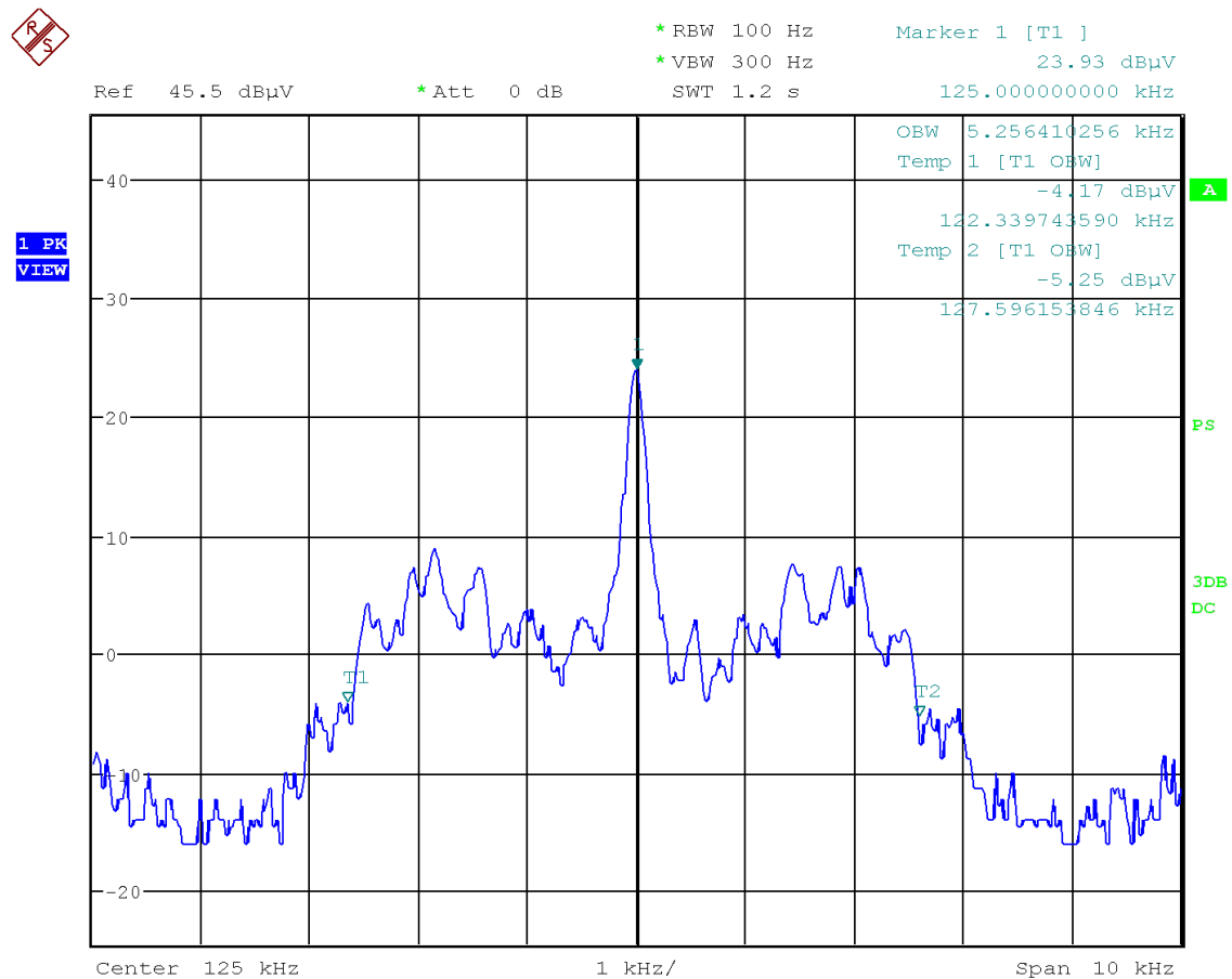
Figure 7: Chart of occupied bandwidth test, with tag
