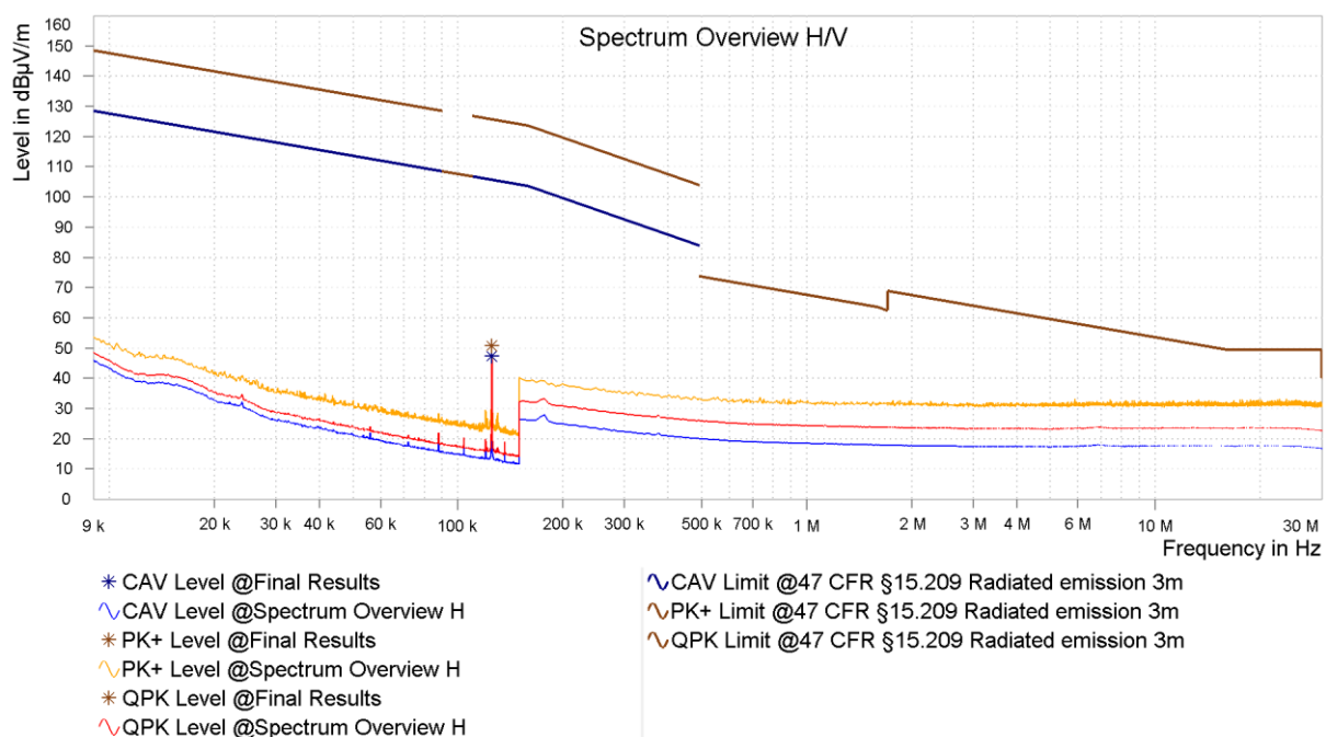
Figure 10: Chart of radiated emissions test below 30 MHz, EUT position Y, antenna polarization parallel, without tag
