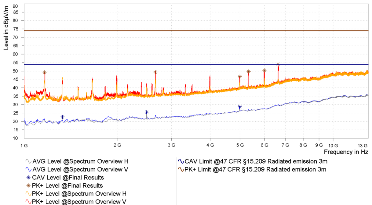
Figure 14: Chart of radiated emissions pre-measurement from 1 GHz to 13 GHz, EUT position Y, with tag, antenna polarization horizontal and vertical
