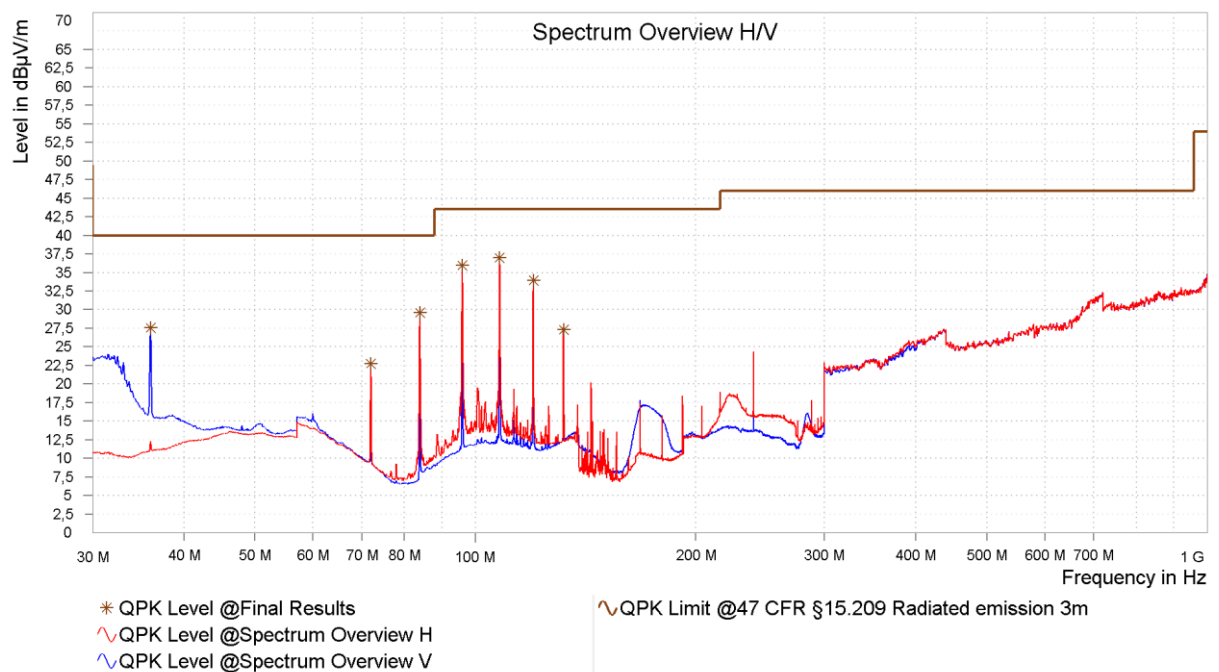
Figure 11: Chart of radiated emissions test from 30 MHz to 1 GHz, EUT position X, with tag, antenna horizontal and vertical
