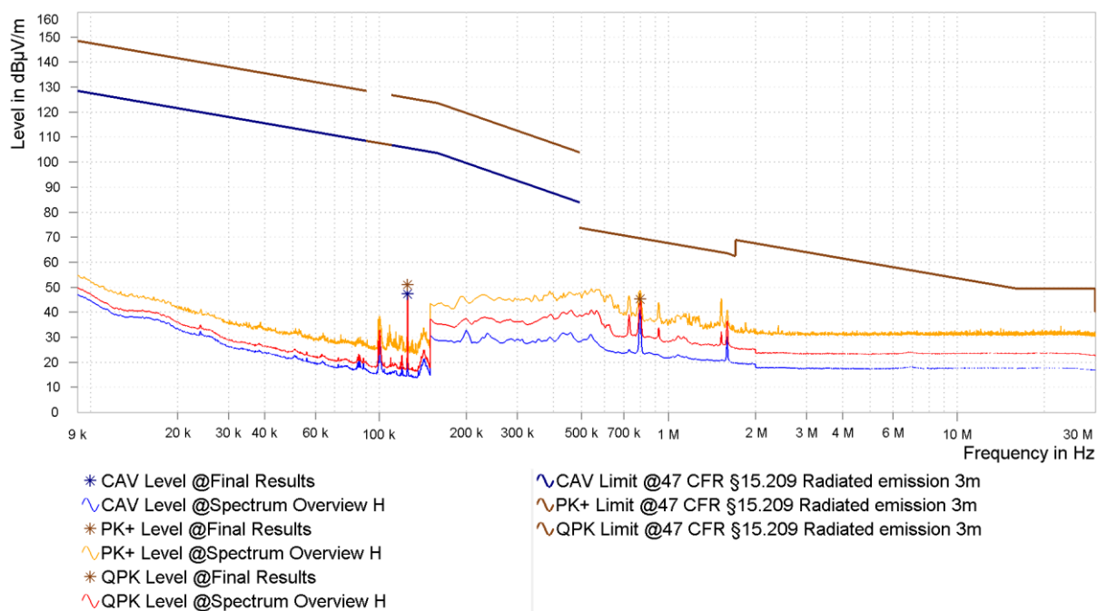
Figure 9: Chart of radiated emissions test below 30 MHz, EUT position Y, antenna polarization parallel, without tag
