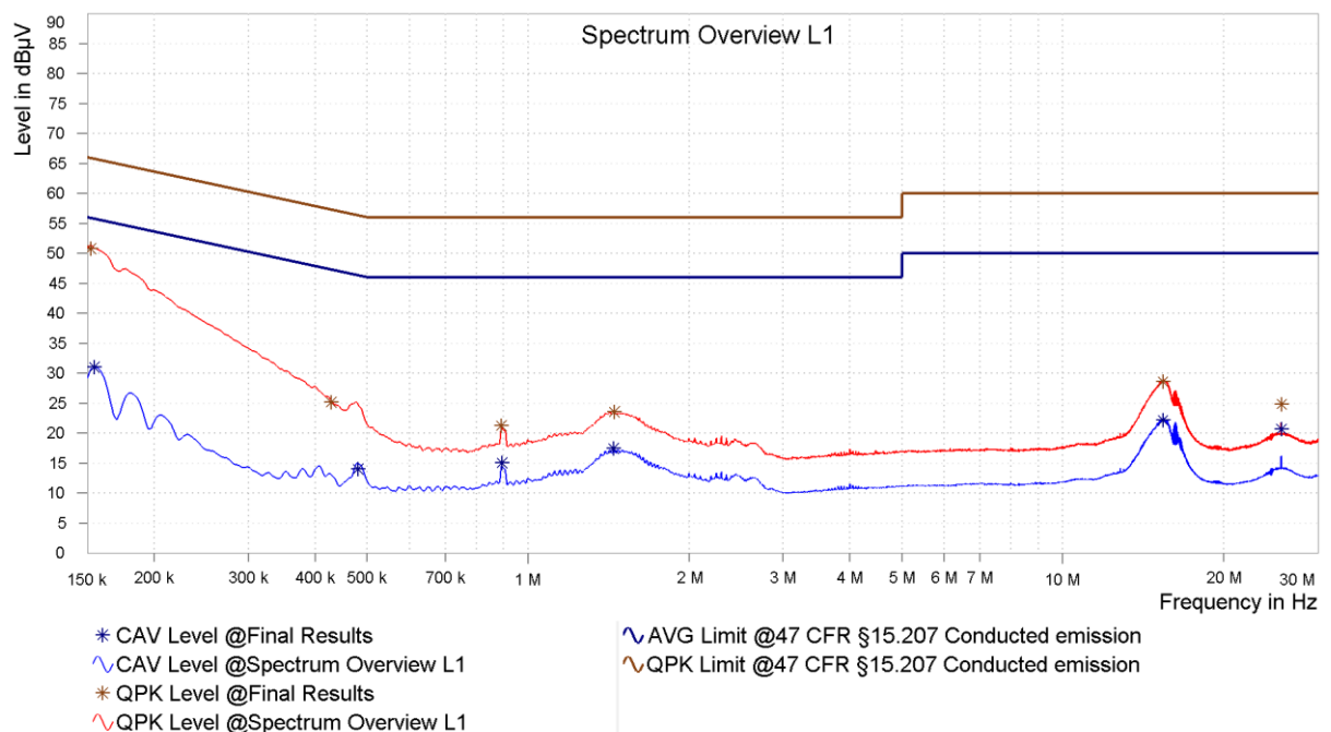
Figure 5: Chart of AC powerline conducted emissions on L1
