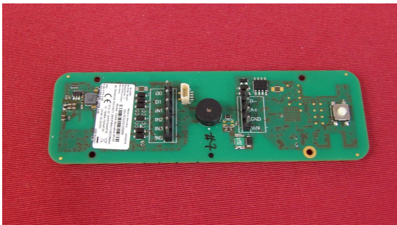
Picture 2: Opened EUT – bottom side
