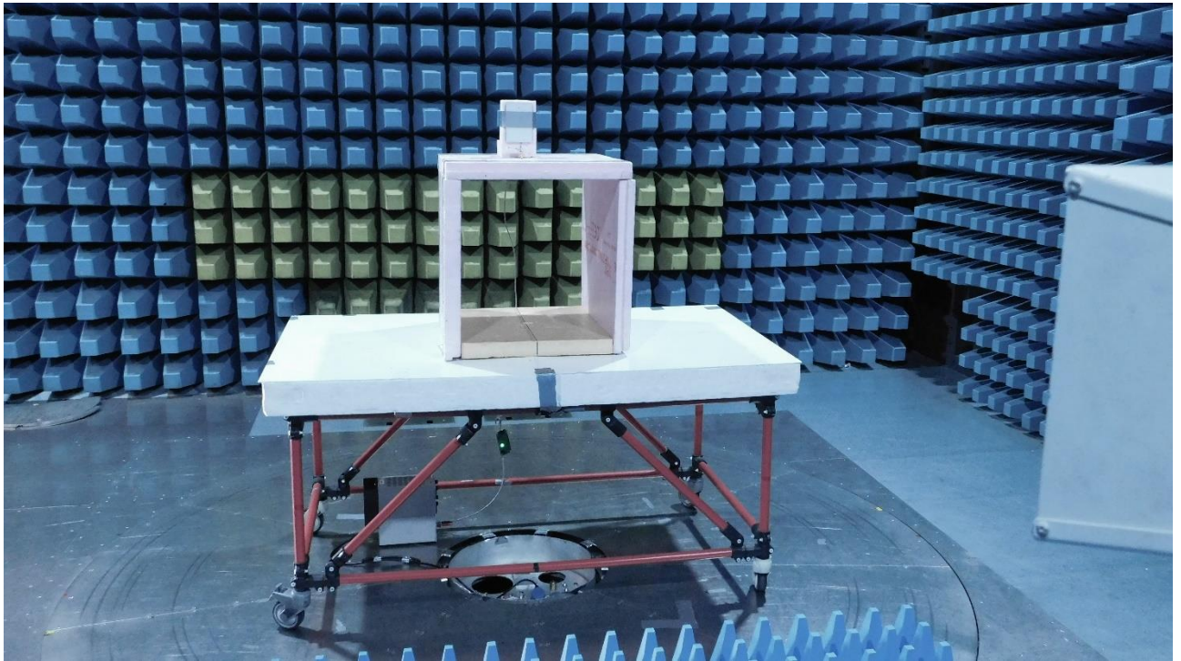
Picture 23: SAC, radiated emission test 1 GHz – 17 GHz (rear view)
