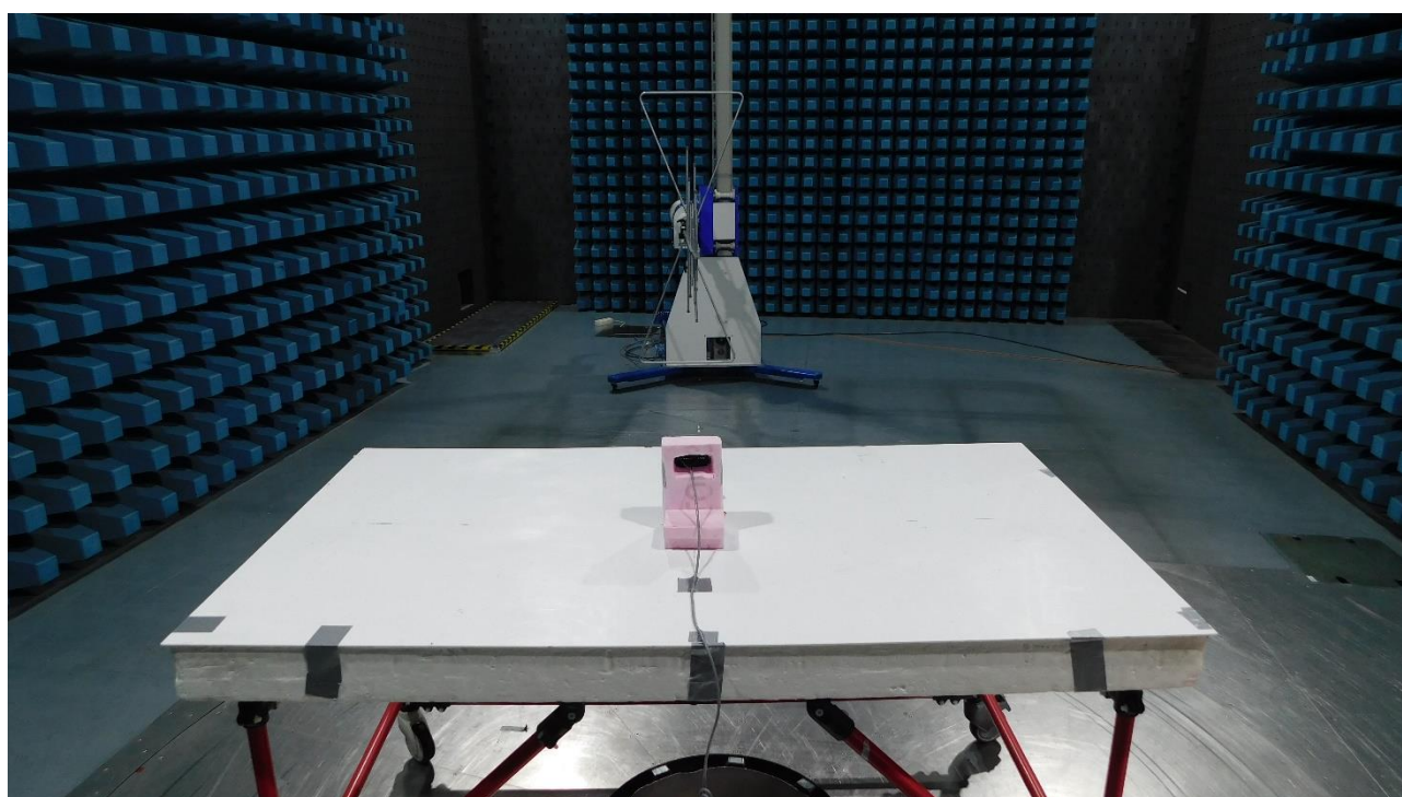
Picture 20: SAC, radiated emission test 30 MHz - 1 GHz (front view)
