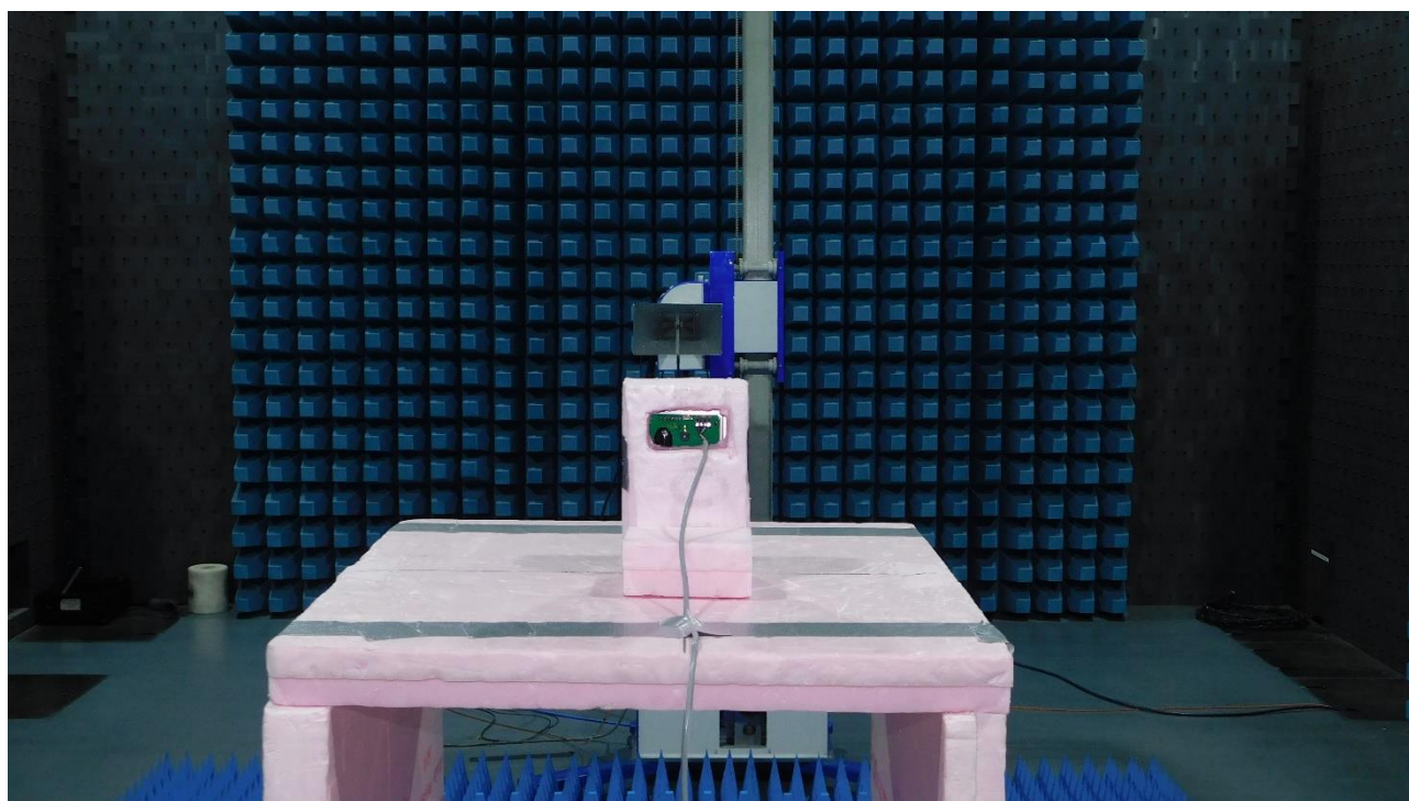
Picture 15: SAC, radiated emission test 1 GHz – 17 GHz (front view)
