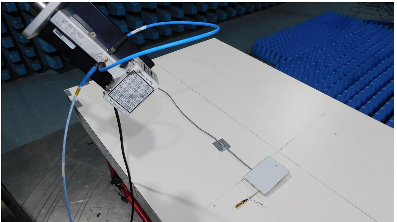
Picture 24: SAC, exploratory radiated emission test 17 GHz – 25 GHz (front view)
