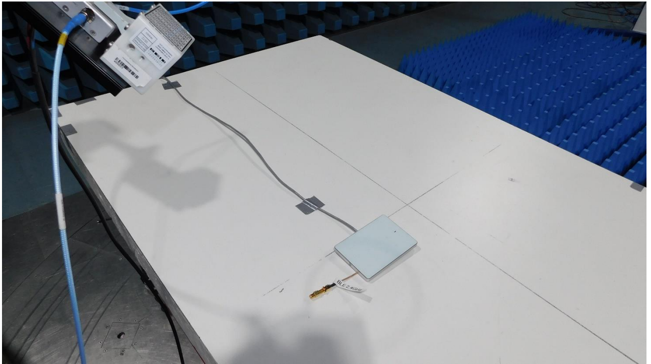
Picture 17: SAC, exploratory radiated emission test 17 GHz – 25 GHz (front view)
