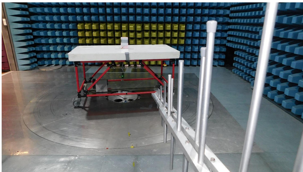
Picture 21: SAC, radiated emission test 30 MHz - 1 GHz (rear view)
