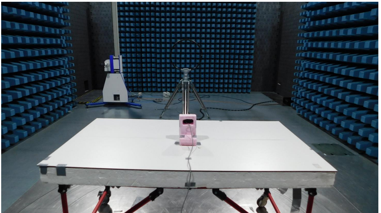
Picture 18: SAC, test setup radiated emission test 9 kHz - 30 MHz (front view)
