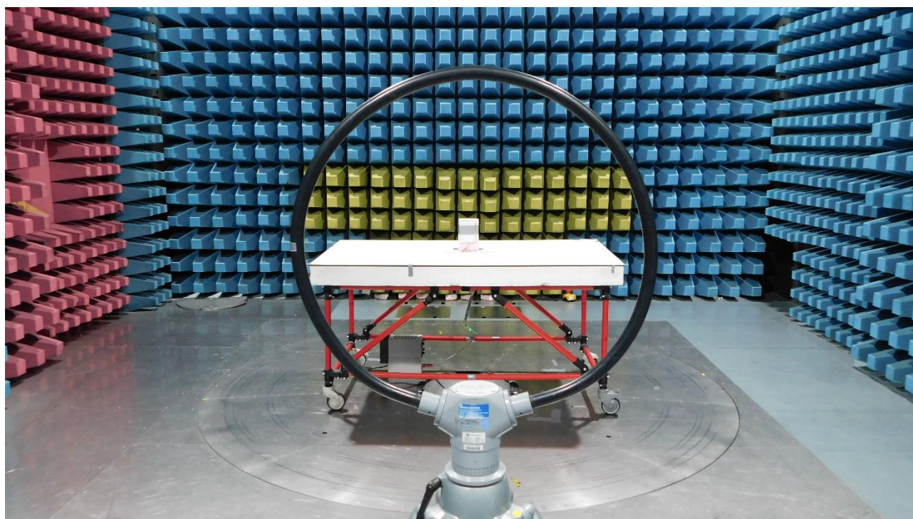
Picture 19: SAC, test setup radiated emission test 9 kHz - 30 MHz (rear view)
