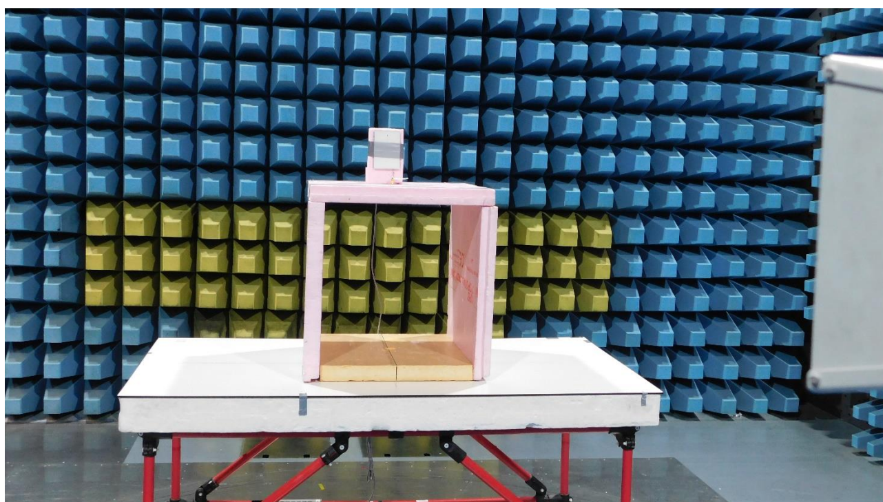
Picture 16: SAC, radiated emission test 1 GHz – 17 GHz (rear view)
