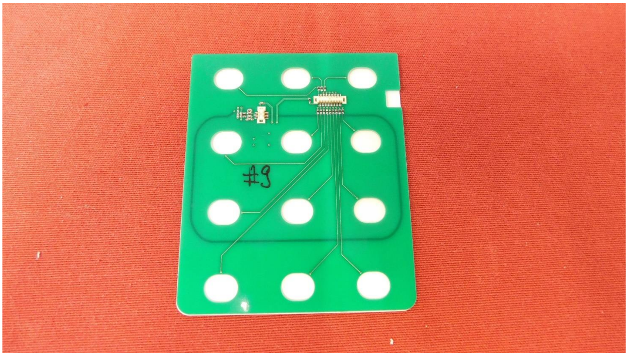
Picture 5: Touch PCB – bottom side
