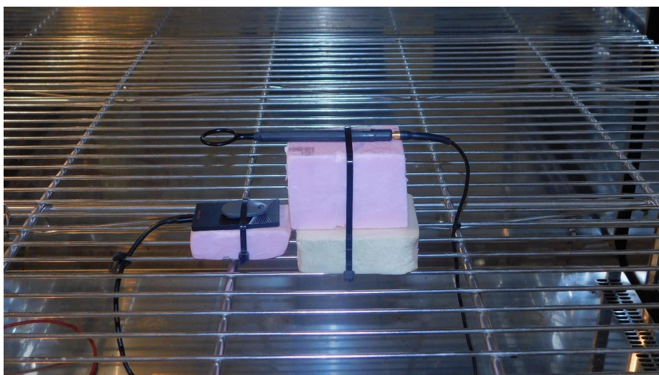
Picture 10: Test setup-Carrier frequency stability test
