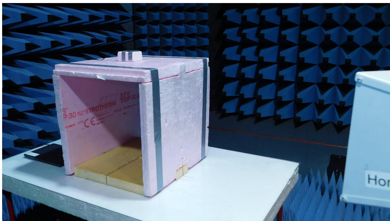
Picture 5: FS-SAC, radiated emission test 1 GHz – 12.5 GHz (front view)
