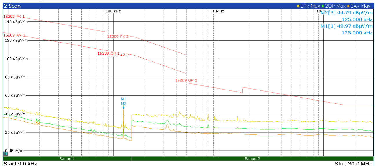
Figure 8: Chart of radiated emissions test below 30 MHz, EUT position Z, antenna polarization parallel, without tag
