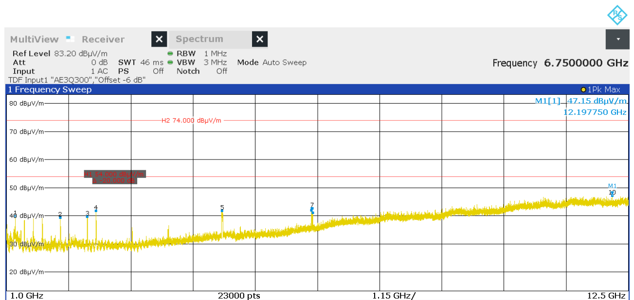
Figure 10: Chart of radiated emissions pre-measurement from 1 GHz to 12.5 GHz, EUT position Z, with tag, antenna polarization vertical
