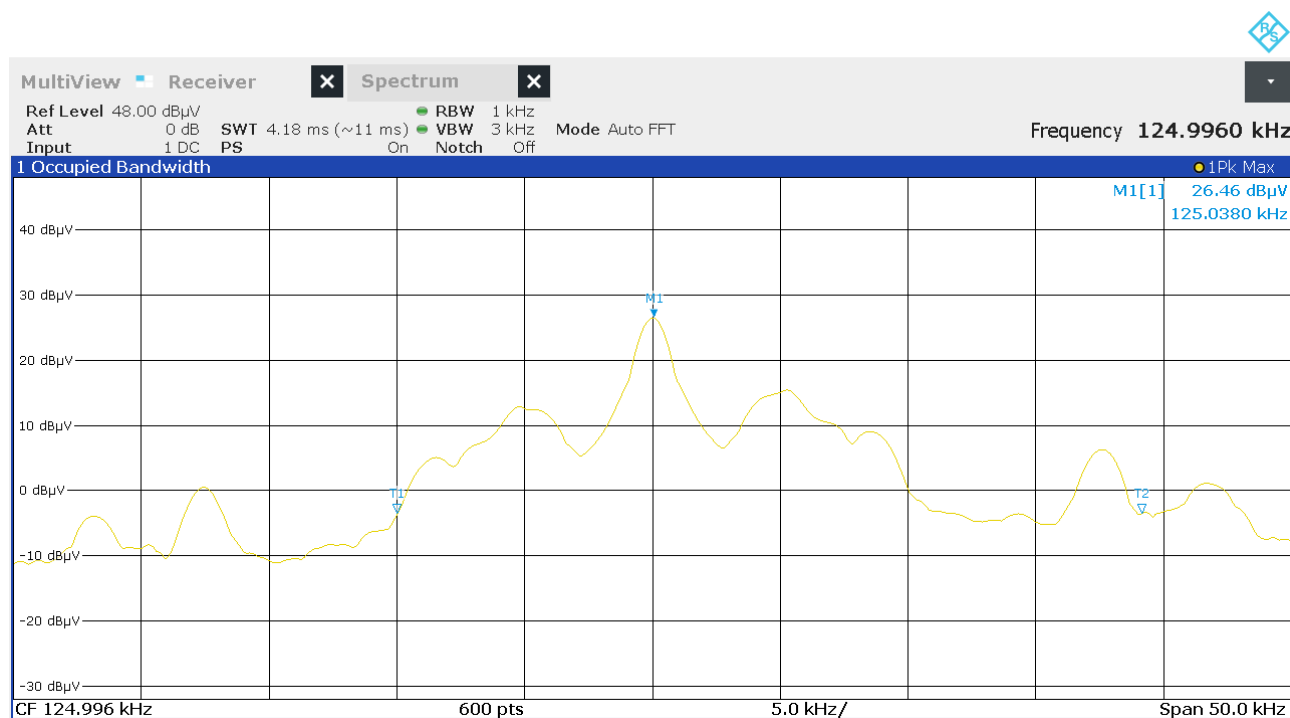
Figure 7: Chart of occupied bandwidth test, without tag
