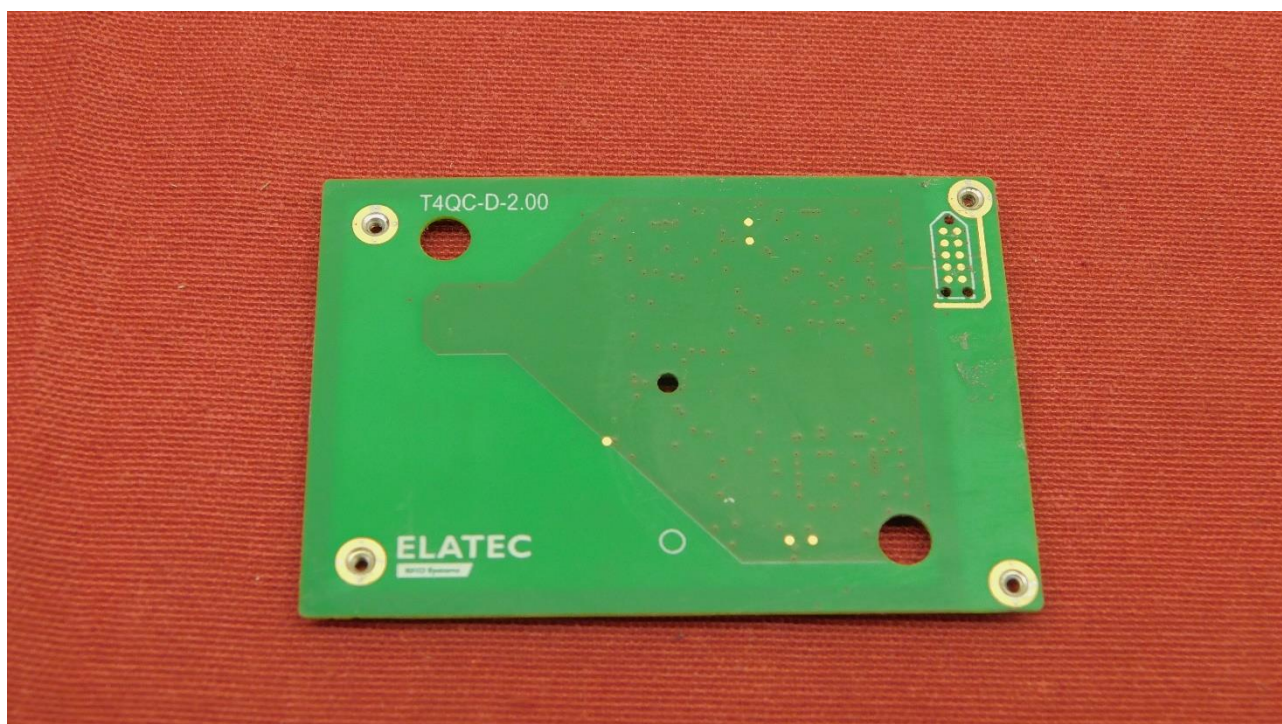
Picture 2: PCB of EUT - bottom side
