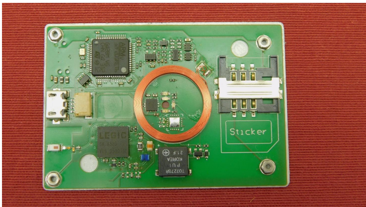
Picture 1: PCB of EUT - top side
