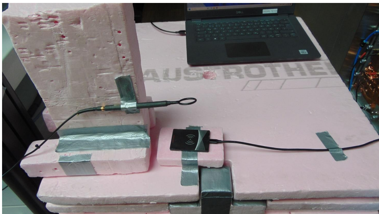
Picture 9: Test setup occupied bandwidth test
