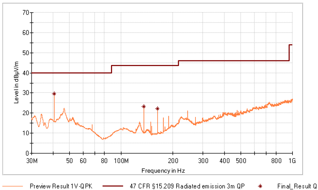
Figure 12: Chart of radiated emissions test from 30 MHz to 1 GHz, EUT position Y, antenna polarization vertical, without tag
