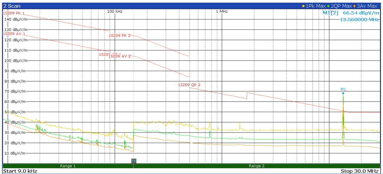
Figure 11: Chart of radiated emissions test below 30 MHz, EUT position Z, antenna polarization in line, without tag
