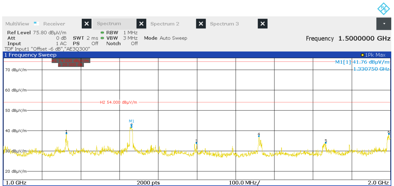
Figure 13: Chart of emissions test from 1 GHz to 2 GHz, EUT position Z, antenna polarization horizontal, with tag
