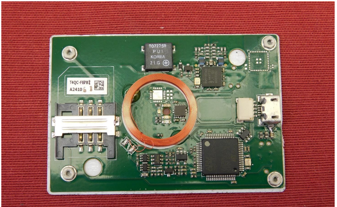
Picture 1: PCB - top side
