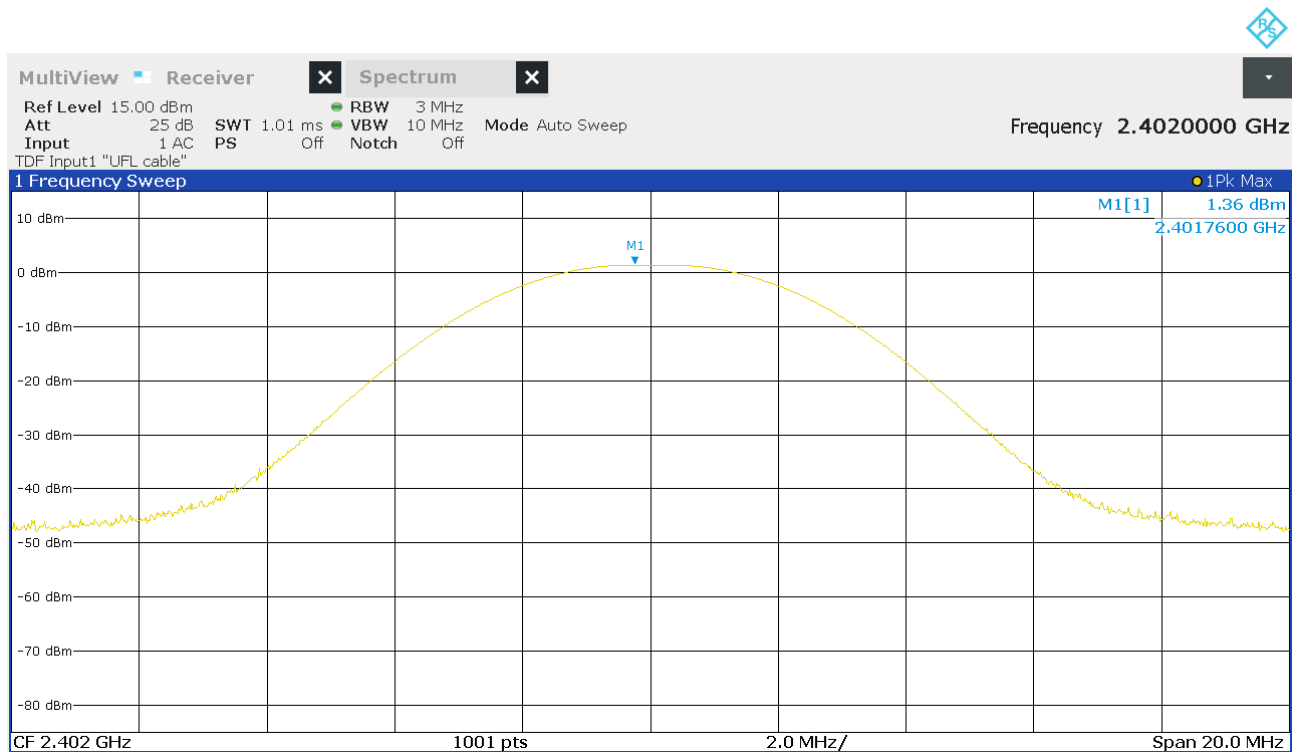
Figure 16: Chart of conducted output power on lowest channel
