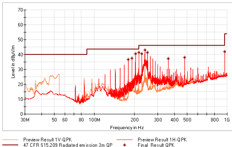
Figure 35: Chart of radiated emissions test from 30 MHz to 1 GHz on lowest channel, EUT position X, antenna polarization vertical and horizontal
