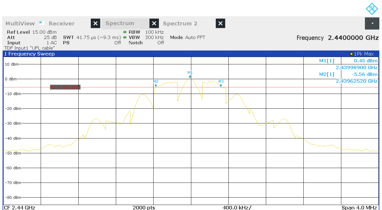
Figure 9: Chart of 6 dB bandwidth test on middle channel
