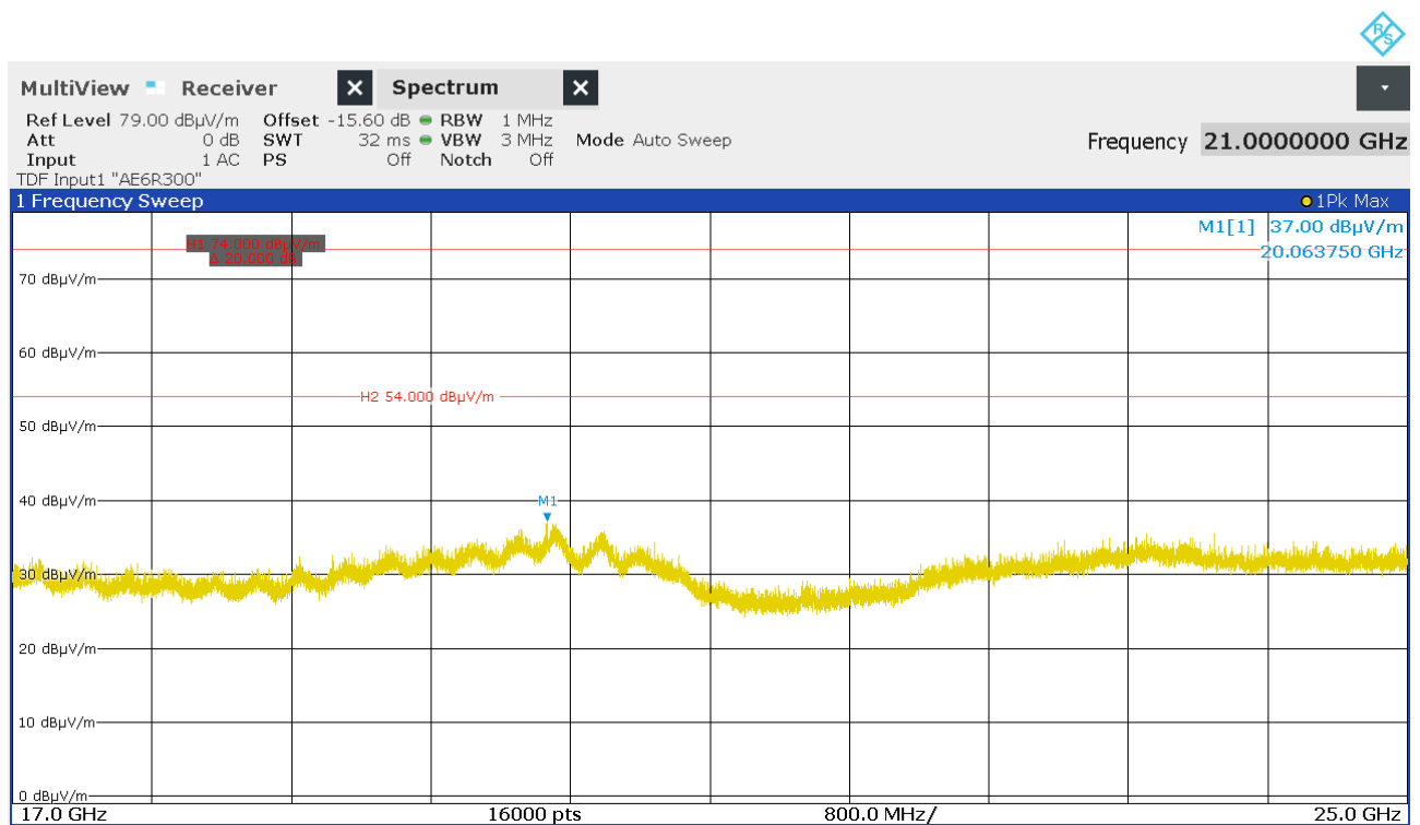
Figure 39: Chart of exploratory emission test from 17 GHz to 25 GHz on middle channel at 0.5 m, EUT position X, antenna polarization vertical and horizontal
