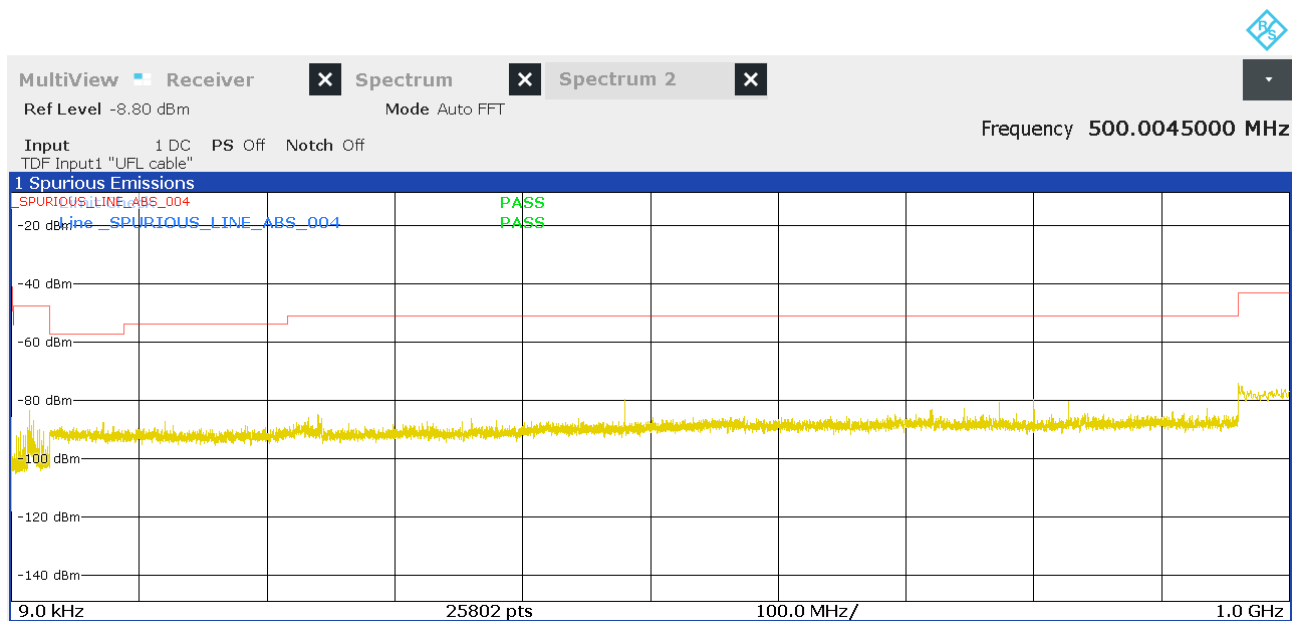
Figure 25: Chart of emissions test from 9 kHz to 1 GHz on lowest channel, Pk
