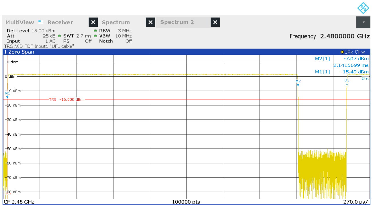
Figure 15: Chart of the duty cycle measurement in a time interval of 2.7 ms on the highest channel
