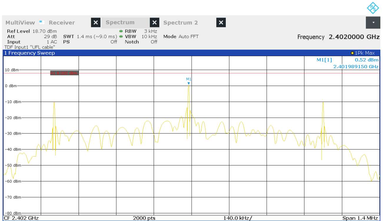
Figure 19: Chart of power spectral density on lowest channel
