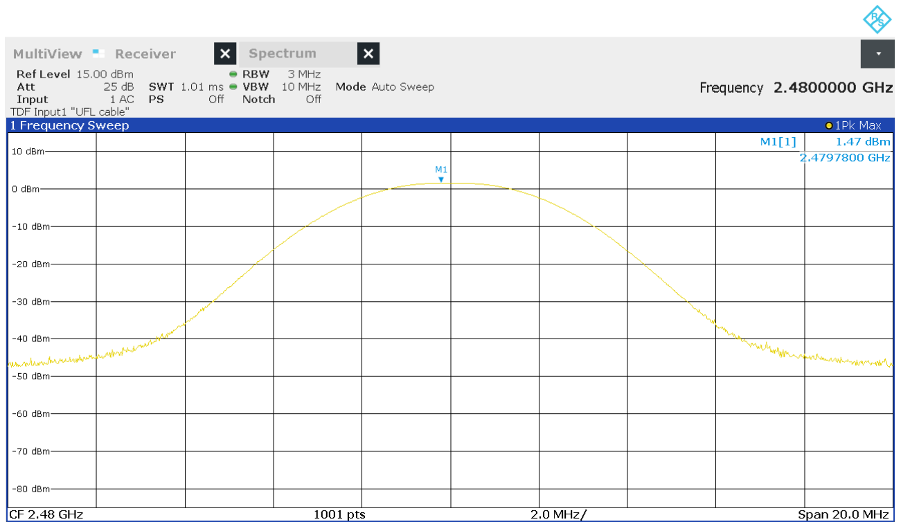
Figure 18: Chart of conducted output power on highest channel
