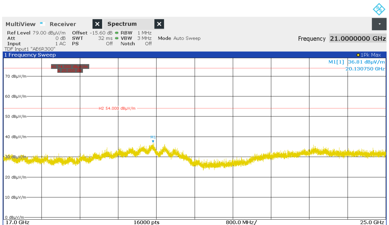
Figure 41: Chart of exploratory emission test from 17 GHz to 25 GHz on highest channel at 0.5 m, EUT position X, antenna polarization vertical and horizontal
