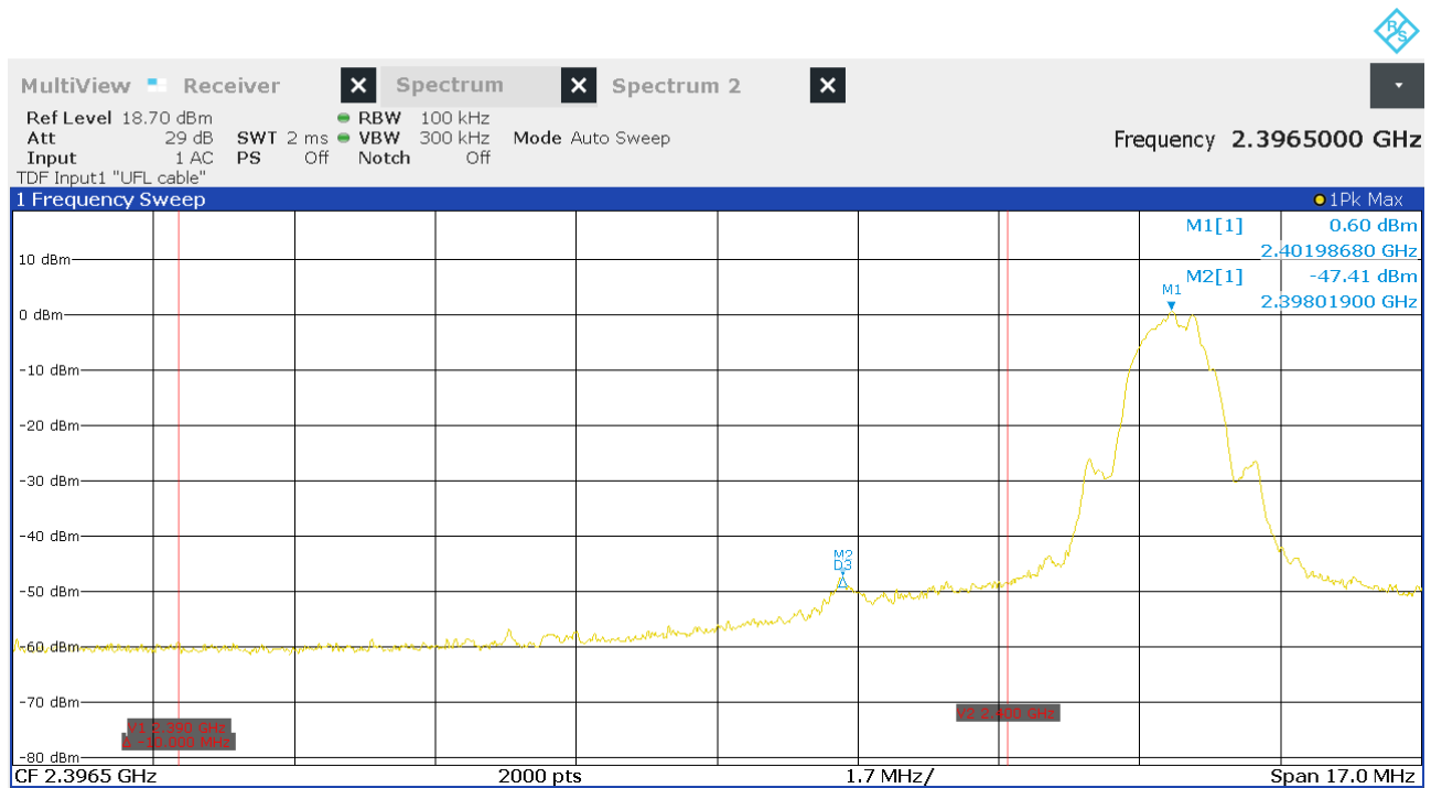
Figure 22: Chart of lower band-edge measurement on lowest channel
