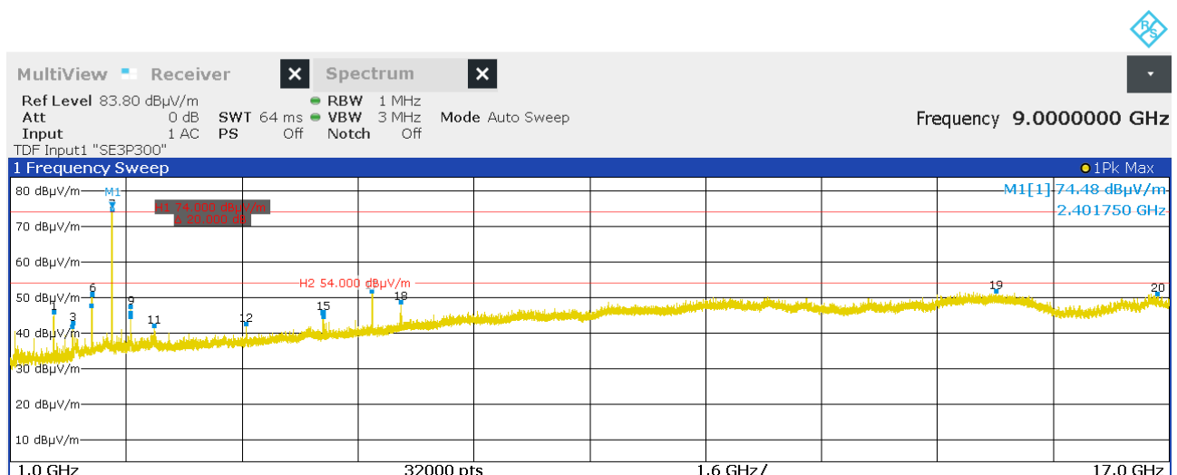
Figure 36: Chart of radiated emissions pre-measurement from 1 GHz to 17 GHz on lowest channel, EUT position X, antenna polarization vertical
