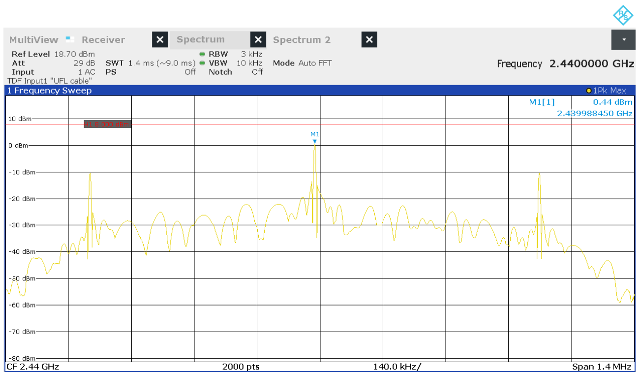
Figure 20: Chart of power spectral density on middle channel
