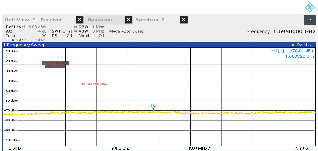
Figure 32: Chart of emissions test from 1 GHz to 2.39 GHz on highest channel, Pk
