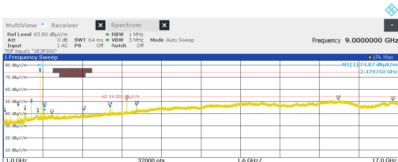
Figure 40: Chart of emissions test from 1 GHz to 17 GHz on highest channel, EUT position X, antenna polarization vertical
