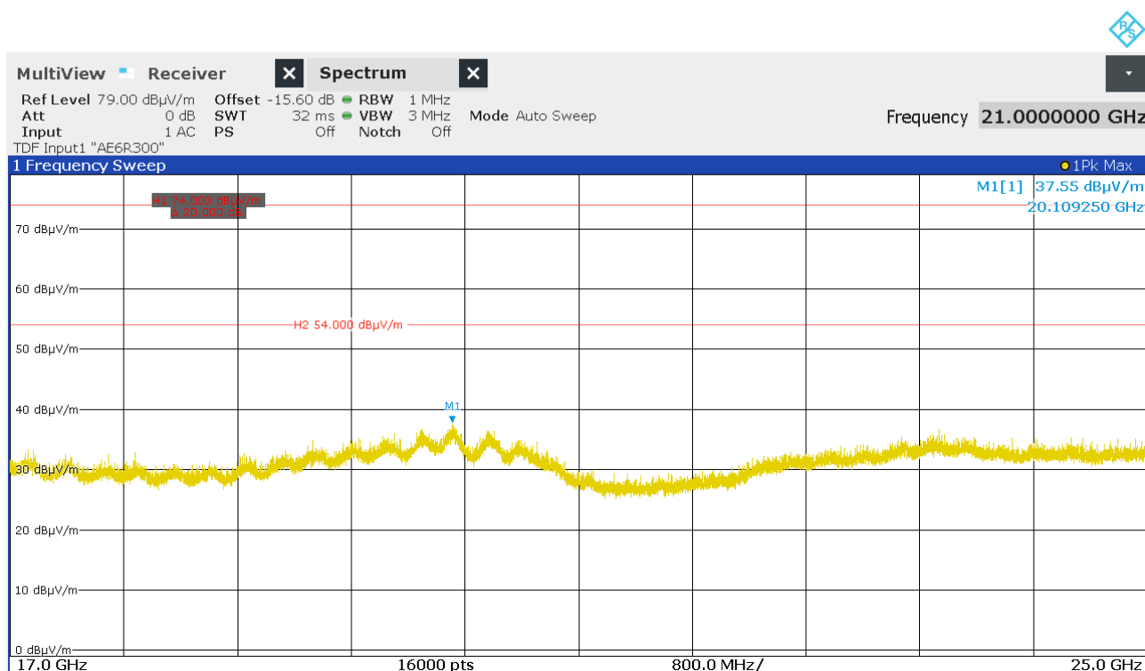
Figure 37: Chart of exploratory emission test from 17 GHz to 25 GHz on lowest channel at 0.5 m, EUT position X, antenna polarization vertical and horizontal
