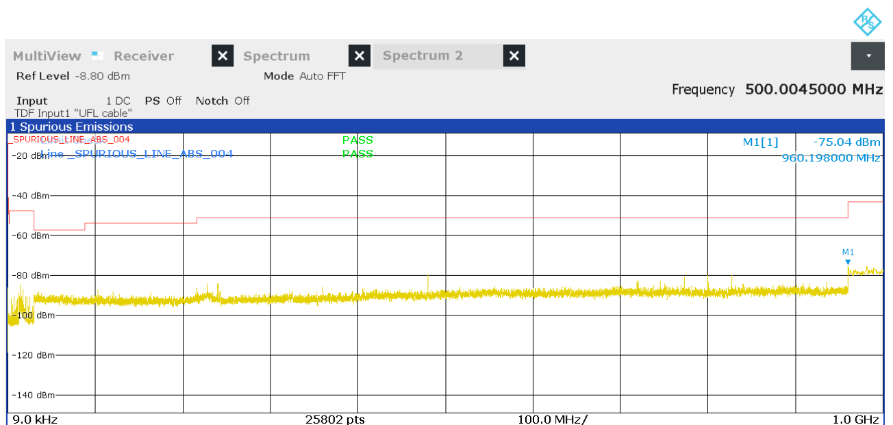
Figure 31: Chart of emissions test from 9 kHz to 1 GHz on highest channel, Pk
