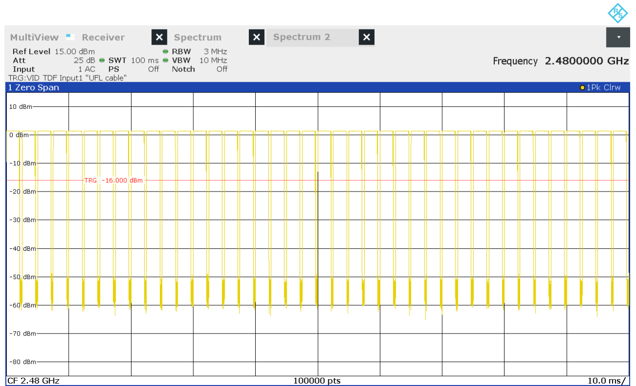
Figure 14: Chart of the duty cycle measurement in a time interval of 100 ms on the highest channel
