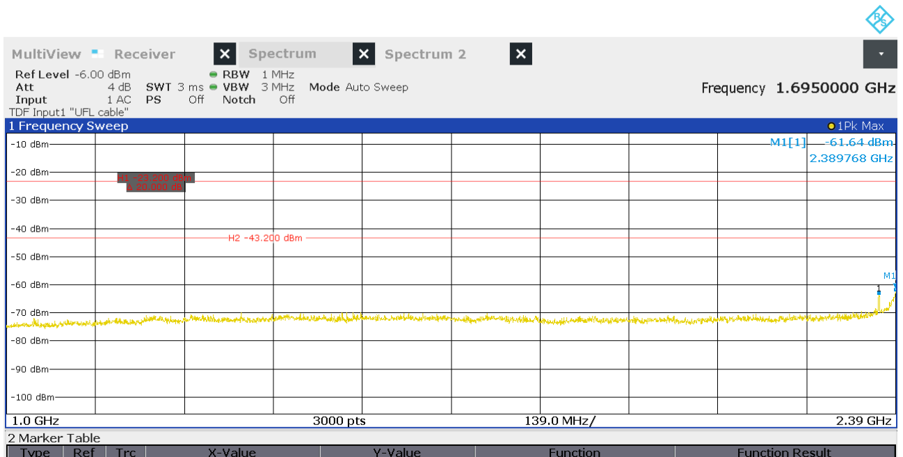
Figure 26: Chart of emissions test from 1 GHz to 2.39 GHz on lowest channel, Pk
