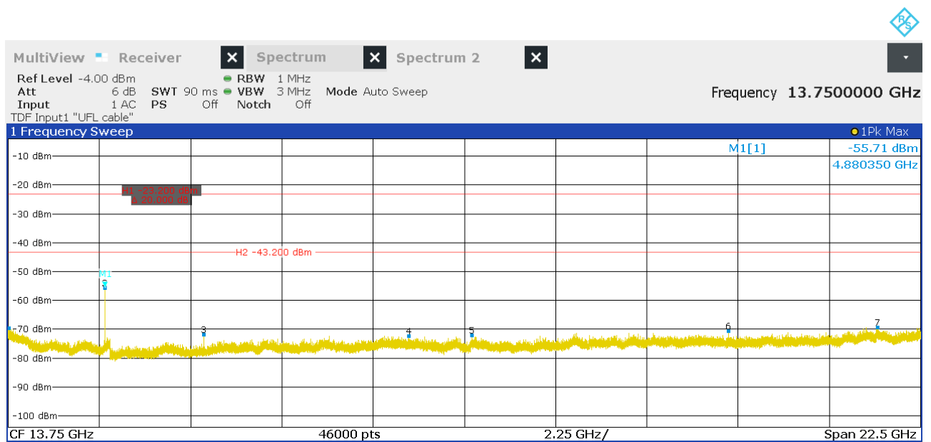
Figure 30: Chart of emissions test from 2.5 GHz to 25 GHz on middle channel, Pk
