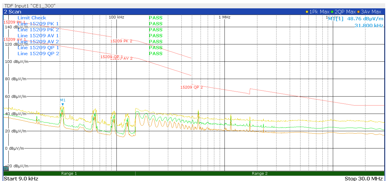
Figure 34: Chart of emissions test below 30 MHz on lowest channel, EUT position X, antenna parallel
