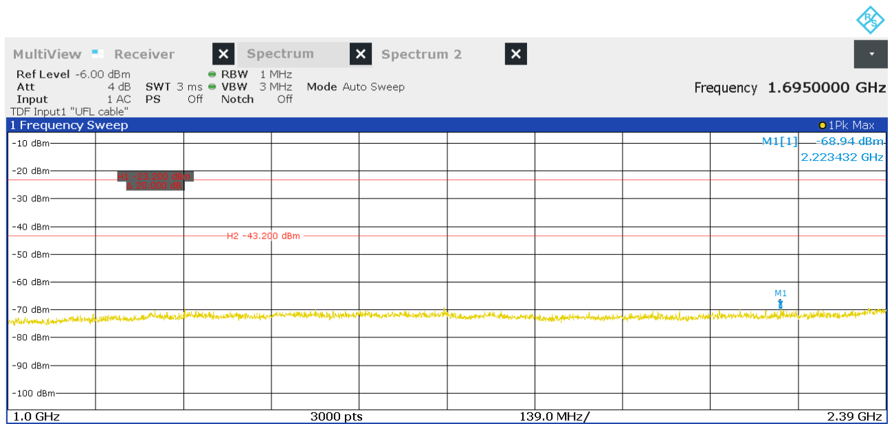
Figure 29: Chart of emissions test from 1 GHz to 2.39 GHz on middle channel, Pk
