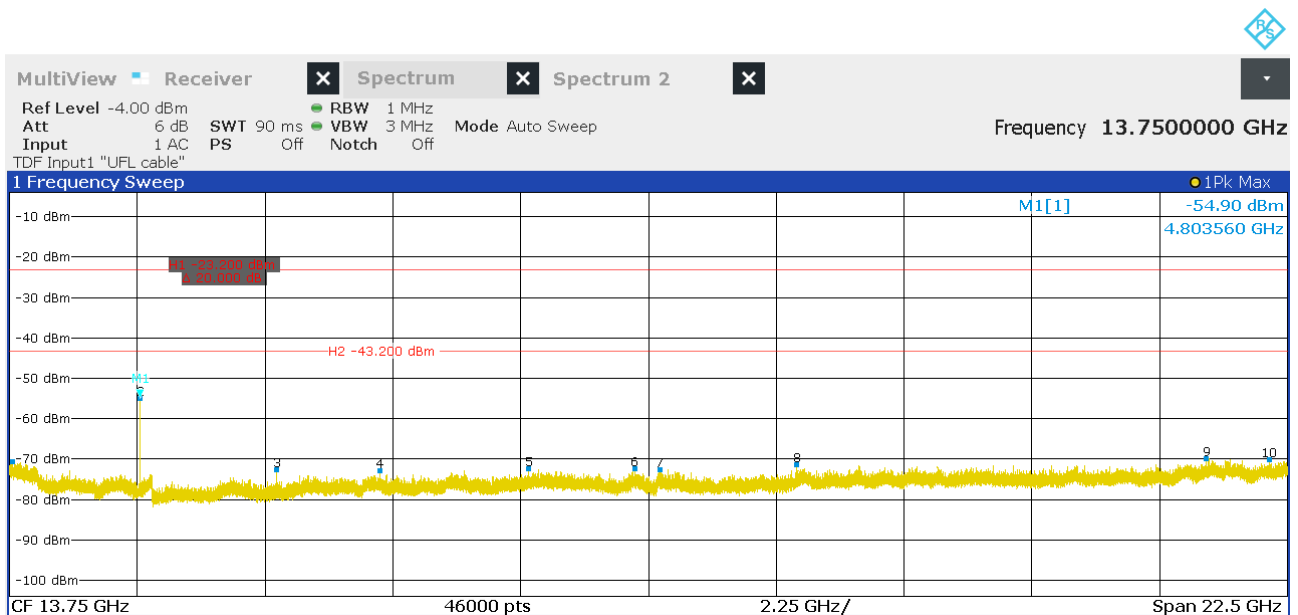
Figure 27: Chart of emissions test from 2.5 GHz to 25 GHz on lowest channel, Pk
