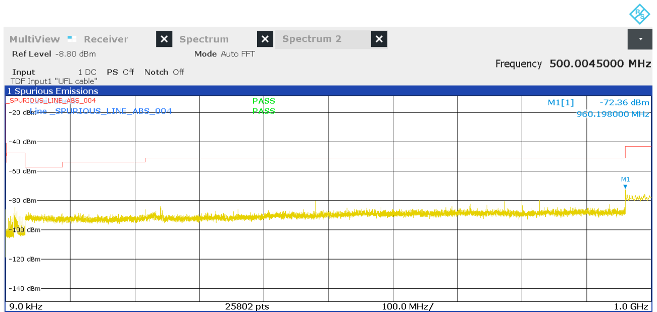
Figure 28: Chart of emissions test from 9 kHz to 1 GHz on middle channel, Pk
