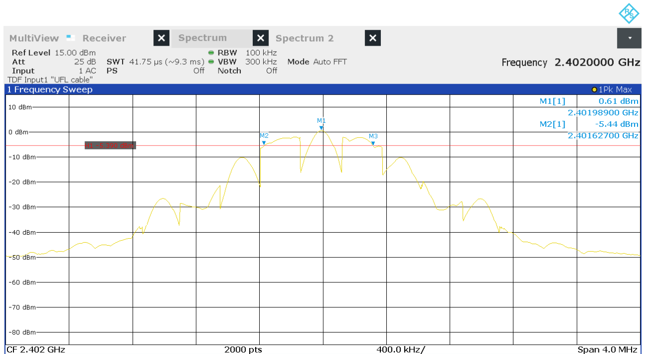
Figure 8: Chart of 6 dB bandwidth test on lowest channel
