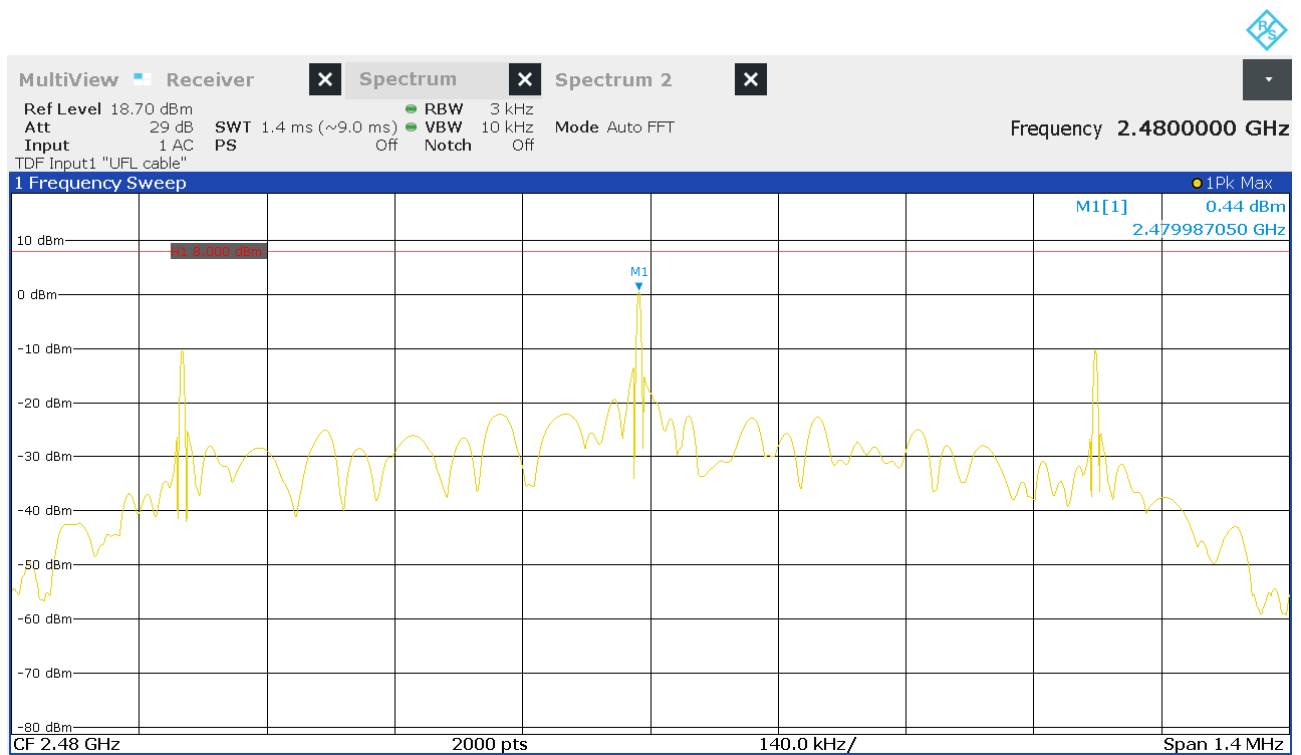
Figure 21: Chart of power spectral density on highest channel
