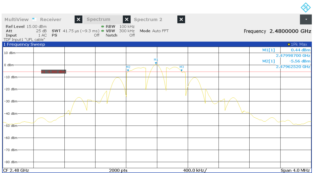
Figure 10: Chart of 6 dB bandwidth test on highest channel
