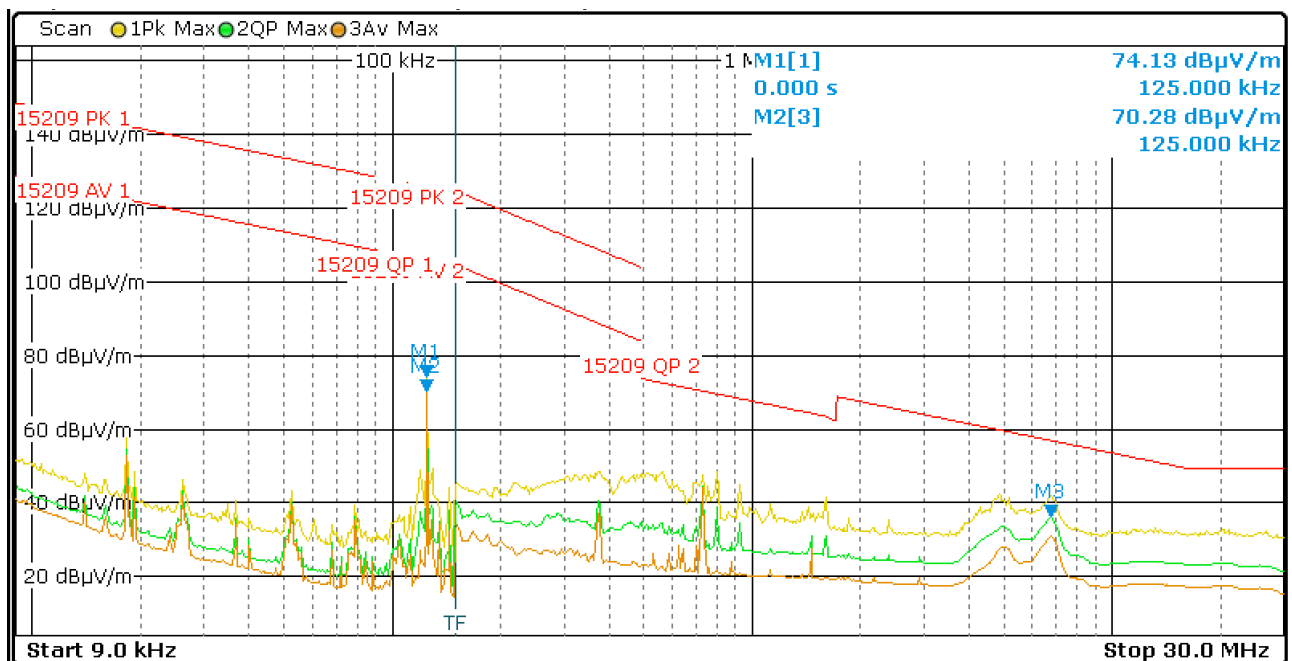
Figure 11: Chart of radiated emissions test below 30 MHz, EUT position X, without tag, antenna parallel
