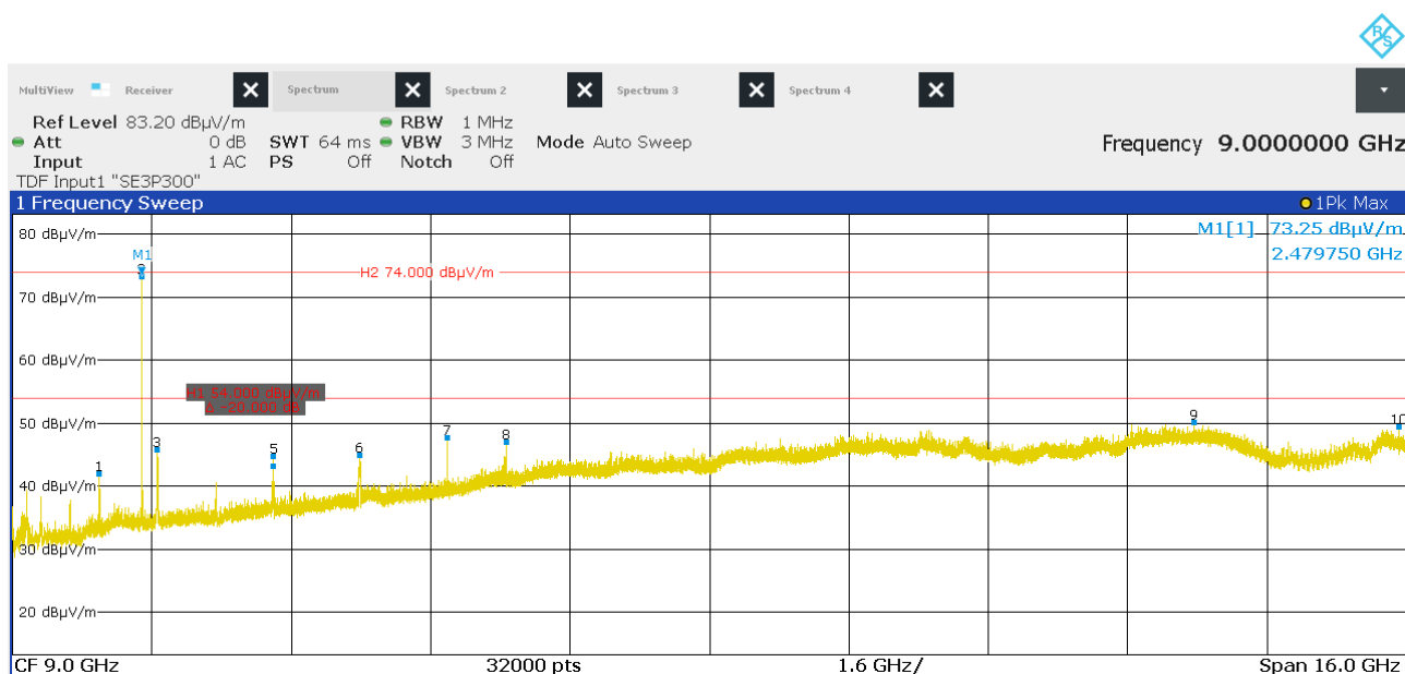
Figure 13: Chart of radiated emissions pre-measurement from 1 GHz to 17 GHz on highest channel, EUT position X, antenna polarization vertical, with tag
