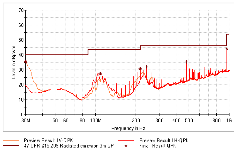
Figure 12: Chart of radiated emissions test from 30 MHz to 1 GHz, EUT position X, without tag, antenna horizontal and vertical
