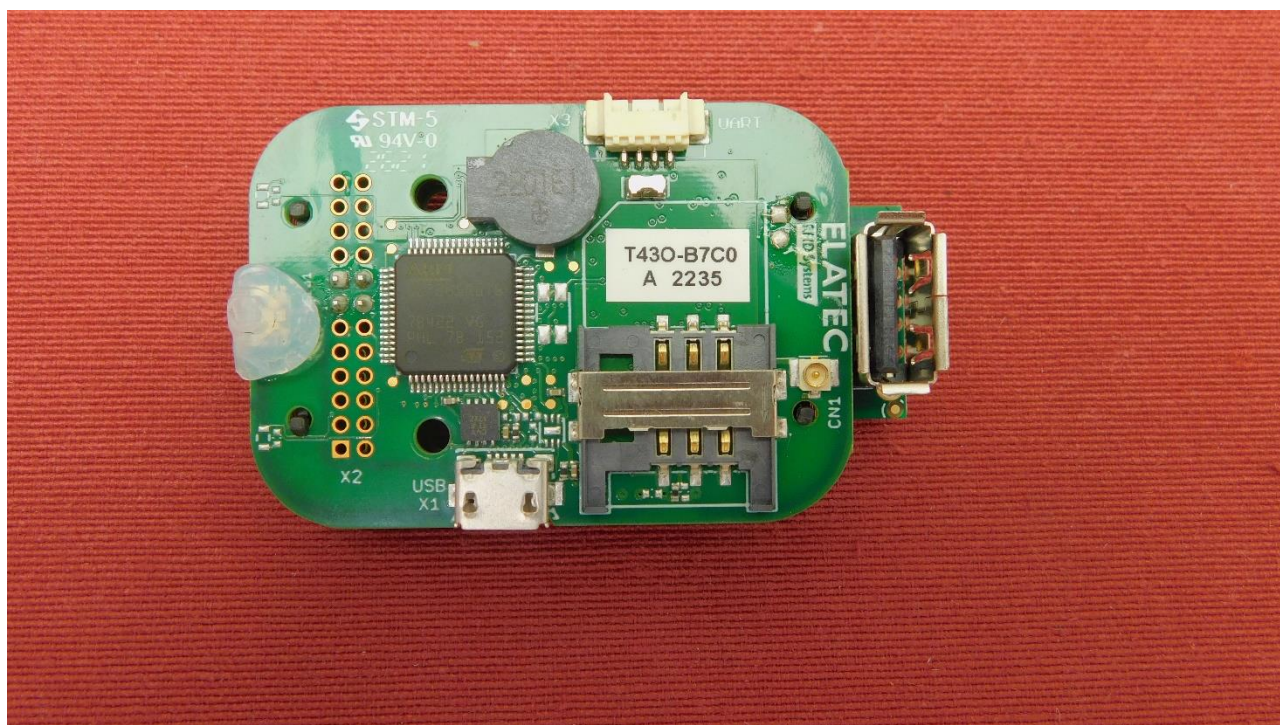
Picture 1: PCB 1 of EUT - top view
