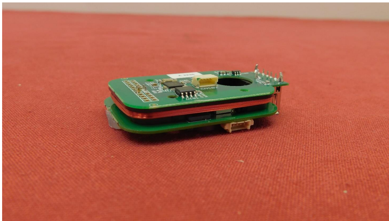
Picture 3: PCB 1 and 2 of EUT – side view
