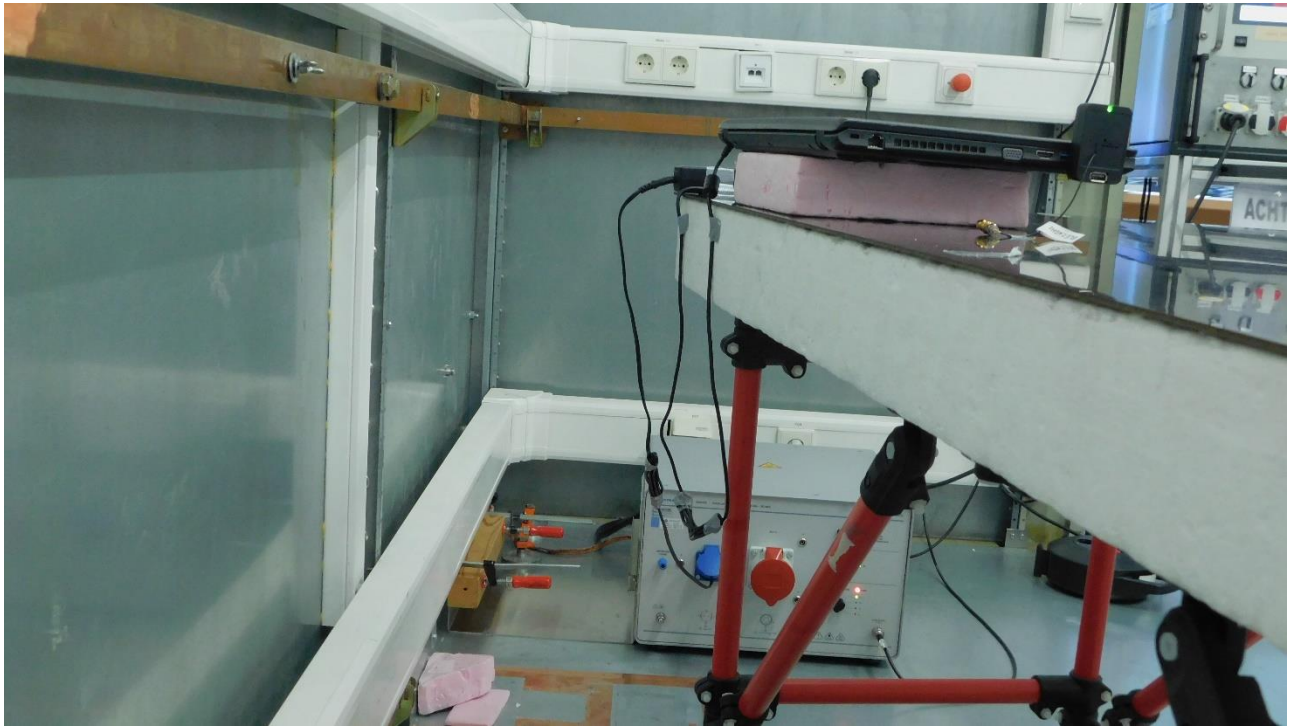
Picture 9: Test setup AC power line conducted emissions (rear view)
