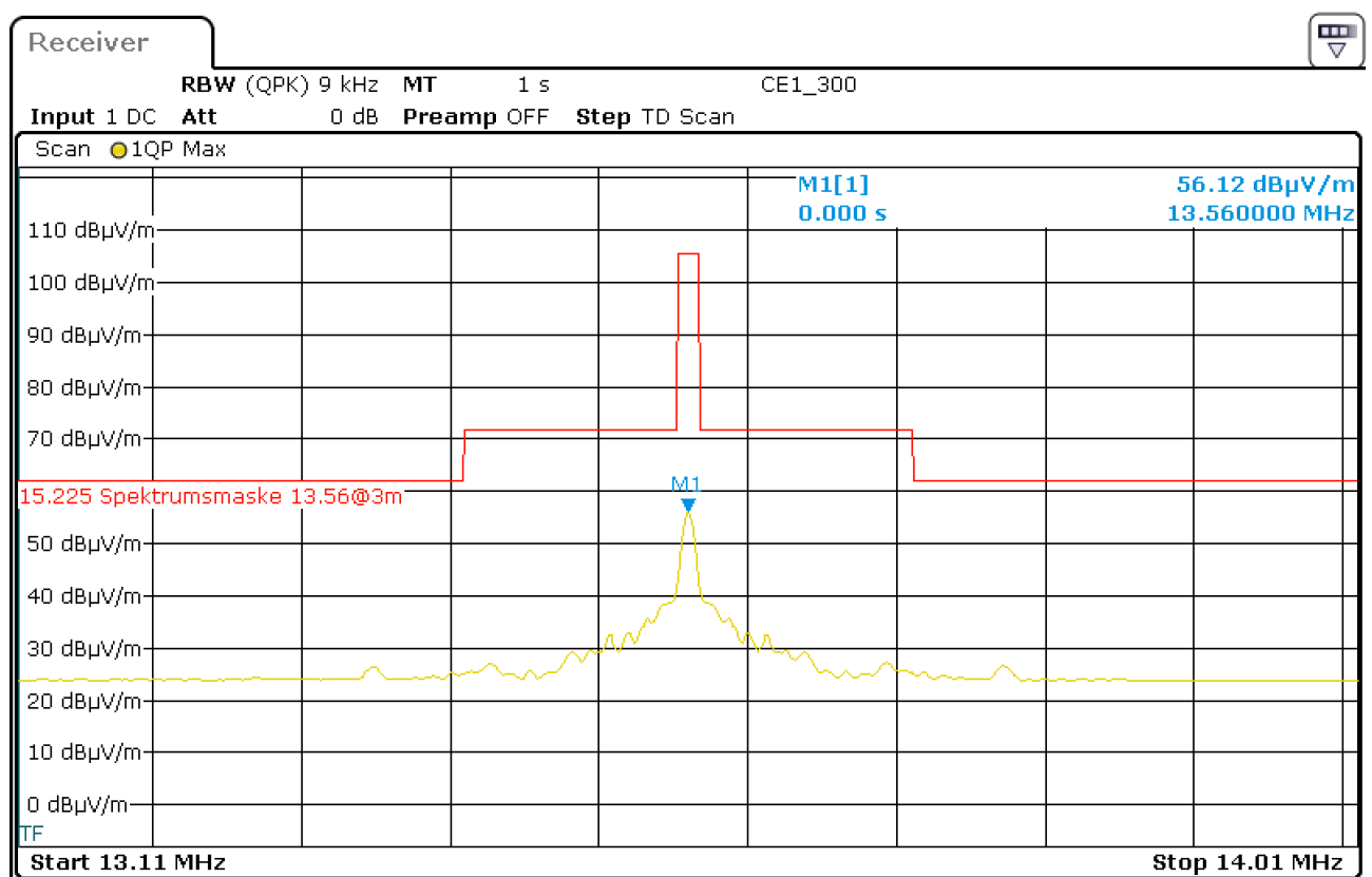
Figure 10: Chart of emission within the band 13.110 MHz to 14.010 MHz, EUT in position X, without tag, antenna in line at 3 m distance
