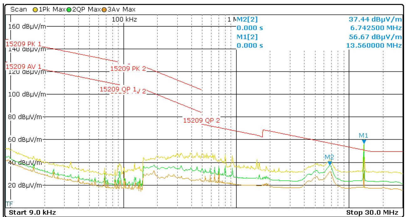
Figure 11: Chart of radiated emissions pre-measurement below 30 MHz, EUT position X, antenna polarization parallel, without tag
