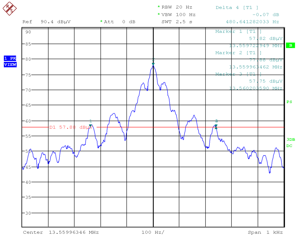
Figure 8: Chart of 20 dB bandwidth tests at normal conditions, without tag
