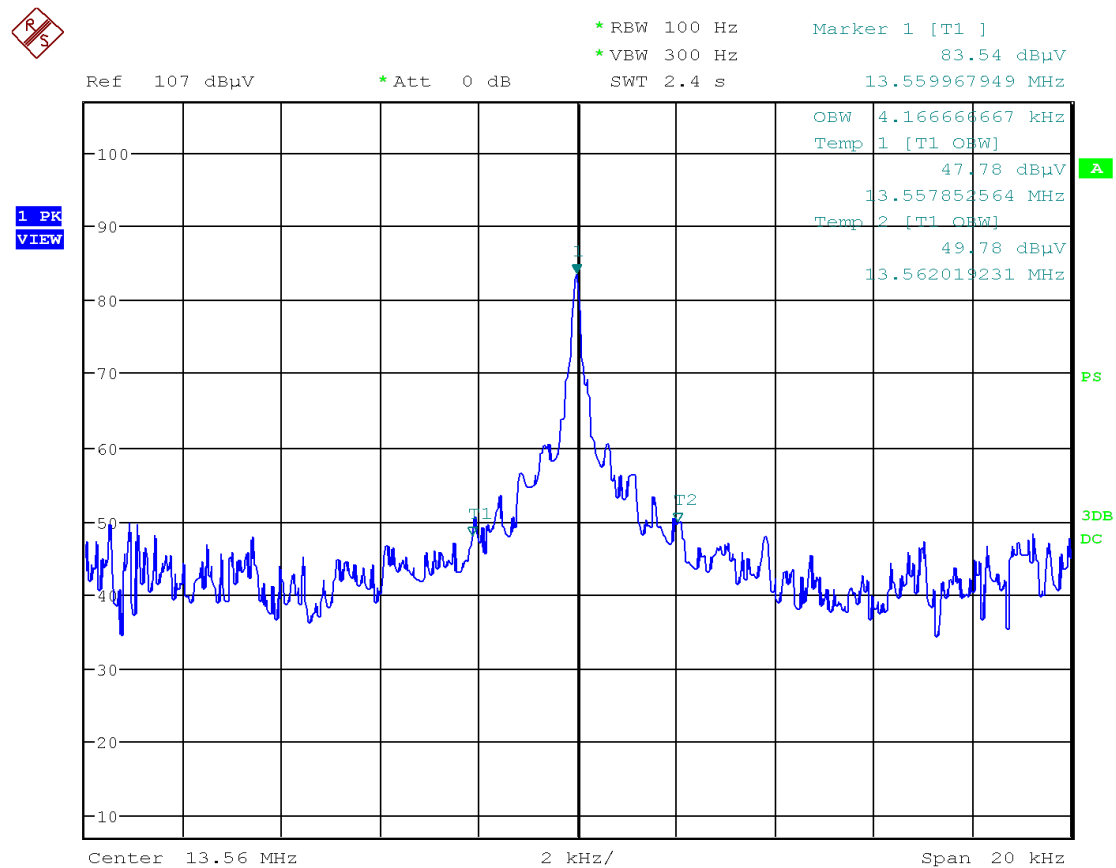
Figure 9: Chart of occupied bandwidth test, without tag
