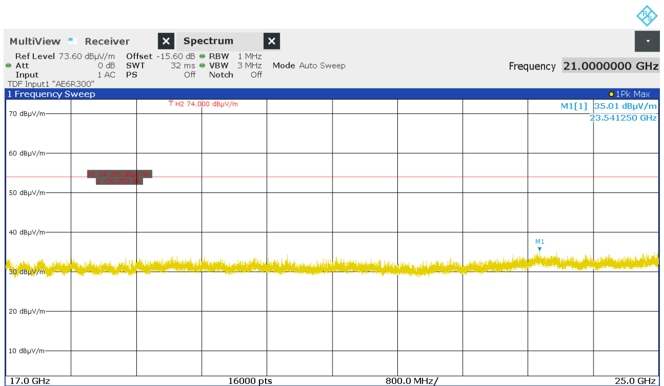
Figure 15: Chart of exploratory radiated emissions measurement from 17 GHz to 25 GHz on highest channel, EUT position Y, antenna polarization horizontal, without tag
