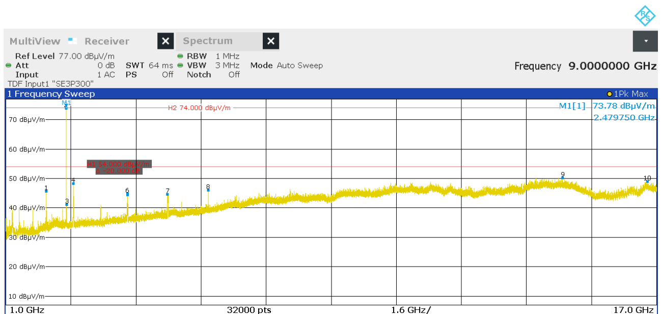
Figure 14: Chart of radiated emissions pre-measurement from 1 GHz to 17 GHz on highest channel, EUT position Z, antenna polarization vertical, with 13.56 MHz tag
