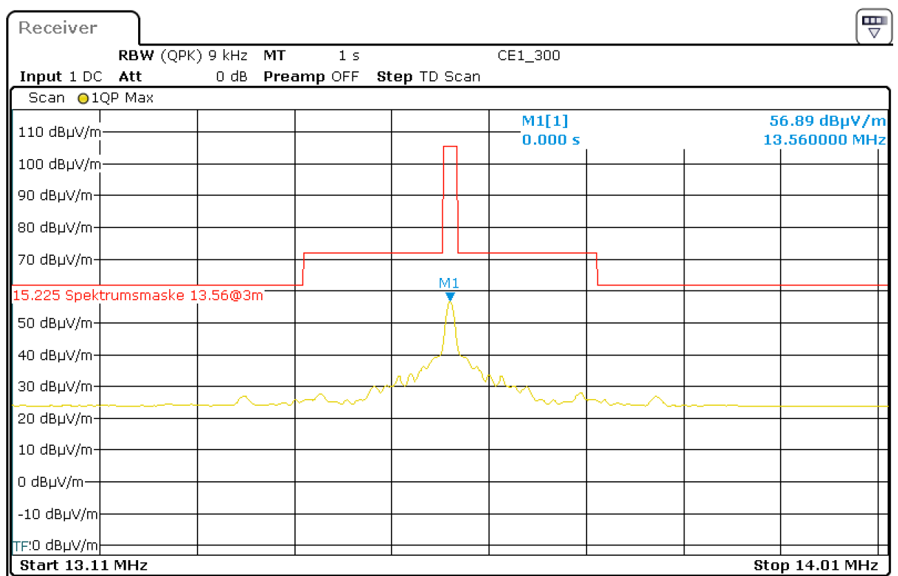
Figure 9: Chart of emission within the band 13.110 MHz to 14.010 MHz, EUT in position X, without tag, antenna parallel at 3 m distance
