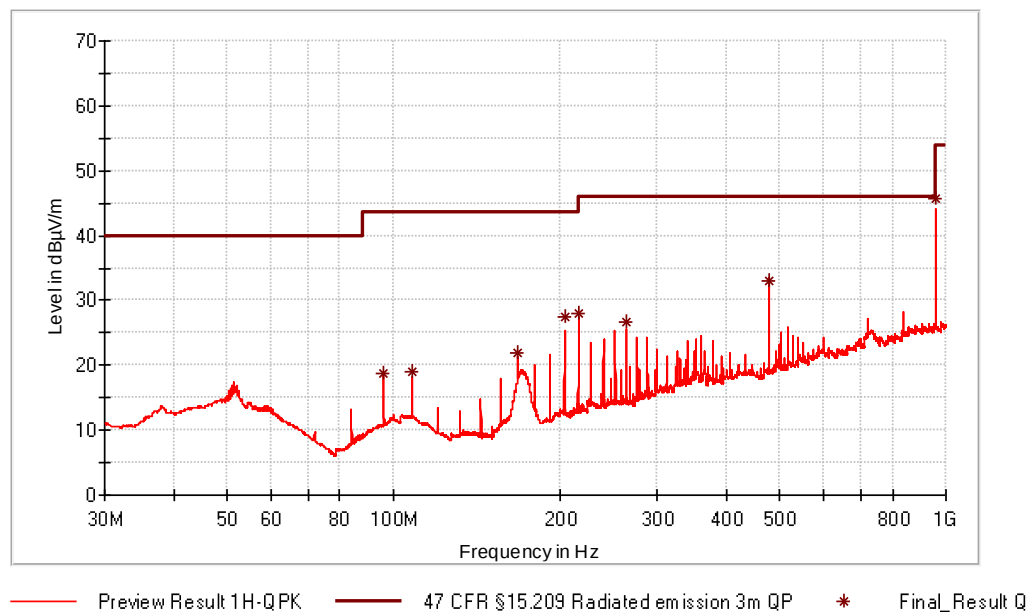
Figure 13: Chart of radiated emissions test from 30 MHz to 1 GHz, EUT position X, without tag, antenna horizontal
