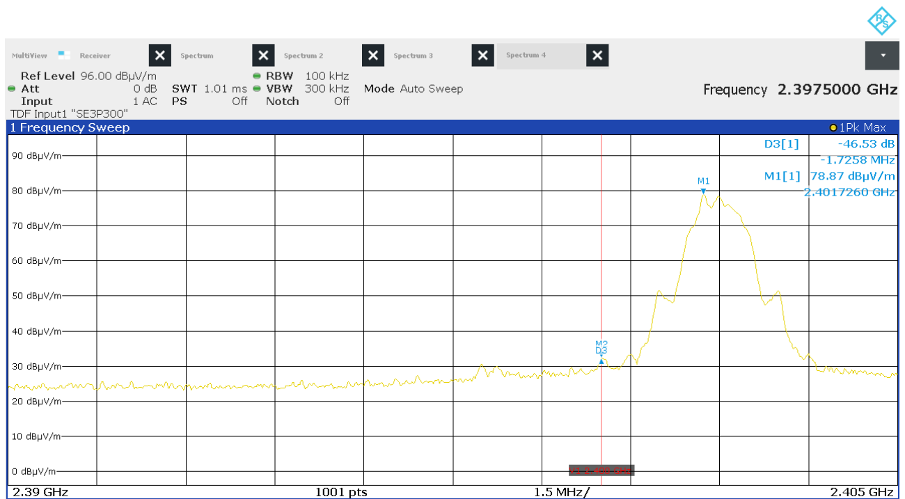
Figure 10: Chart of lower band edge measurement on lowest channel, EUT position X, antenna polarization horizontal
