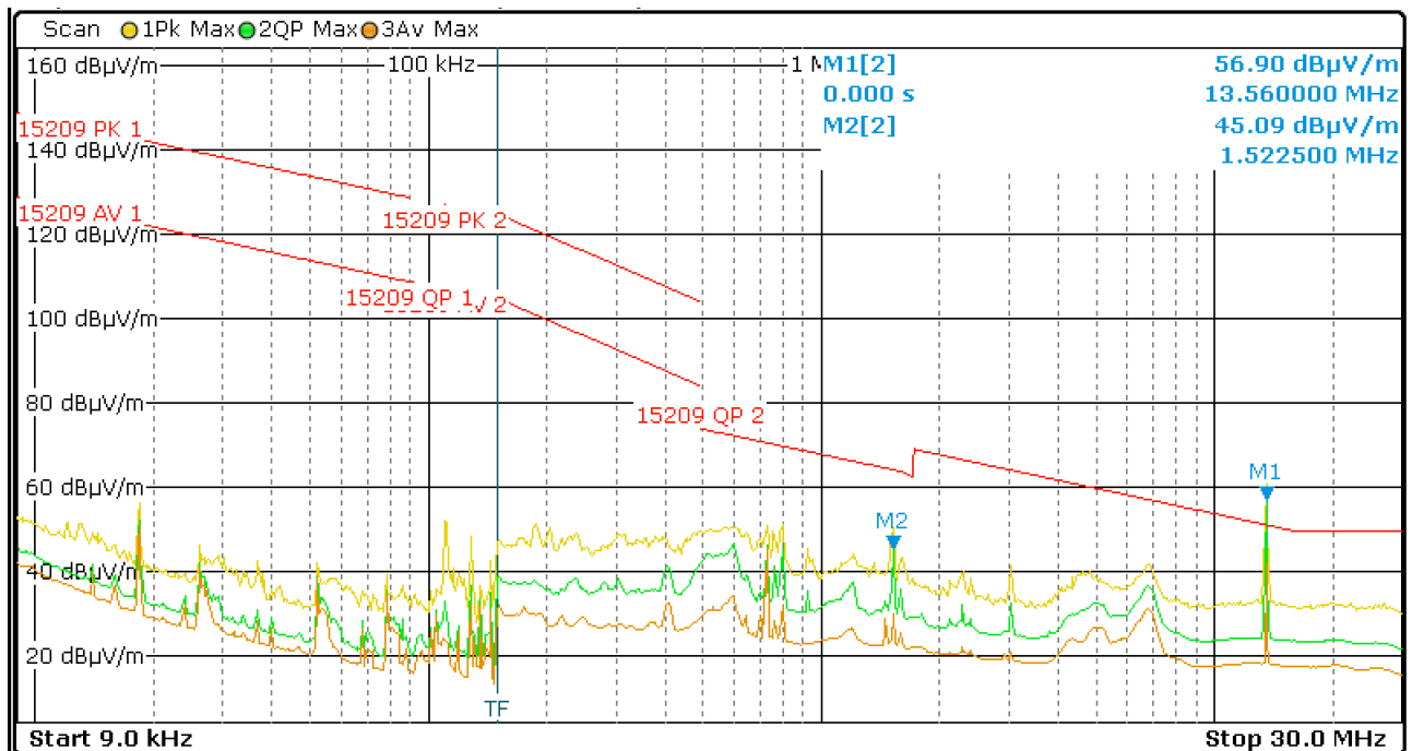
Figure 12: Chart of radiated emissions test below 30 MHz, EUT position X, with tag, antenna parallel
