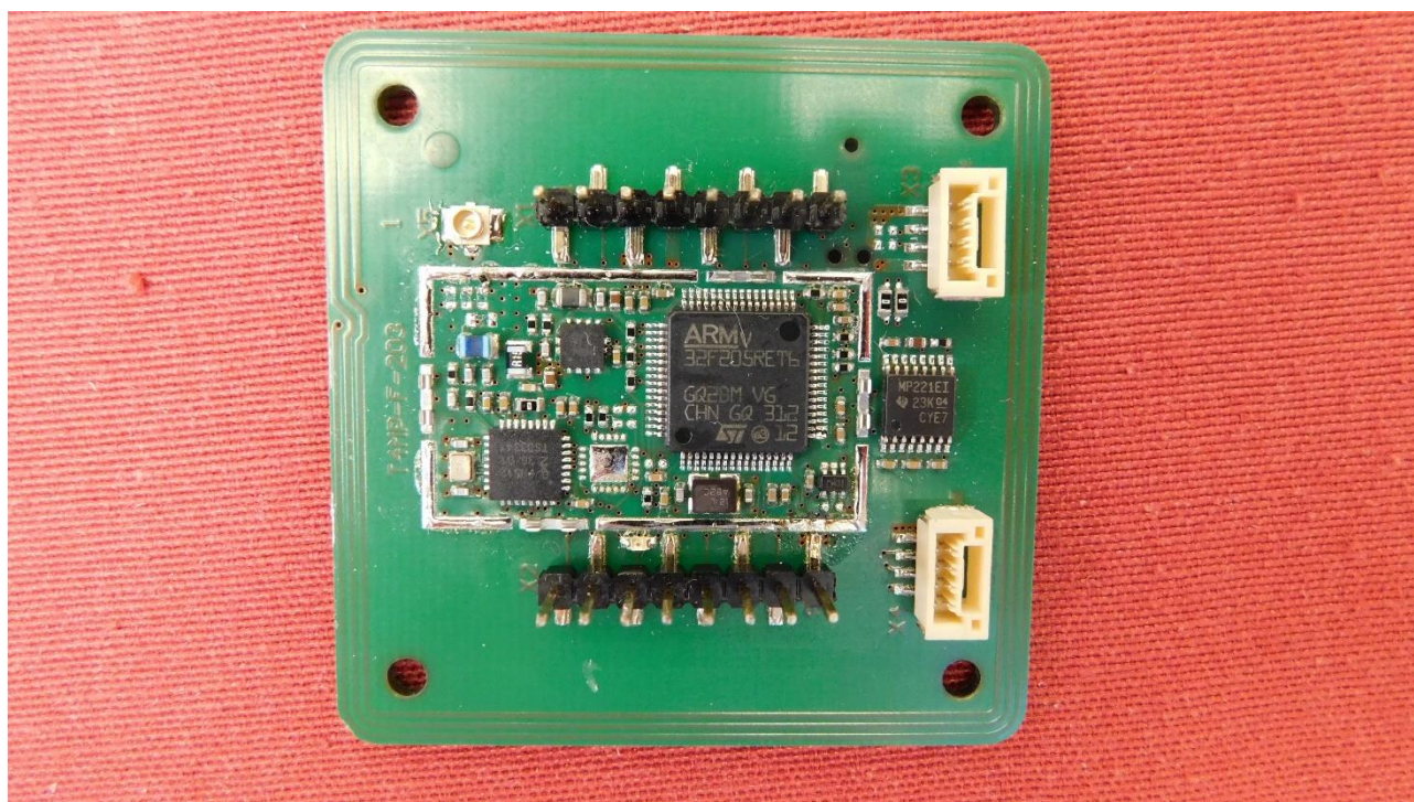
Picture 5: PCB – bottom side without shielding
