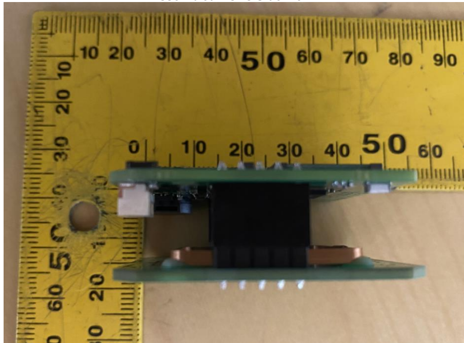
Assembled PCBs Side view 1
