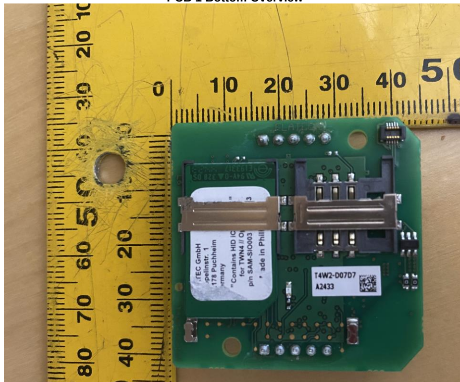
PCB 1 Bottom Overview
