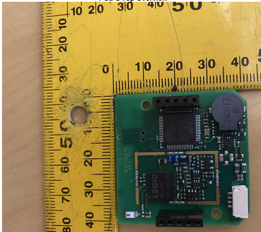
PCB 1 Top Overview
