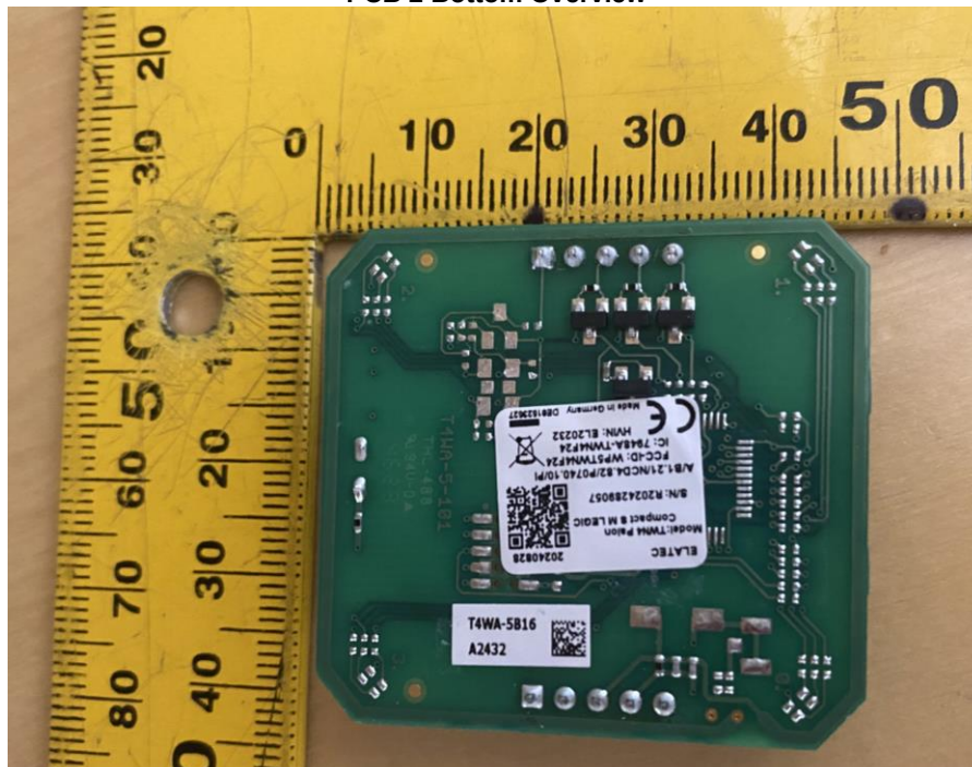
PCB 2 Bottom Overview
