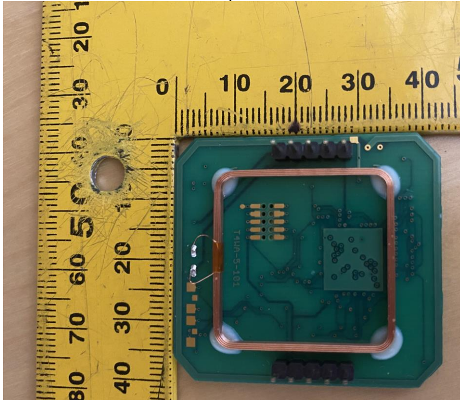
PCB 2 Top Overview
