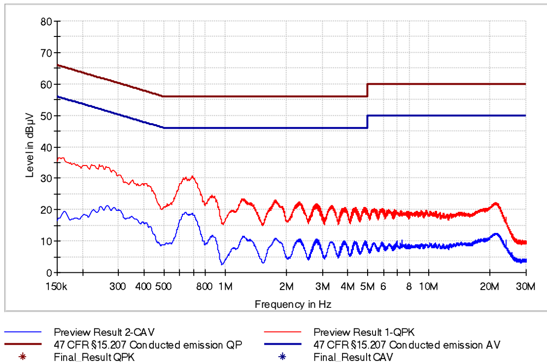
Figure 7: Chart of AC powerline conducted emissions on L1, RS232
