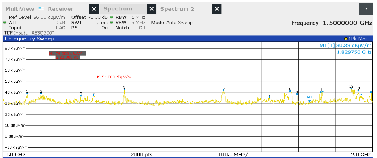
Figure 16: Chart of radiated emissions pre-measurement from 1 GHz to 2 GHz, EUT position Y, with tag, antenna polarization vertical, RS232
