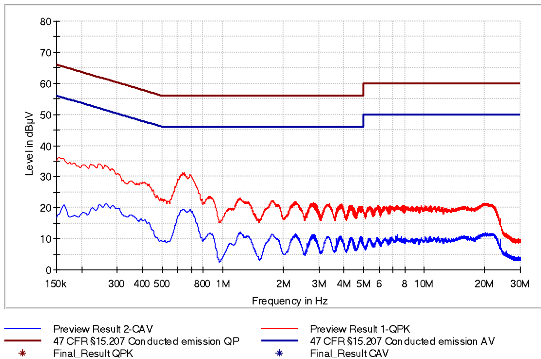
Figure 8: Chart of AC powerline conducted emissions on N, RS232
