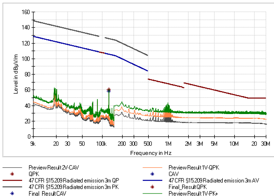
Figure 11: Chart of radiated emissions test below 30 MHz, EUT position Z, without tag, antenna parallel, USB
