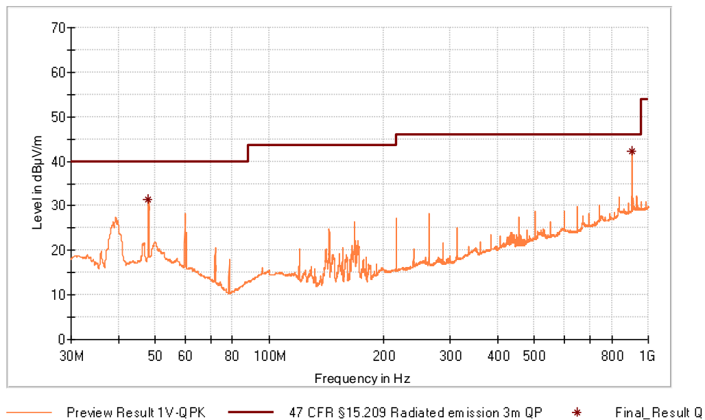
Figure 14: Chart of radiated emissions test from 30 MHz to 1 GHz, EUT position Y, without tag, antenna vertical, RS232
