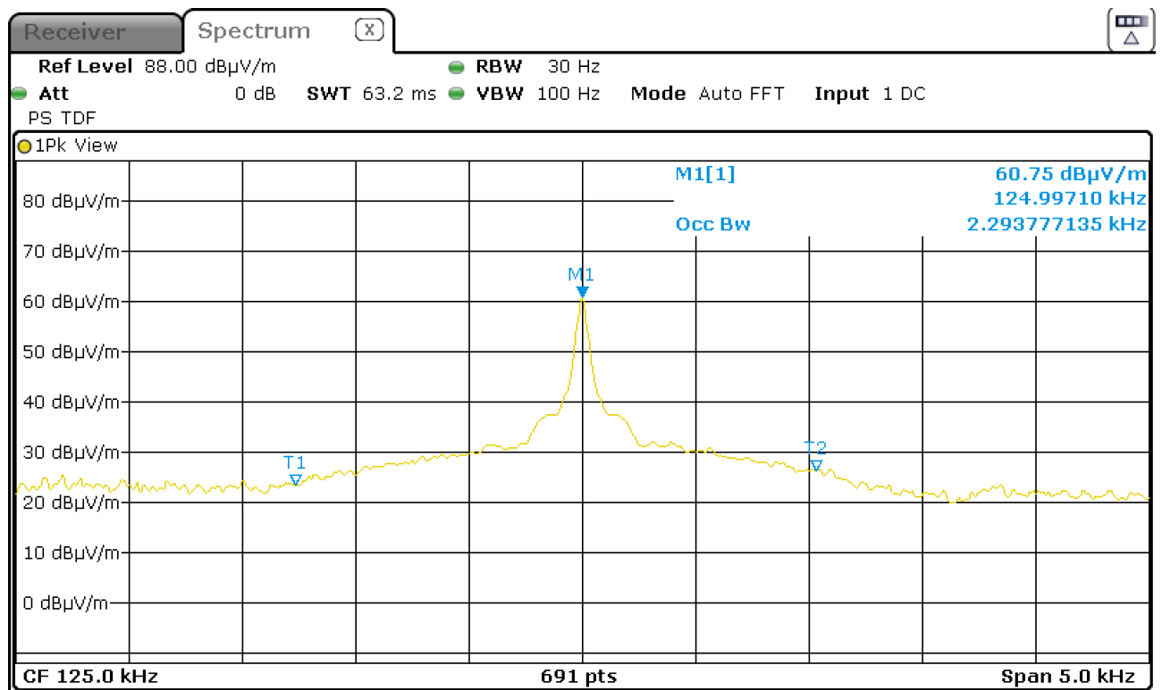
Figure 9: Chart of occupied bandwidth test, without tag, USB
