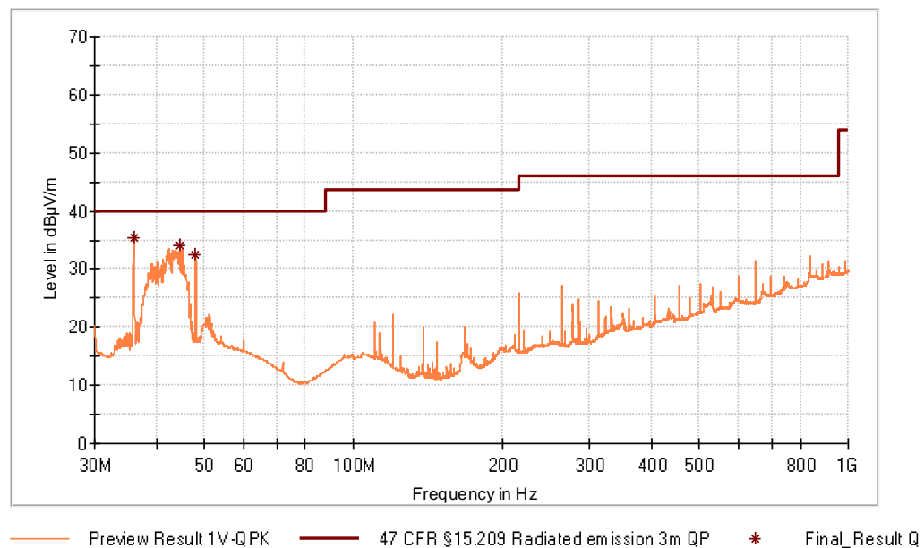
Figure 13: Chart of radiated emissions test from 30 MHz to 1 GHz, EUT position X, with tag, antenna vertical, USB
