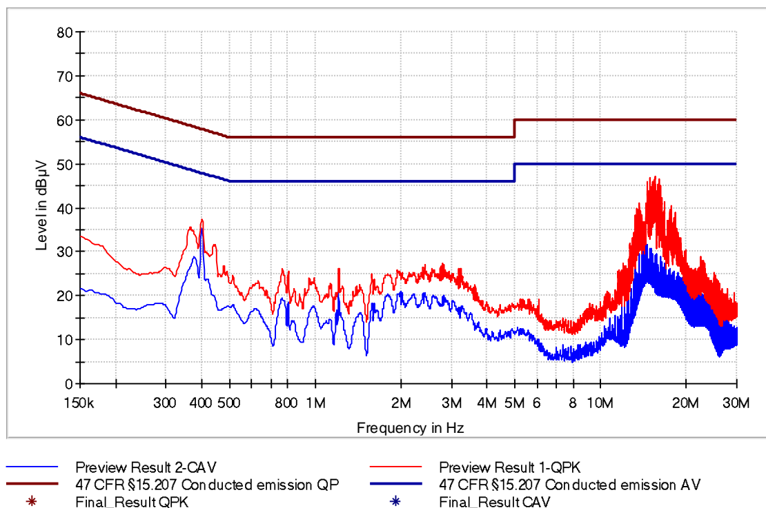
Figure 6: Chart of AC powerline conducted emissions on N, USB
