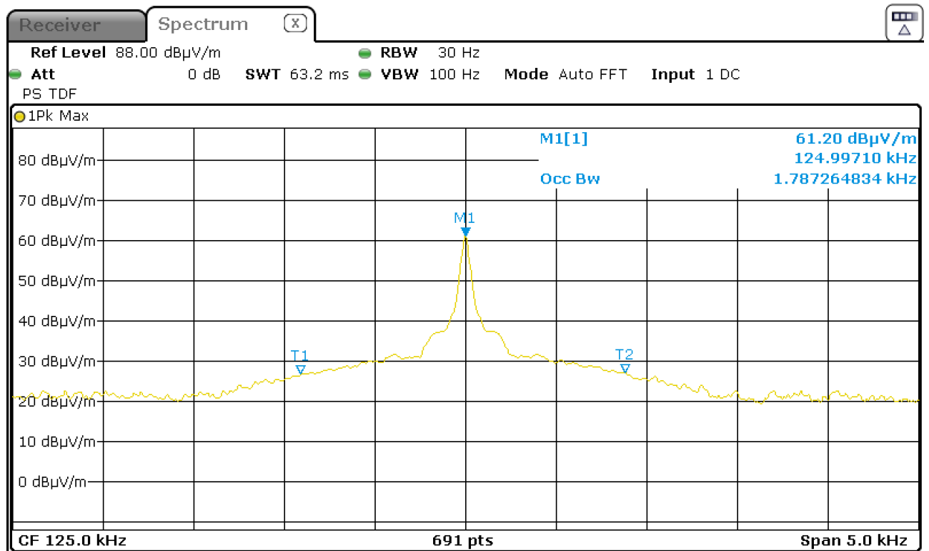
Figure 10: Chart of occupied bandwidth test, without tag, RS232
