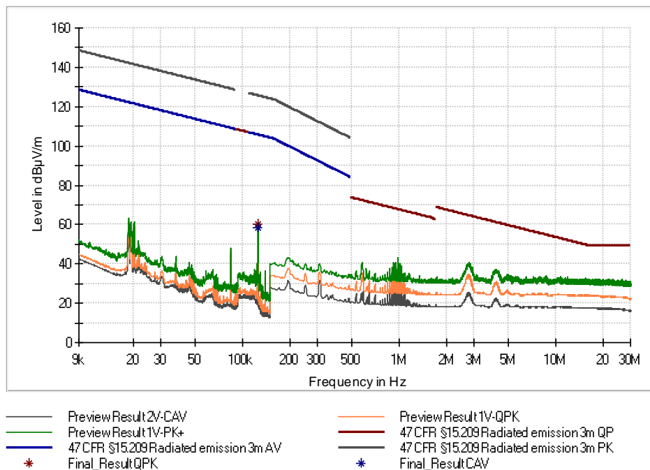
Figure 12: Chart of radiated emissions test below 30 MHz, EUT position Y, without tag, antenna in line, RS232
