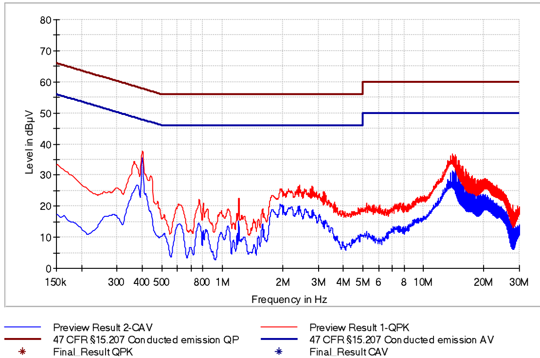
Figure 5: Chart of AC powerline conducted emissions on L1, USB
