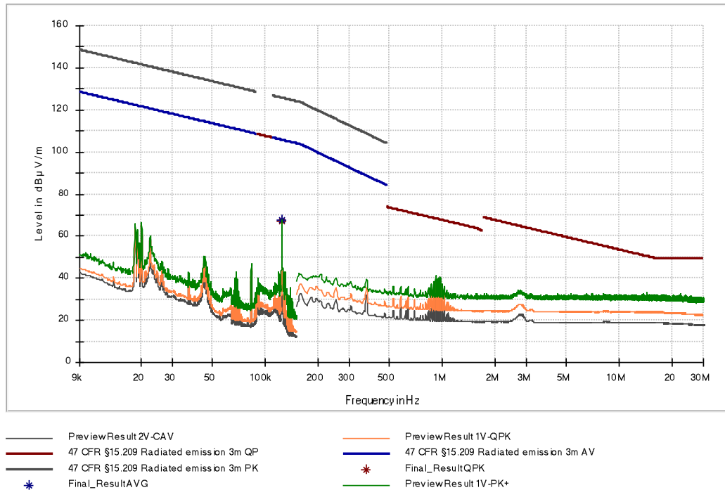
Figure 12: Chart of emissions test below 30 MHz, EUT position Y, without tag, antenna parallel at 3 m
