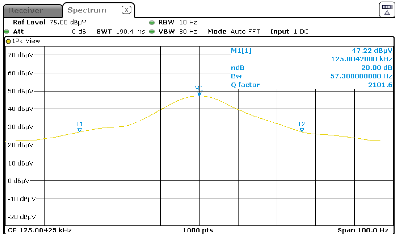
Figure 9: Chart of 20 dB bandwidth test, with tag
