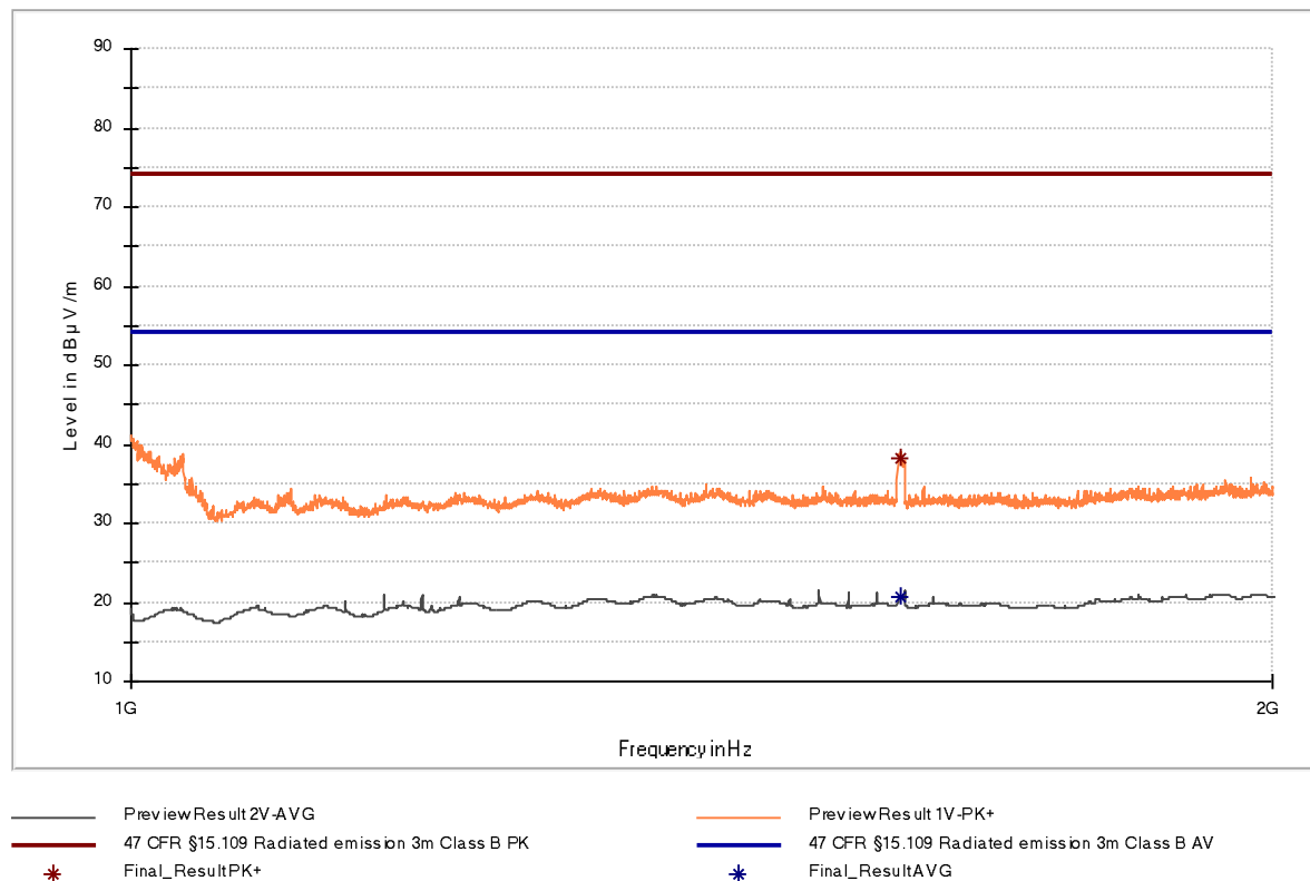
Figure 14: Chart of emissions test from 1 GHz to 2 GHz, EUT position Y, without tag, antenna vertical, at 3 m
