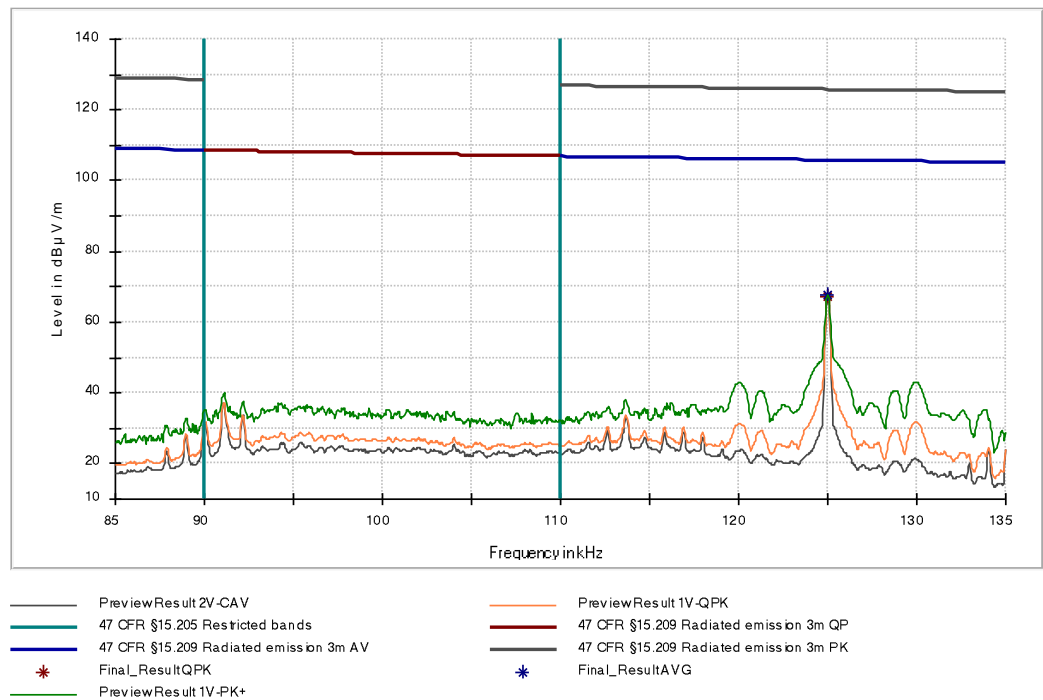
Figure 11: Chart of restricted band of operation, EUT position Y, without tag, antenna parallel at 3 m
