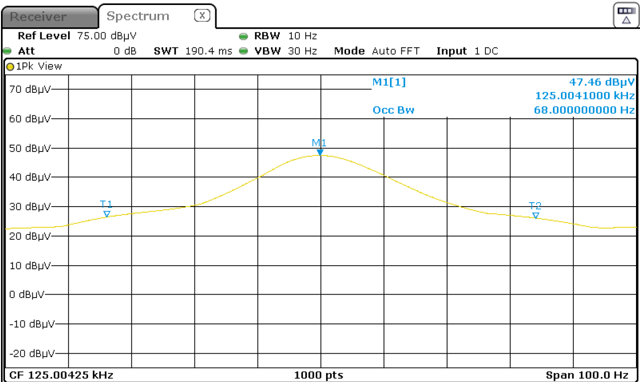
Figure 10: Chart of occupied bandwidth test, with tag
