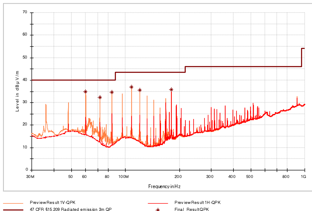
Figure 13: Chart of emissions test from 30 MHz to 1 GHz, EUT position X, with tag, at 3 m
