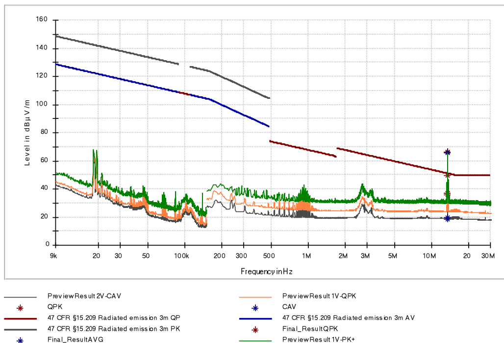
Figure 15: Chart of emissions test below 30 MHz without tag in position 2, antenna in line at 3 m, USB active
