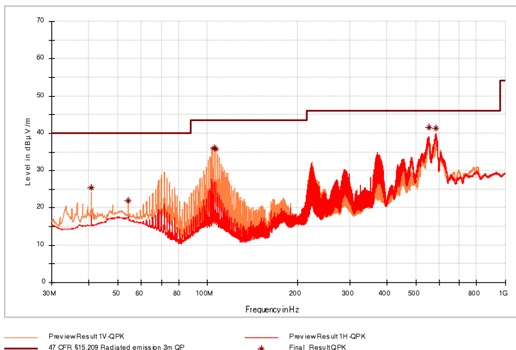
Figure 17: Chart of emissions test from 30 MHz to 1 GHz with tag in position 2 at 3 m, RS-232 active
