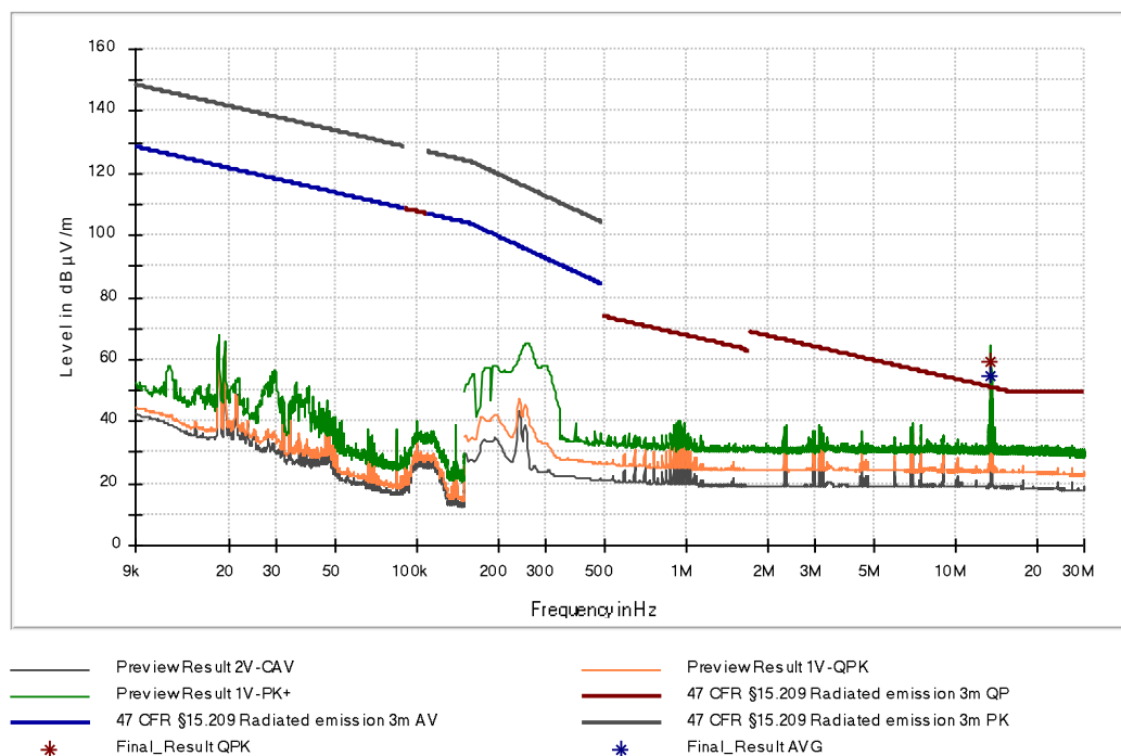
Figure 13: Chart of emissions test below 30 MHz without tag in position 1, antenna in line at 3 m, RS-485 active
