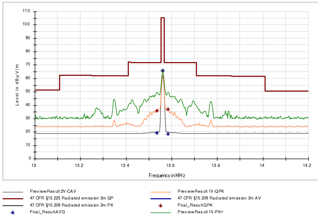
Figure 12: Chart of emission within the band 13.110 MHz to 14.010 MHz, without tag, position 2, antenna in line at 3m distance
