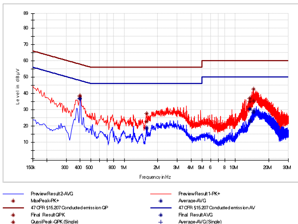
Figure 9: Chart of AC powerline conducted emissions on N – with termination
