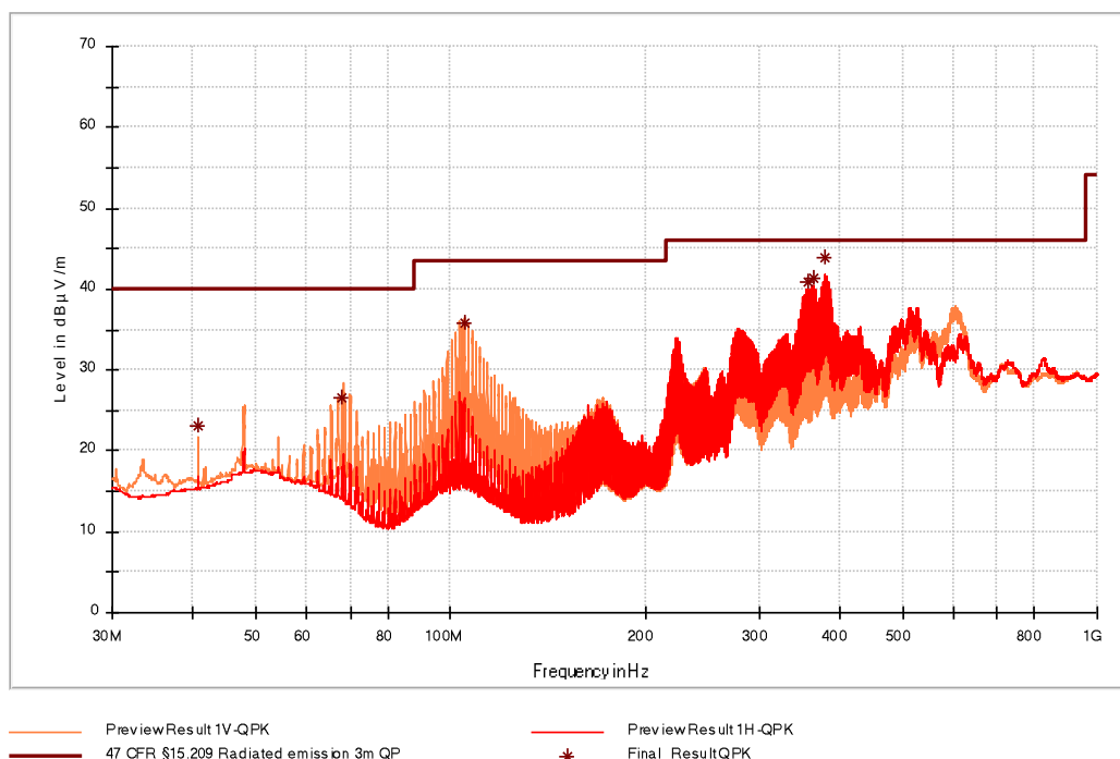
Figure 16: Chart of emissions test from 30 MHz to 1 GHz with tag in position 2 at 3 m, RS-485 active
