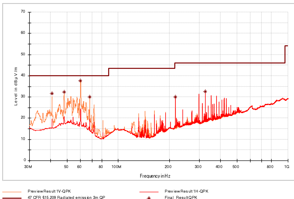
Figure 18: Chart of emissions test from 30 MHz to 1 GHz with tag in position 2 at 3 m, USB active
