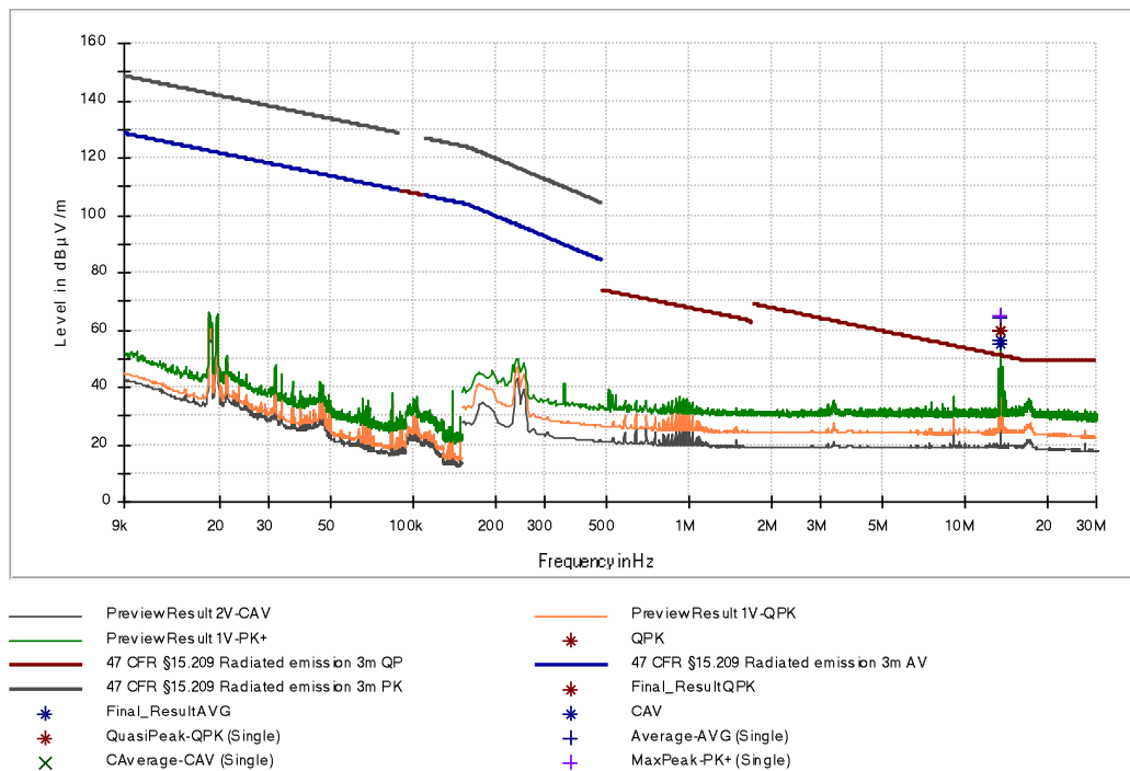
Figure 14: Chart of emissions test below 30 MHz without tag in position 1, antenna in line at 3 m, RS-232 active
