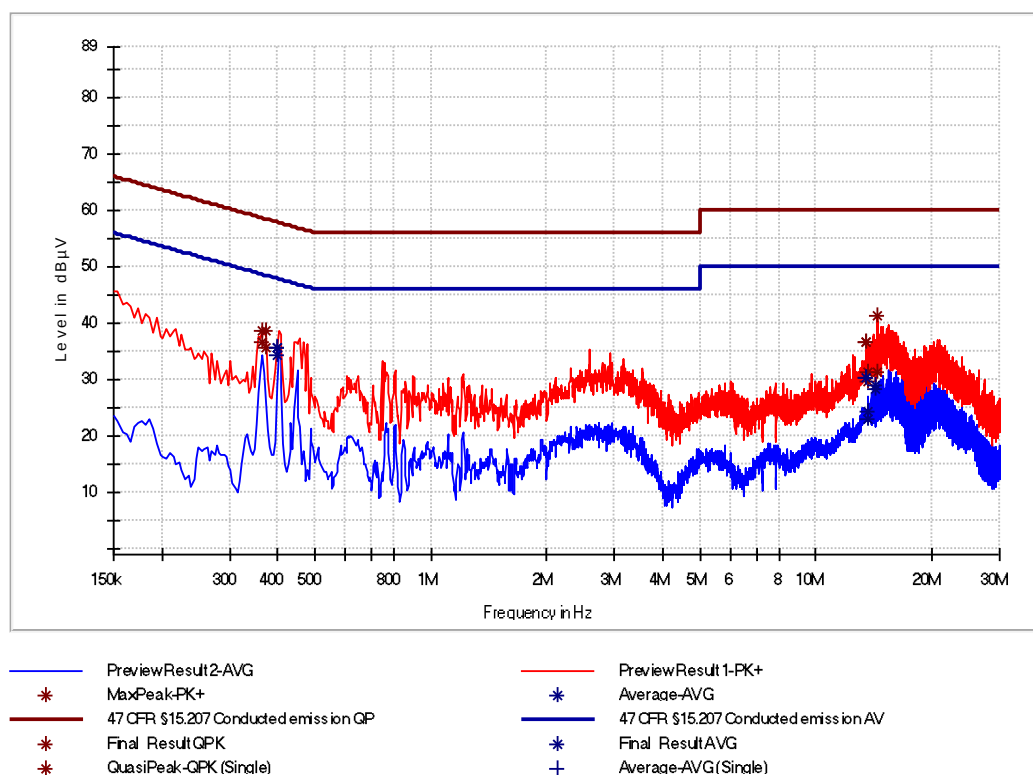
Figure 8: Chart of AC powerline conducted emissions on L1 – with termination
