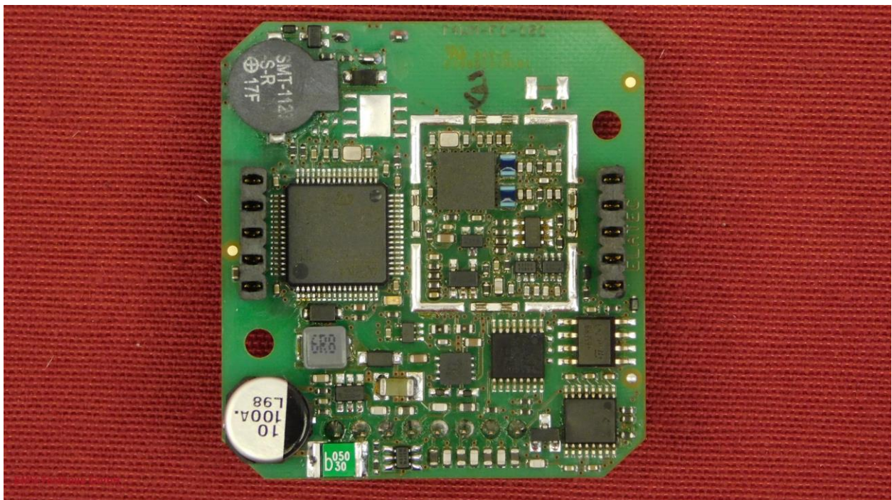
Picture 4: Controller board – top view – without shielding
