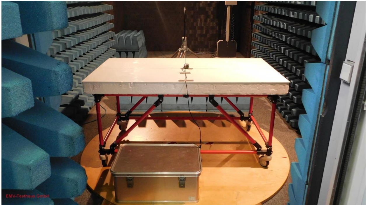
Picture 1: EUT test setup radiated emission test 9 kHz – 30 MHz (front view)
