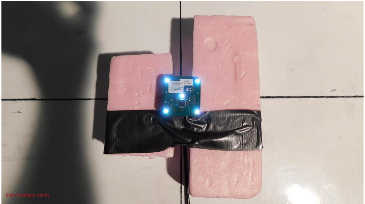
Picture 9: EUT Position 3
