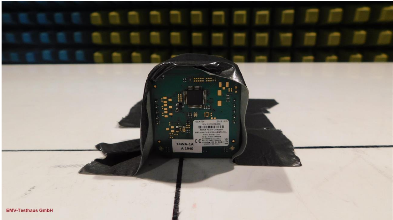
Picture 7: EUT Position 1
