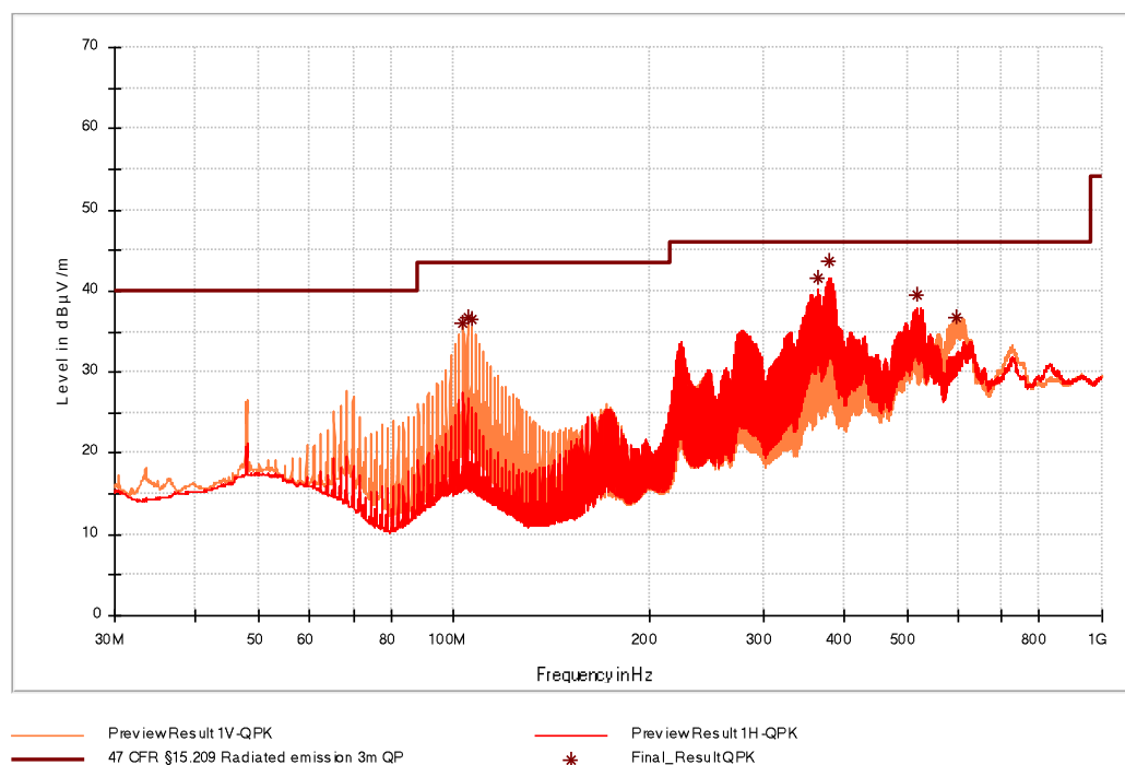
Figure 15: Chart of emissions test from 30 MHz to 1 GHz with tag in position 2, RS-485 active
