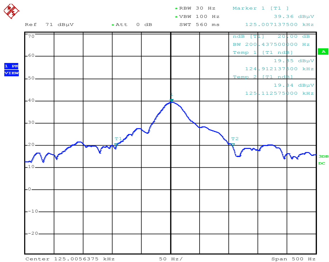
Figure 9: Chart of 20 dB bandwidth on 125 kHz without tag
