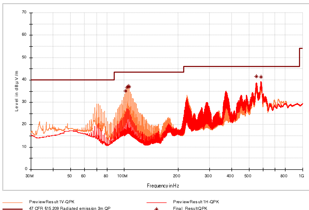
Figure 16: Chart of emissions test from 30 MHz to 1 GHz with tag in position 2, RS-232 active
