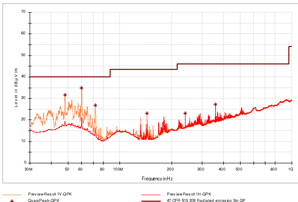
Figure 17: Chart of emissions test from 30 MHz to 1 GHz with tag in position 2, USB active
