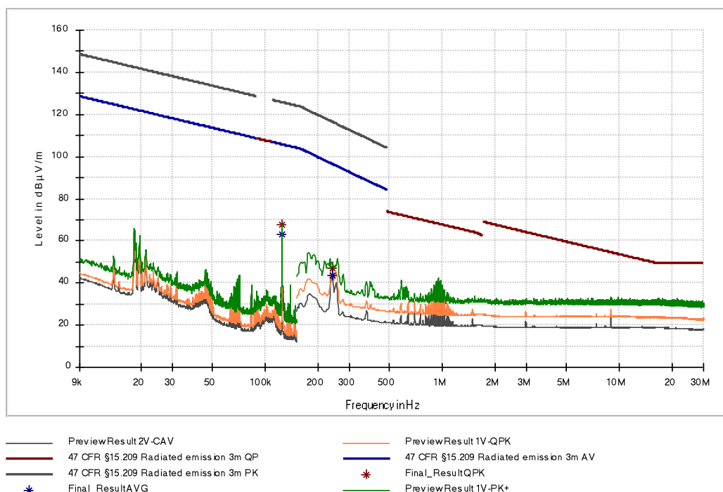
Figure 12: Chart of emissions test below 30 MHz without tag in position 1, RS-485 active
