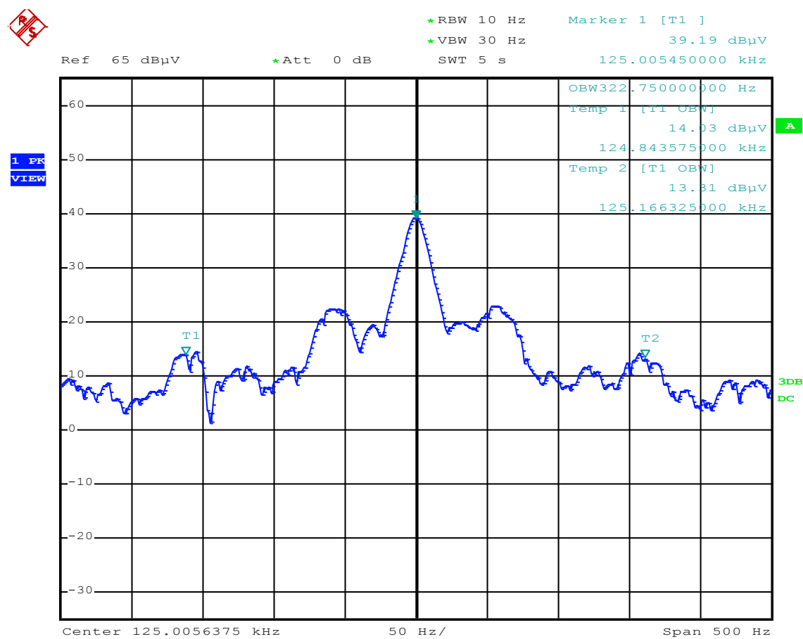
Figure 10: Chart of occupied bandwidth test
