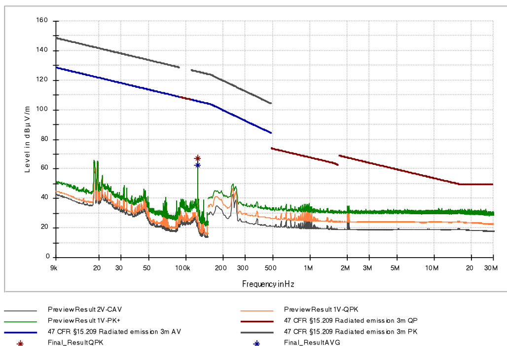
Figure 13: Chart of emissions test below 30 MHz without tag in position 1, RS-232 active
