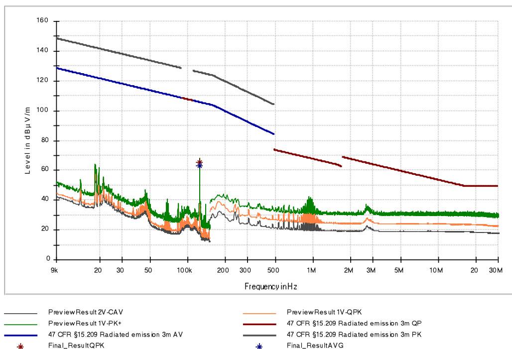
Figure 14: Chart of emissions test below 30 MHz without tag in position 2, USB active
