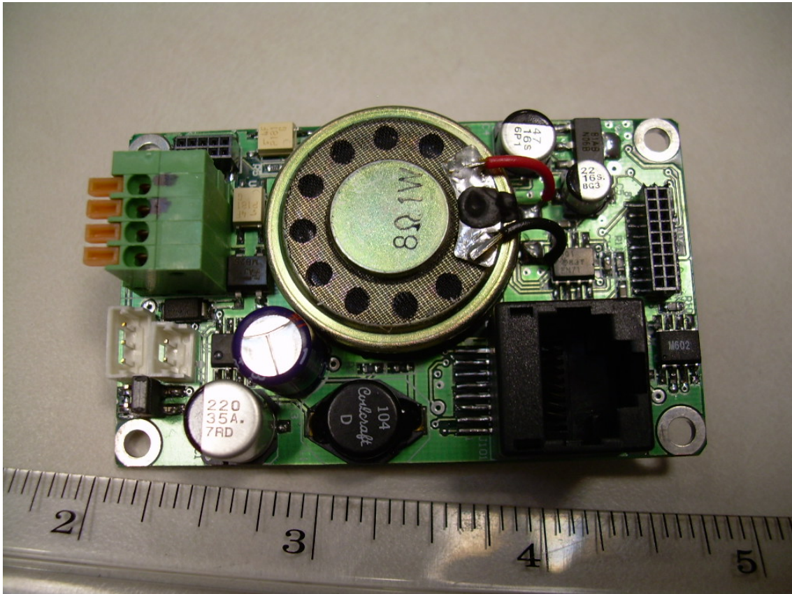
Back View of the Interface PCB
