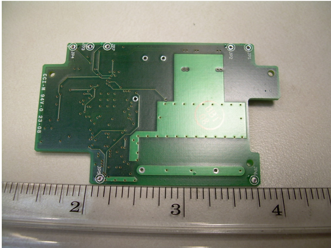
Back View of the RF PCB
