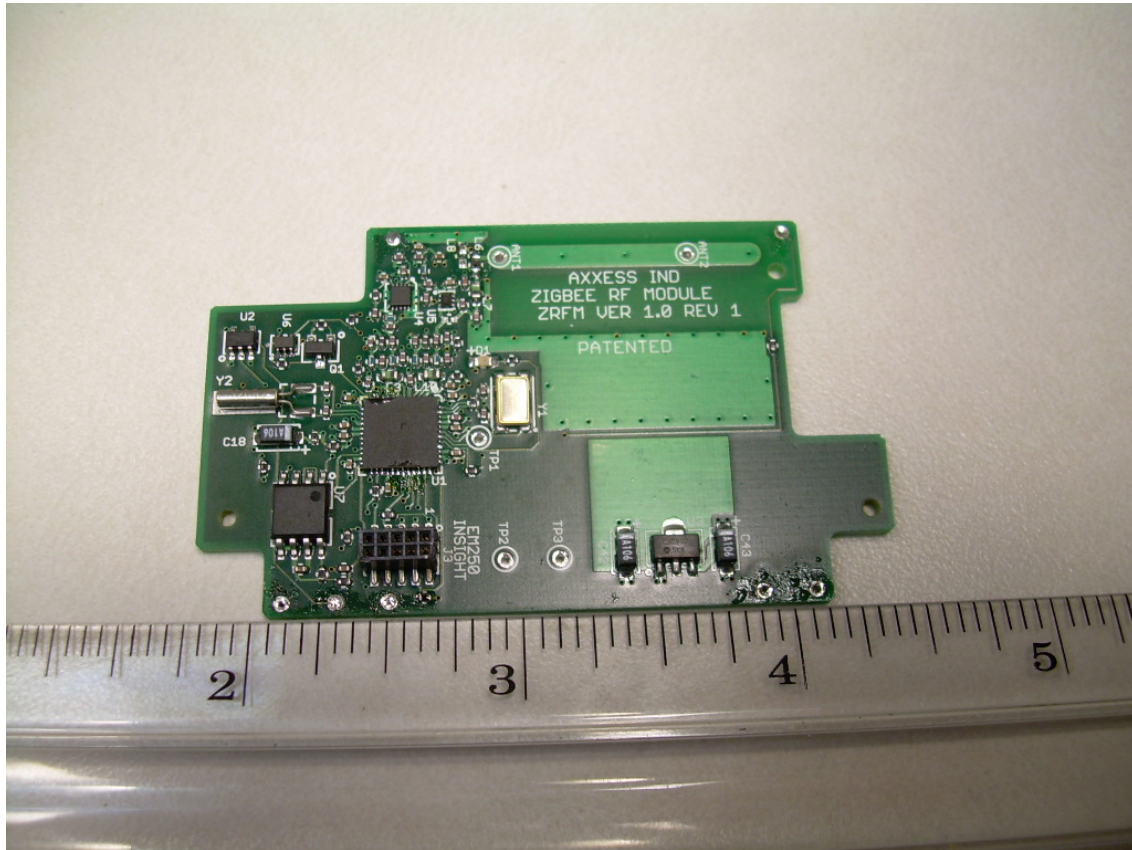
Front View of the RF PCB
