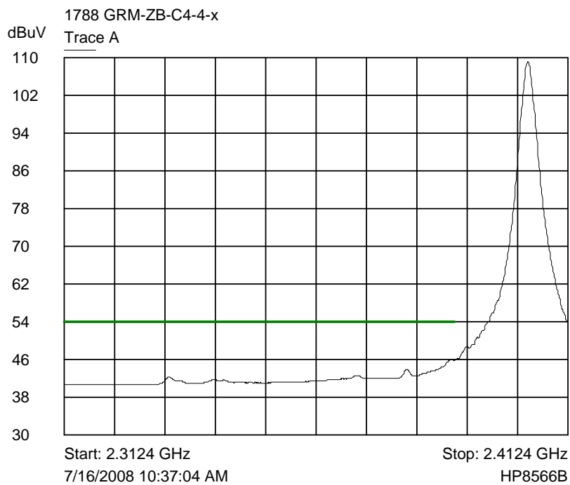
Trace A Radiated lower band edge - average detection vs average limit - corrected plot
