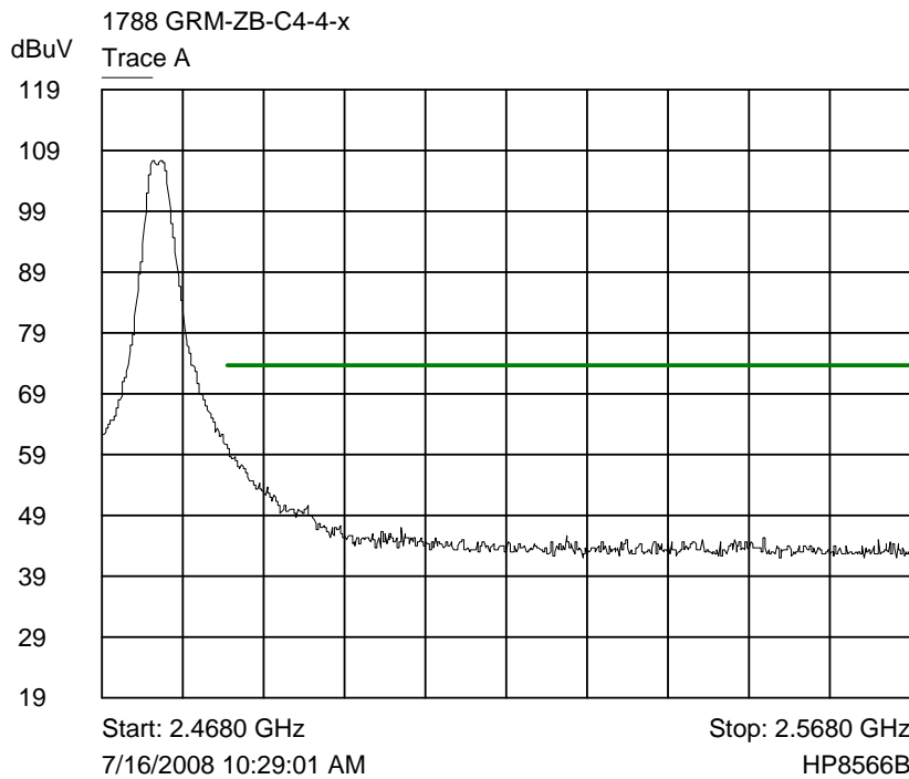
Trace A Radiated upper band edge - peak detection vs peak limit - corrected plot
