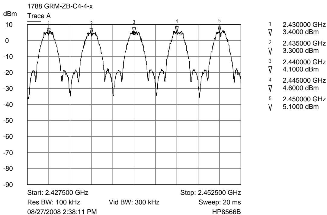
Trace A Middle 5 channels
