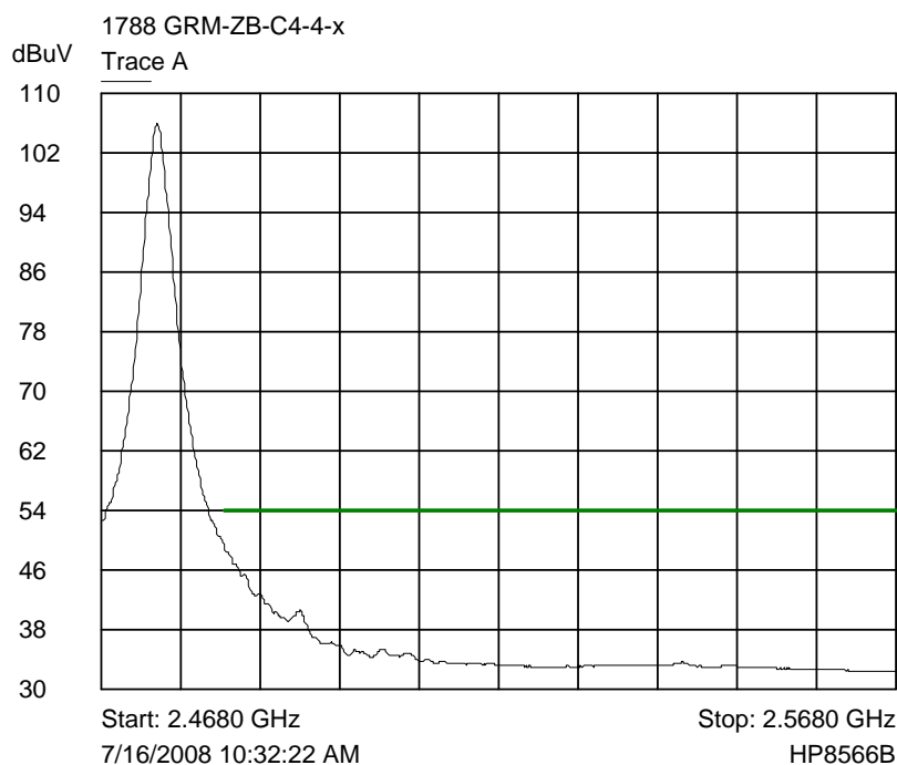
Trace A Radiated upper band edge - average detection vs average limit - corrected plot
