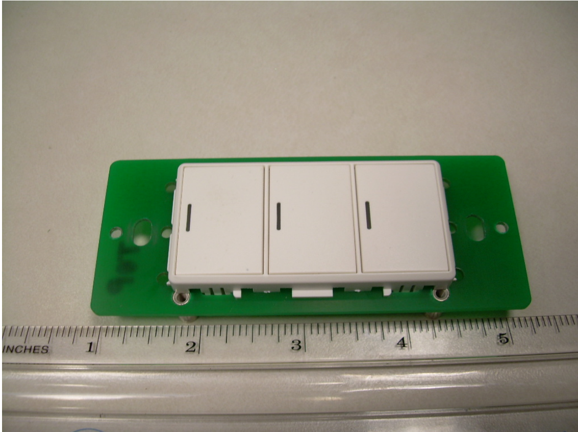
Front View of the Button PCB
